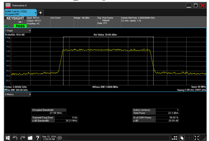
n77_2_30MHz_30kHz_3565MHz_DFT-s-OFDM 16 QAM_RB75@0 27.748MHz
