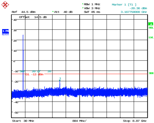
5MHz_Low_QPSK_1@0(30MHz~8.87GHz)
