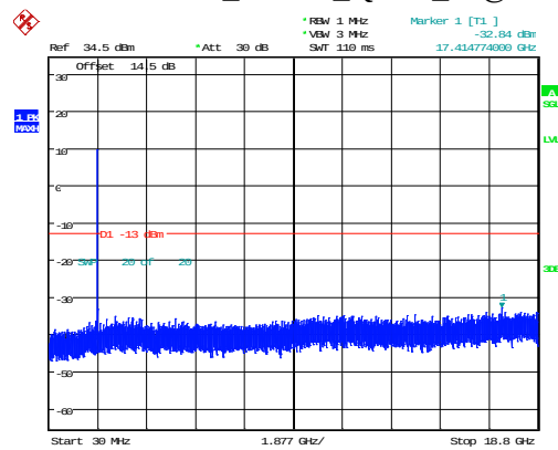
15MHz_Middle_QPSK_75@0
