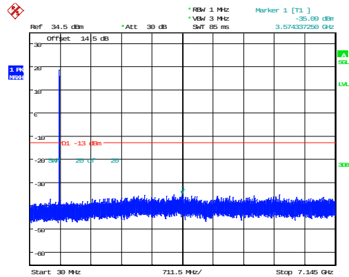
3MHz_High_QPSK_1@0
