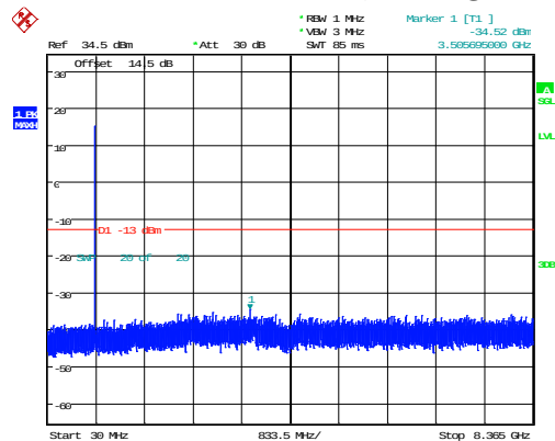
3MHz_Middle_QPSK_1@0
