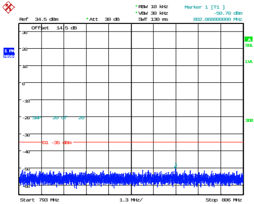
5MHz_Low_QPSK_1@0(793MHz~806MHz)
