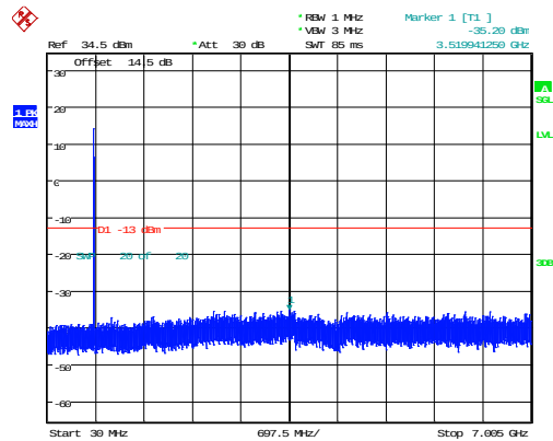
3MHz_Low_QPSK_1@0
