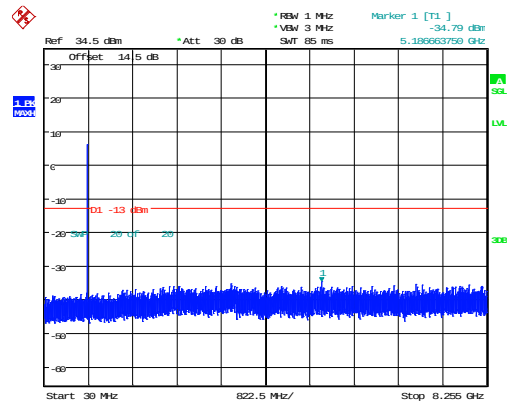
3MHz_Low_QPSK_15@0
