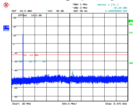
3MHz_High_QPSK_15@0
