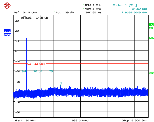
3MHz_Middle_QPSK_15@0
