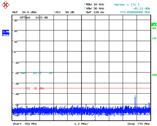
5MHz_Low_QPSK_1@0(763MHz~775MHz)
