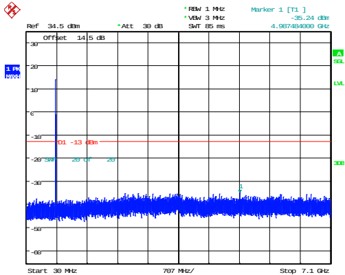
5MHz_Middle_QPSK_1@0
