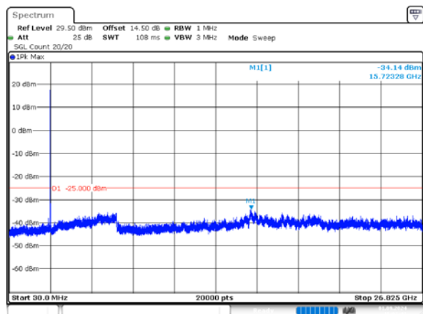
15MHz_High_QPSK_1@0
