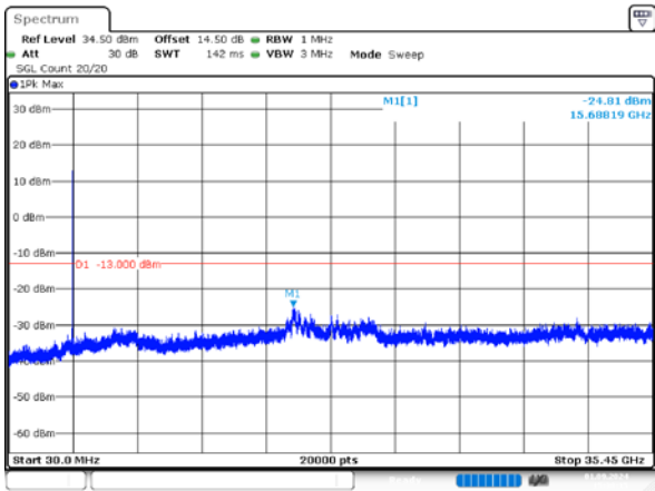
1_10MHz_High_QPSK_1@0
