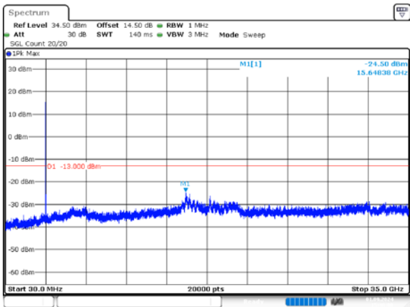
1_15MHz_Middle_QPSK_1@0
