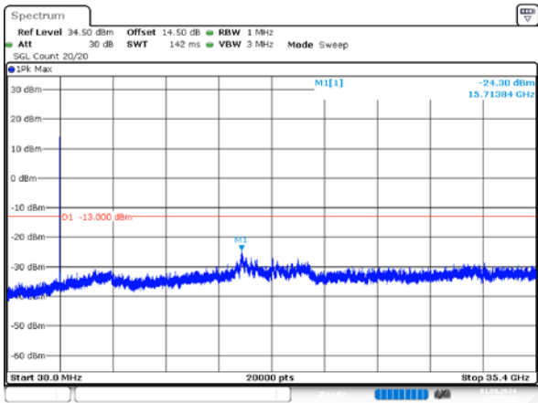
1_20MHz_High_QPSK_1@0
