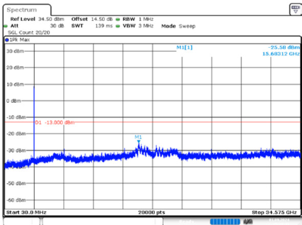
1_15MHz_Low_QPSK_75@0
