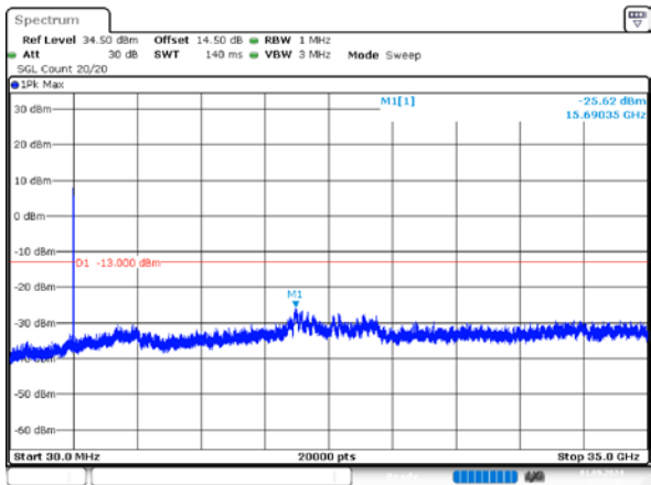
1_20MHz_Middle_QPSK_100@0
