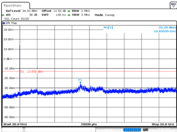
1_10MHz_Middle_QPSK_1@0
