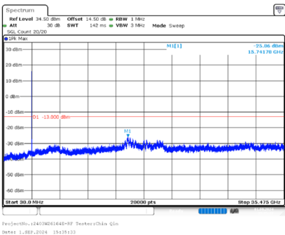
1_5MHz_High_QPSK_1@0
