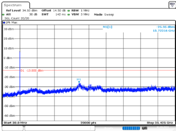
1_15MHz_High_QPSK_75@0
