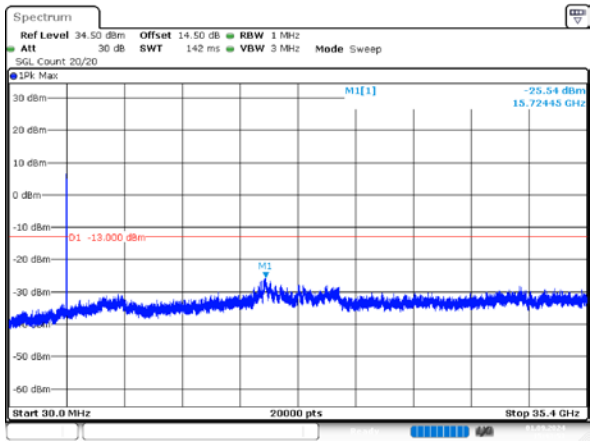
1_20MHz_High_QPSK_100@0
