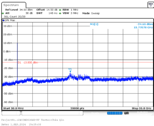
1_5MHz_High_QPSK_25@0
