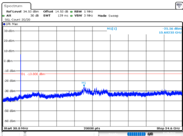
1_20MHz_Low_QPSK_100@0
