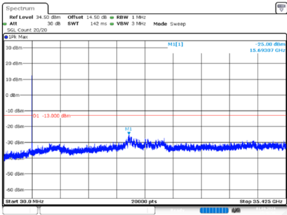
1_15MHz_High_QPSK_1@0
