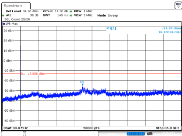
1_20MHz_Middle_QPSK_1@0
