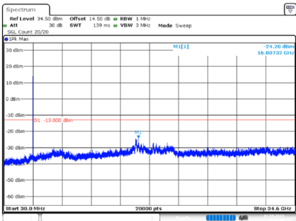
1_20MHz_Low_QPSK_1@0
