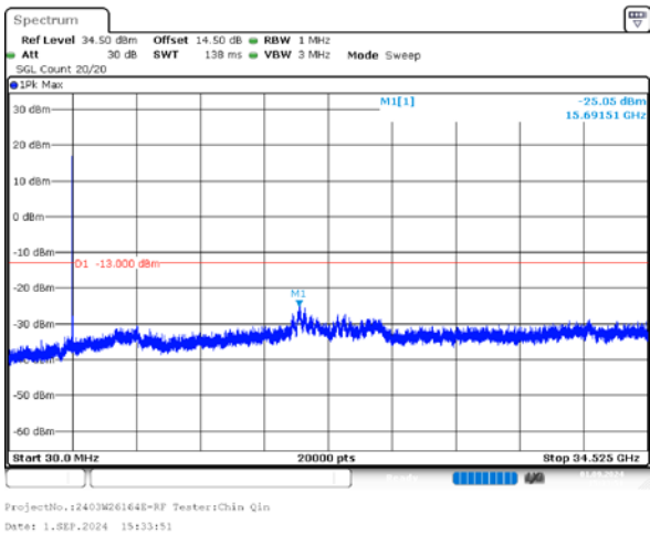
1_5MHz_Middle_QPSK_1@0
