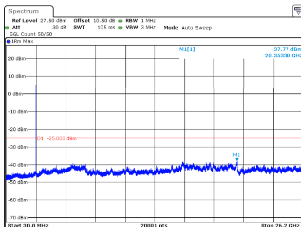
n38_15MHz_30kHz_2612.5MHz_DFT-s-OFDM QPSK_RB36@0 -37.77dBm
