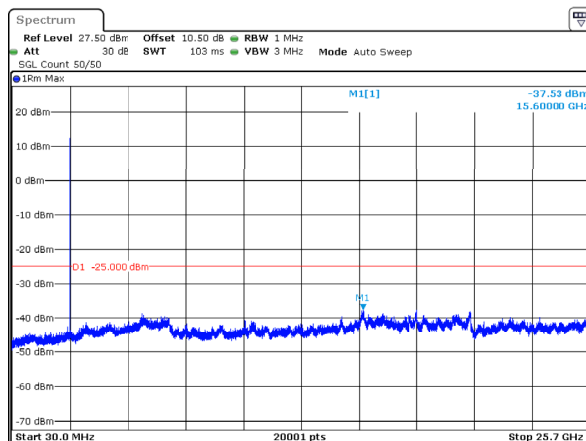
n7_5MHz_15kHz_2567.5MHz_DFT-s-OFDM QPSK_RB1@24 -37.53dBm
