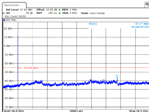
n38_10MHz_30kHz_2615MHz_DFT-s-OFDM QPSK_RB1@23 -37.77dBm
