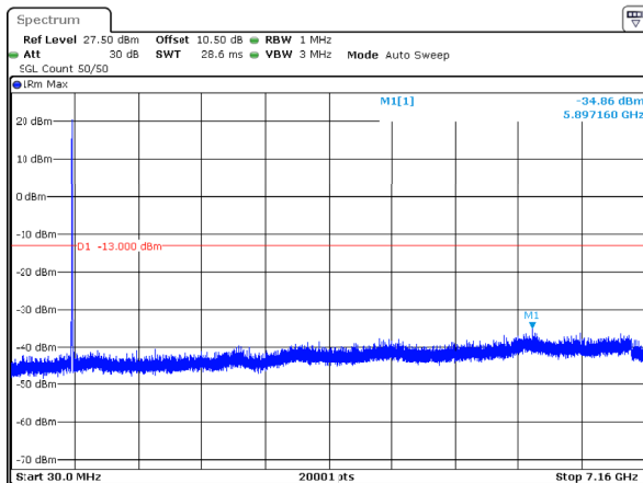
n12_5MHz_15kHz_713.5MHz_DFT-s-OFDM QPSK_RB25@0 -34.86dBm
