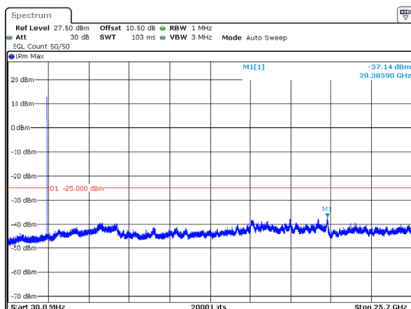
n7_10MHz_15kHz_2505MHz_DFT-s-OFDM QPSK_RB1@51 -37.14dBm
