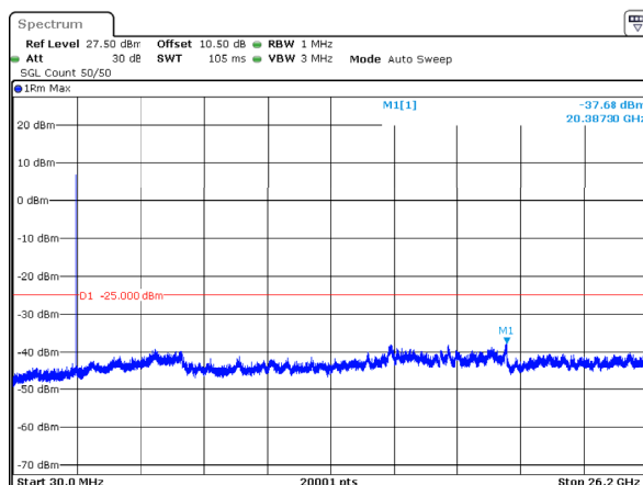
n38_15MHz_30kHz_2577.5MHz_DFT-s-OFDM QPSK_RB36@0 -37.68dBm
