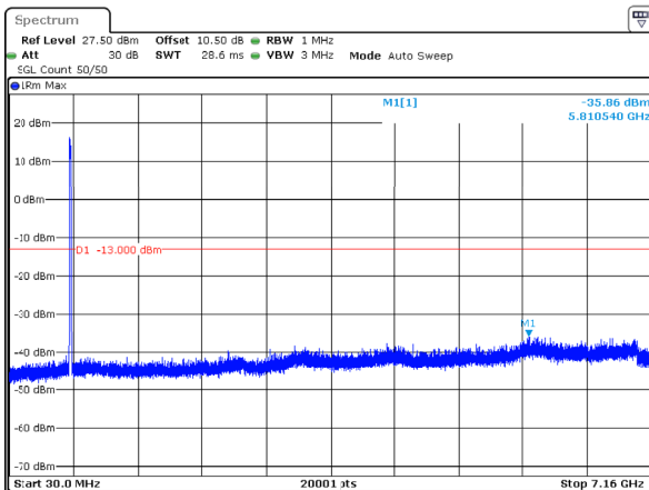
n12_15MHz_15kHz_706.5MHz_DFT-s-OFDM QPSK_RB75@0 -35.86dBm
