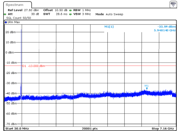
n12_15MHz_15kHz_706.5MHz_DFT-s-OFDM QPSK_RB1@78 -35.99dBm
