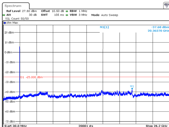
n38_15MHz_30kHz_2595MHz_DFT-s-OFDM QPSK_RB36@0 -37.68dBm
