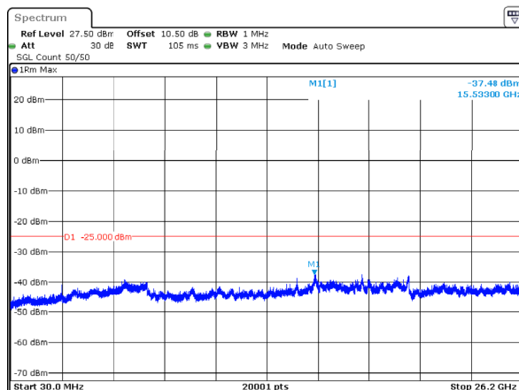
n38_15MHz_30kHz_2612.5MHz_DFT-s-OFDM QPSK_RB1@0 -37.48dBm
