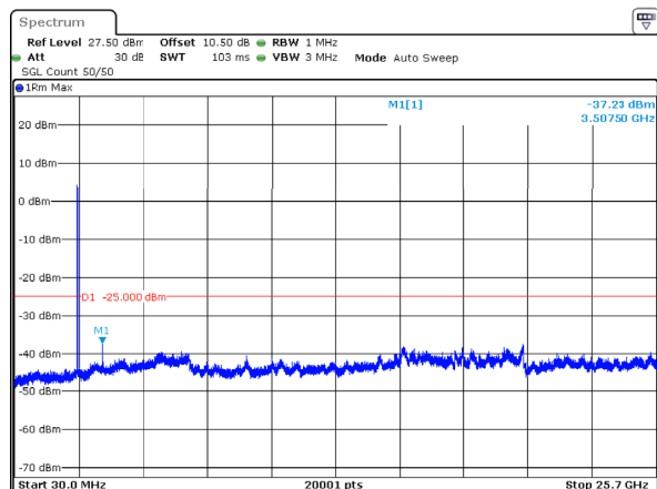
n7_20MHz_15kHz_2510MHz_DFT-s-OFDM QPSK_RB100@0 -37.23dBm
