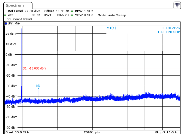
n12_15MHz_15kHz_707.5MHz_DFT-s-OFDM QPSK_RB1@0 -33.30dBm
