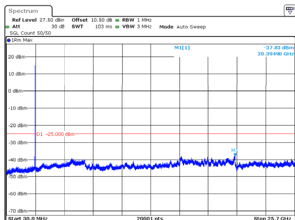
n7_20MHz_15kHz_2510MHz_DFT-s-OFDM QPSK_RB1@105 -37.83dBm
