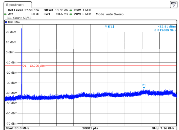
n12_5MHz_15kHz_713.5MHz_DFT-s-OFDM QPSK_RB1@24 -35.81dBm
