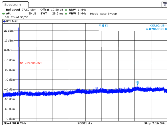
n12_5MHz_15kHz_713.5MHz_DFT-s-OFDM QPSK_RB1@0 -35.62dBm
