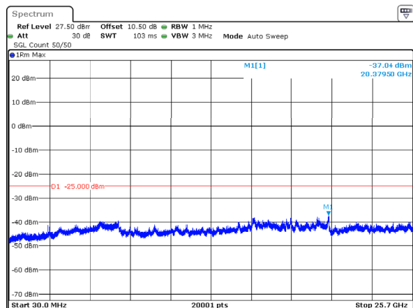
n7_15MHz_15kHz_2562.5MHz_DFT-s-OFDM QPSK_RB1@78 -37.04dBm
