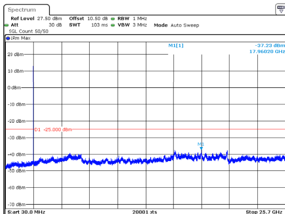
n7_5MHz_15kHz_2567.5MHz_DFT-s-OFDM QPSK_RB1@0 -37.23dBm
