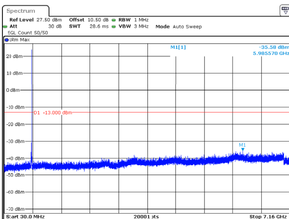
n12_15MHz_15kHz_707.5MHz_DFT-s-OFDM QPSK_RB1@78 -35.58dBm
