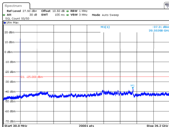
n38_15MHz_30kHz_2595MHz_DFT-s-OFDM QPSK_RB1@37 -37.31dBm
