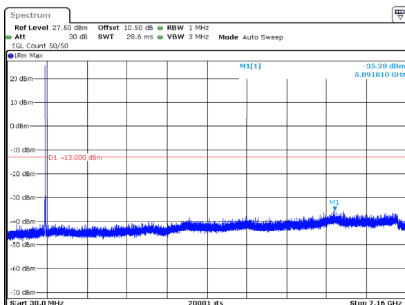
n12_10MHz_15kHz_704MHz_DFT-s-OFDM QPSK_RB1@51 -35.28dBm
