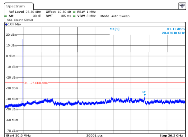
n38_5MHz_15kHz_2572.5MHz_DFT-s-OFDM QPSK_RB1@0 -37.11dBm
