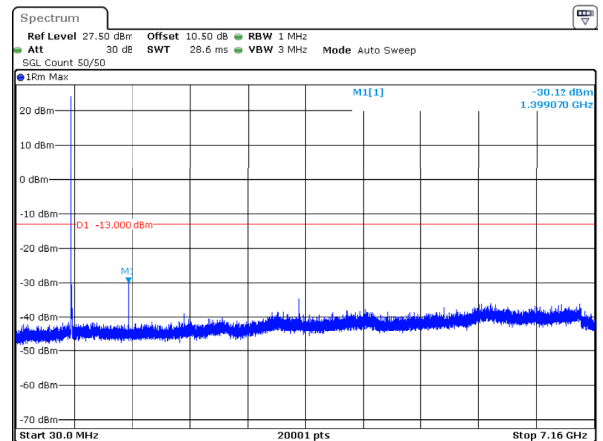
n12_10MHz_15kHz_704MHz_DFT-s-OFDM QPSK_RB1@0 -30.12dBm
