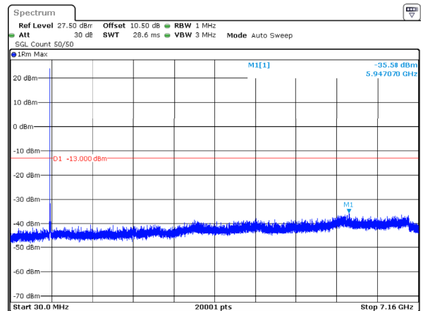
n12_10MHz_15kHz_711MHz_DFT-s-OFDM QPSK_RB1@0 -35.58dBm
