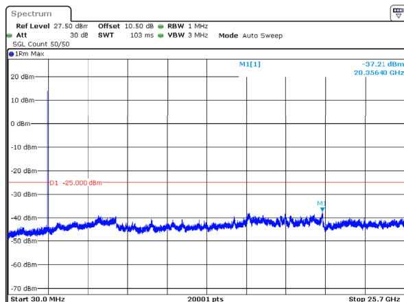
n7_10MHz_15kHz_2535MHz_DFT-s-OFDM QPSK_RB1@51 -37.21dBm
