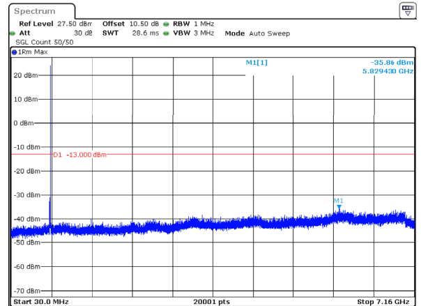
n12_15MHz_15kHz_708.5MHz_DFT-s-OFDM QPSK_RB1@78 -35.86dBm
