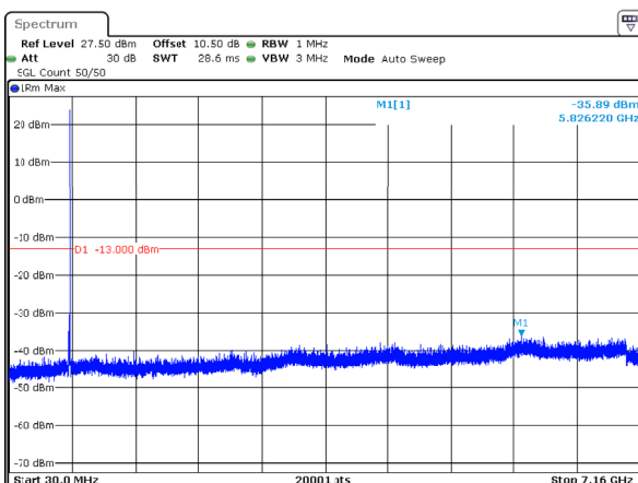
n12_10MHz_15kHz_711MHz_DFT-s-OFDM QPSK_RB1@51 -35.89dBm
