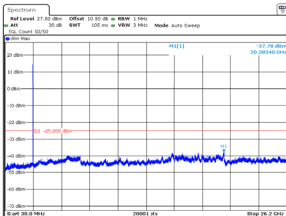
n38_5MHz_15kHz_2572.5MHz_DFT-s-OFDM QPSK_RB1@24 -37.78dBm
