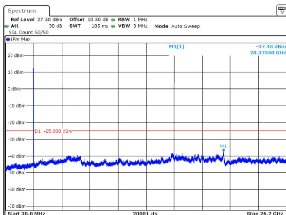
n38_15MHz_30kHz_2612.5MHz_DFT-s-OFDM QPSK_RB1@37 -37.43dBm
