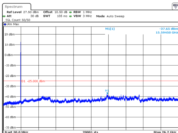
n38_10MHz_30kHz_2595MHz_DFT-s-OFDM QPSK_RB1@23 -37.65dBm
