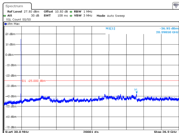
n41_50MHz_30kHz_2592.99MHz_DFT-s-OFDM QPSK_RB1@132 -36.95dBm
