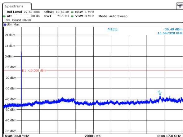
n66_15MHz_15kHz_1772.5MHz_DFT-s-OFDM QPSK_RB75@0 -36.49dBm
