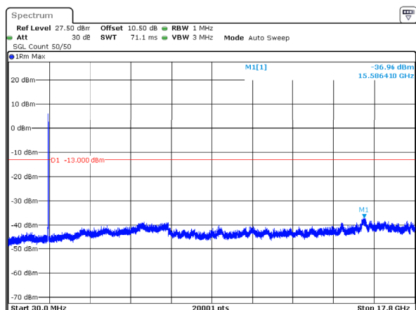
n66_15MHz_15kHz_1745MHz_DFT-s-OFDM QPSK_RB75@0 -36.96dBm
