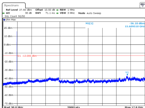
n66_25MHz_15kHz_1745MHz_DFT-s-OFDM QPSK_RB1@0 -36.10dBm
