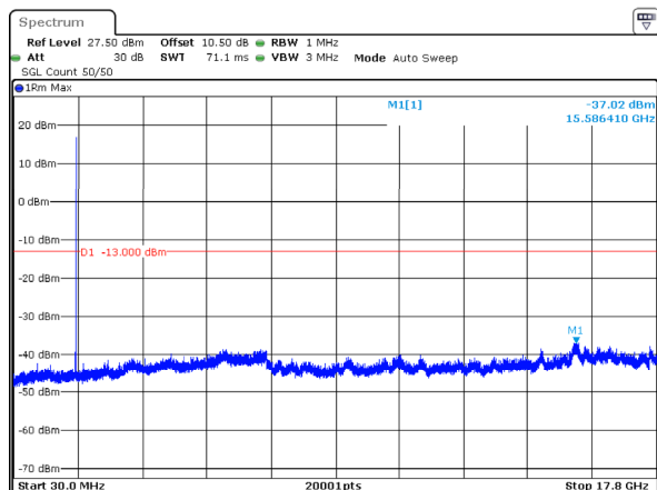
n66_25MHz_15kHz_1722.5MHz_DFT-s-OFDM QPSK_RB1@132 -37.02dBm
