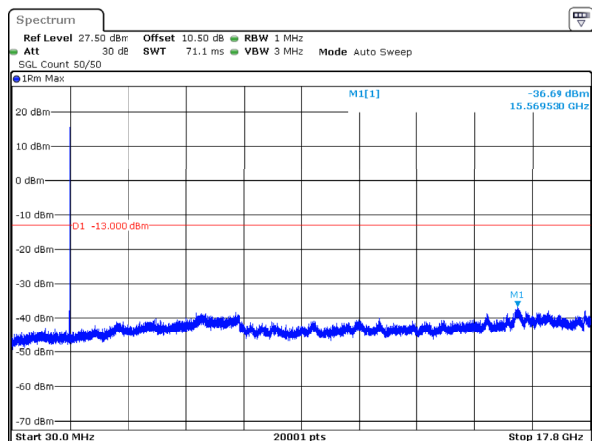
n66_15MHz_15kHz_1772.5MHz_DFT-s-OFDM QPSK_RB1@78 -36.69dBm
