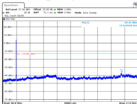
n66_30MHz_15kHz_1725MHz_DFT-s-OFDM QPSK_RB160@0 -36.67dBm
