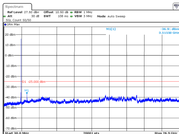
n41_40MHz_30kHz_2592.99MHz_DFT-s-OFDM QPSK_RB1@105 -36.91dBm
