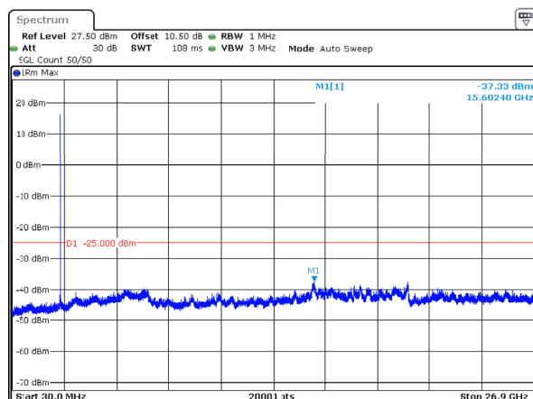
n41_30MHz_30kHz_2511MHz_DFT-s-OFDM QPSK_RB1@77 -37.33dBm
