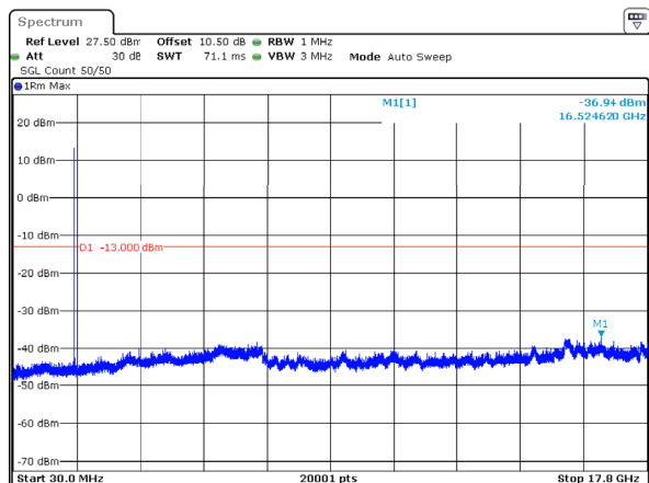
n66_15MHz_15kHz_1717.5MHz_DFT-s-OFDM QPSK_RB1@78 -36.94dBm
