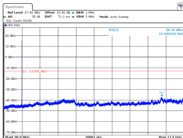
n66_25MHz_15kHz_1745MHz_DFT-s-OFDM QPSK_RB1@132 -36.47dBm
