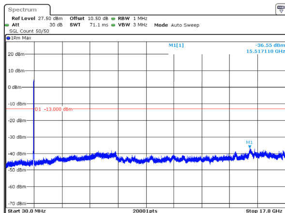
n66_25MHz_15kHz_1767.5MHz_DFT-s-OFDM QPSK_RB128@0 -36.55dBm
