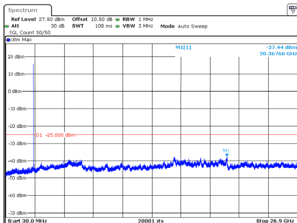
n41_30MHz_30kHz_2592.99MHz_DFT-s-OFDM QPSK_RB1@0 -37.44dBm
