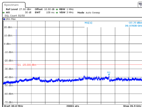
n41_20MHz_30kHz_2506.02MHz_DFT-s-OFDM QPSK_RB1@50 -37.72dBm
