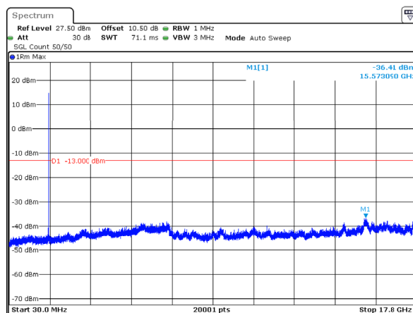
n66_30MHz_15kHz_1725MHz_DFT-s-OFDM QPSK_RB1@159 -36.41dBm
