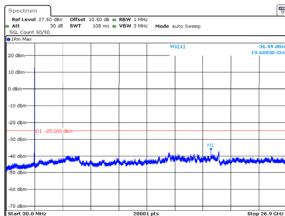
n41_50MHz_30kHz_2664.99MHz_DFT-s-OFDM QPSK_RB1@132 -36.89dBm
