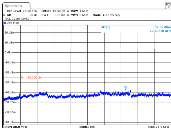
n41_100MHz_30kHz_2592.99MHz_DFT-s-OFDM QPSK_RB1@272 -37.85dBm
