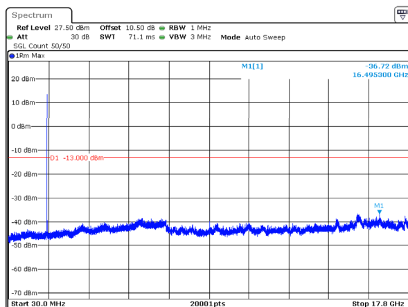
n66_30MHz_15kHz_1725MHz_DFT-s-OFDM QPSK_RB1@0 -36.72dBm
