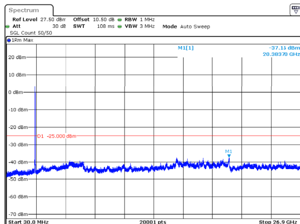
n41_40MHz_30kHz_2592.99MHz_DFT-s-OFDM QPSK_RB100@0 -37.15dBm
