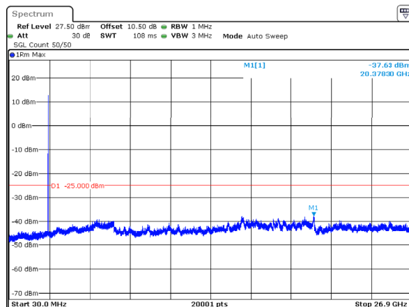
n41_15MHz_30kHz_2592.99MHz_DFT-s-OFDM QPSK_RB1@37 -37.63dBm
