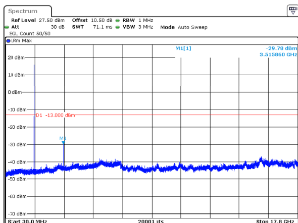
n66_15MHz_15kHz_1745MHz_DFT-s-OFDM QPSK_RB1@78 -29.78dBm
