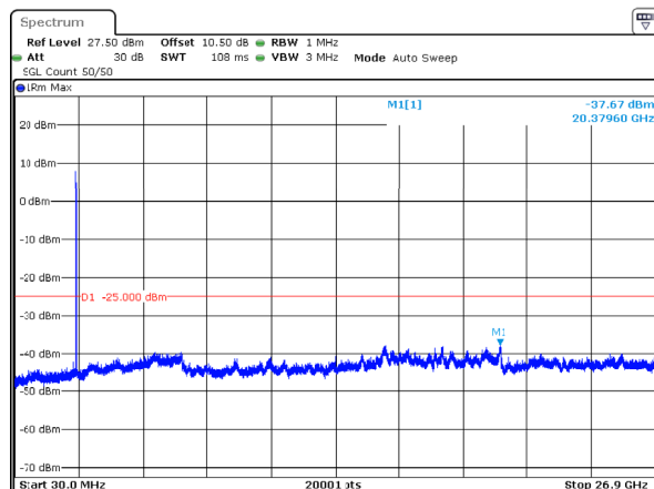
n41_15MHz_30kHz_2592.99MHz_DFT-s-OFDM QPSK_RB36@0 -37.67dBm
