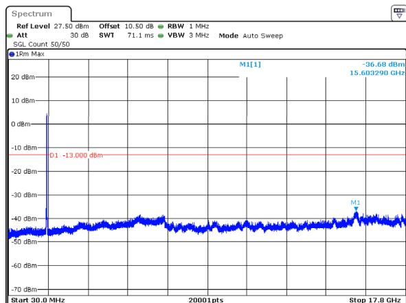
n66_25MHz_15kHz_1722.5MHz_DFT-s-OFDM QPSK_RB128@0 -36.68dBm
