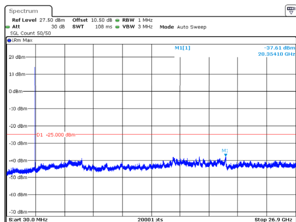
n41_50MHz_30kHz_2664.99MHz_DFT-s-OFDM QPSK_RB1@0 -37.61dBm
