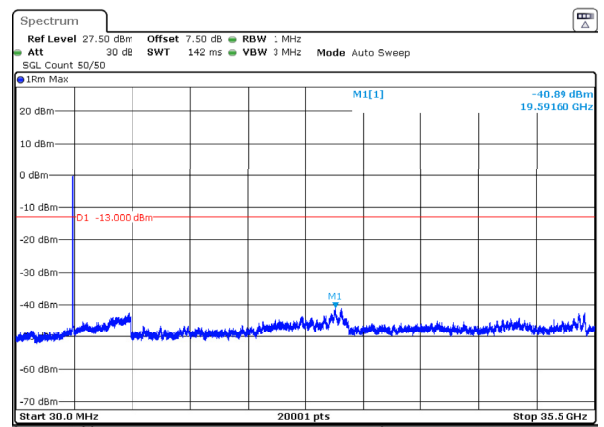
n77_1_50MHz_30kHz_3475MHz_DFT-s-OFDM QPSK_RB128@0 -40.89dBm
