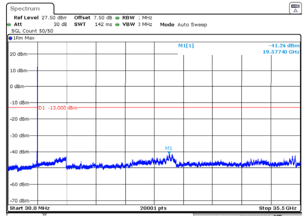
n77_1_40MHz_30kHz_3500MHz_DFT-s-OFDM QPSK_RB1@105 -41.26dBm
