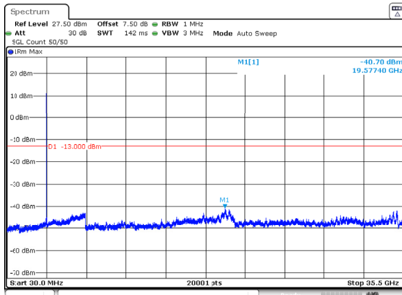
n77_1_30MHz_30kHz_3535MHz_DFT-s-OFDM QPSK_RB1@77 -40.70dBm
