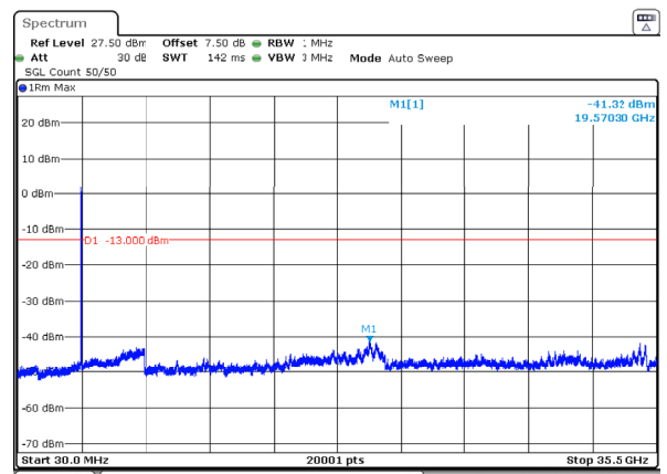
n77_1_40MHz_30kHz_3500MHz_DFT-s-OFDM QPSK_RB100@0 -41.32dBm
