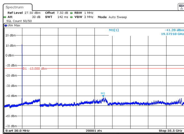
n77_1_50MHz_30kHz_3500MHz_DFT-s-OFDM QPSK_RB1@132 -41.20dBm
