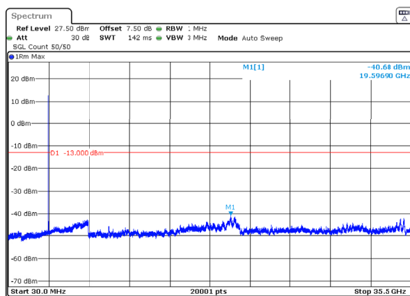
n77_1_20MHz_30kHz_3500MHz_DFT-s-OFDM QPSK_RB1@0 -40.68dBm
