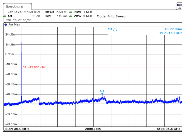
n77_1_50MHz_30kHz_3475MHz_DFT-s-OFDM QPSK_RB1@0 -40.77dBm
