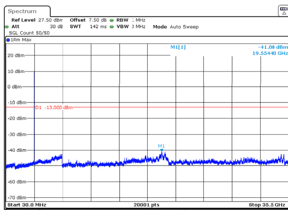
n77_1_15MHz_30kHz_3542.5MHz_DFT-s-OFDM QPSK_RB1@0 -41dBm
