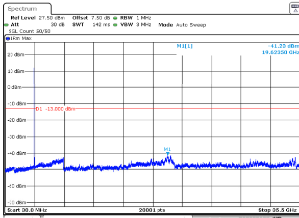
n77_1_40MHz_30kHz_3500MHz_DFT-s-OFDM QPSK_RB1@0 -41.23dBm
