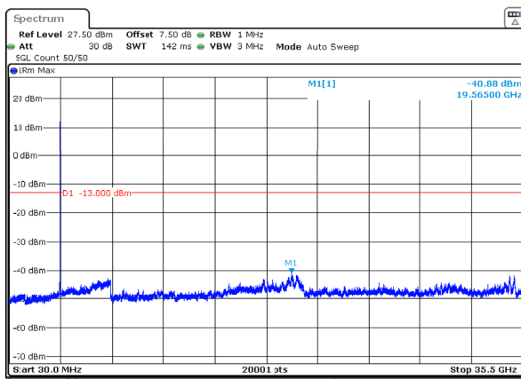
n77_1_40MHz_30kHz_3530MHz_DFT-s-OFDM QPSK_RB1@105 -40.88dBm
