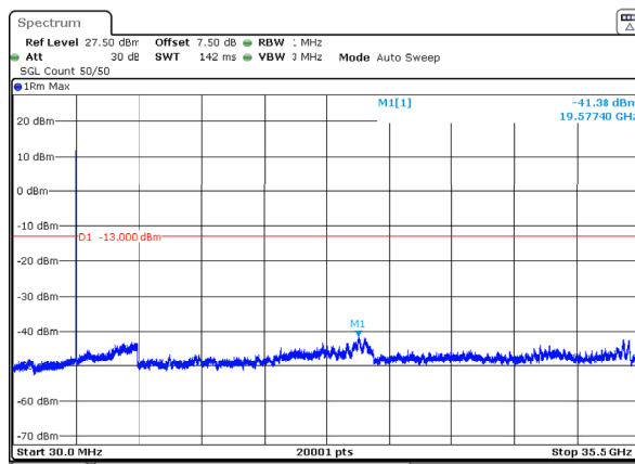
n77_1_20MHz_30kHz_3540MHz_DFT-s-OFDM QPSK_RB1@50 -41.38dBm
