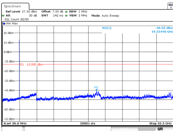
n77_1_10MHz_30kHz_3500MHz_DFT-s-OFDM QPSK_RB1@0 -40.55dBm
