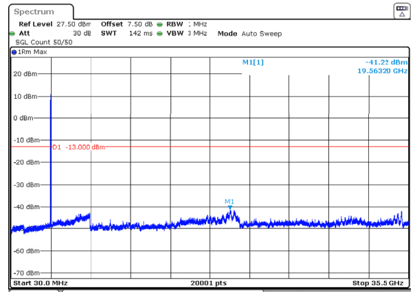
n77_1_40MHz_30kHz_3530MHz_DFT-s-OFDM QPSK_RB1@0 -41.22dBm
