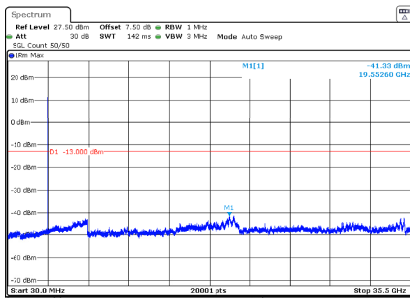
n77_1_15MHz_30kHz_3542.5MHz_DFT-s-OFDM QPSK_RB1@37 -41.33dBm
