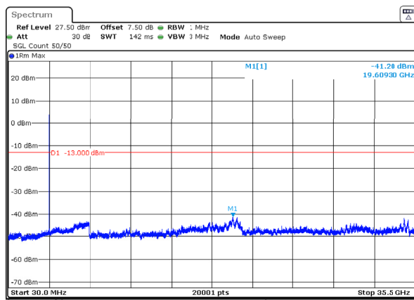
n77_1_15MHz_30kHz_3542.5MHz_DFT-s-OFDM QPSK_RB36@0 -41.20dBm
