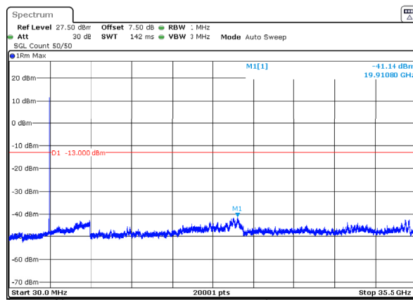
n77_1_50MHz_30kHz_3475MHz_DFT-s-OFDM QPSK_RB1@132 -41.14dBm
