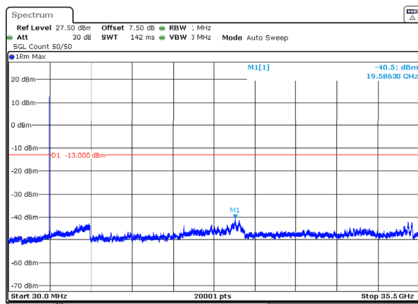
n77_1_15MHz_30kHz_3500MHz_DFT-s-OFDM QPSK_RB1@37 -40.51dBm
