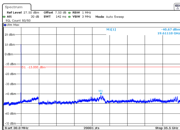
n77_1_70MHz_30kHz_3500MHz_DFT-s-OFDM QPSK_RB1@188 -40.67dBm
