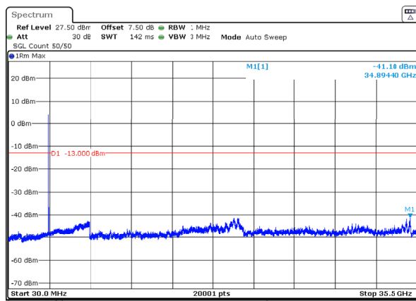
n77_1_15MHz_30kHz_3457.5MHz_DFT-s-OFDM QPSK_RB36@0 -41.10dBm
