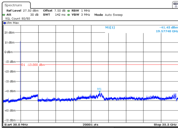
n77_1_30MHz_30kHz_3500MHz_DFT-s-OFDM QPSK_RB1@0 -41.45dBm
