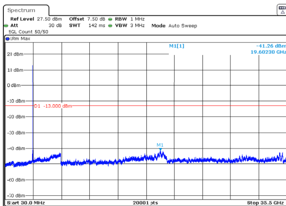
n77_1_60MHz_30kHz_3480MHz_DFT-s-OFDM QPSK_RB1@161 -41.26dBm
