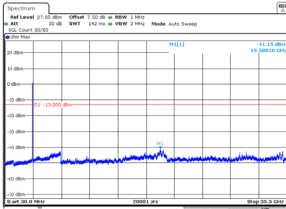
n77_1_40MHz_30kHz_3470MHz_DFT-s-OFDM QPSK_RB100@0 -41.15dBm
