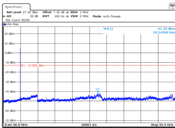
n77_1_15MHz_30kHz_3500MHz_DFT-s-OFDM QPSK_RB36@0 -41.23dBm
