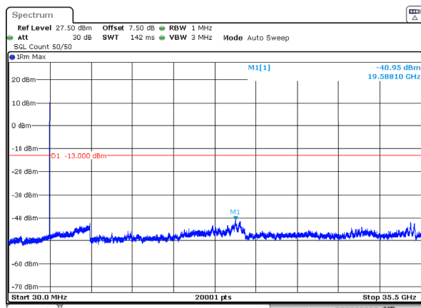
n77_1_10MHz_30kHz_3545MHz_DFT-s-OFDM QPSK_RB1@0 -40.95dBm
