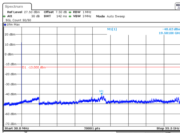
n77_1_10MHz_30kHz_3545MHz_DFT-s-OFDM QPSK_RB1@23 -40.62dBm
