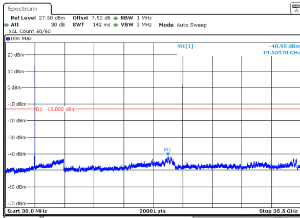
n77_1_50MHz_30kHz_3525MHz_DFT-s-OFDM QPSK_RB1@0 -40.95dBm
