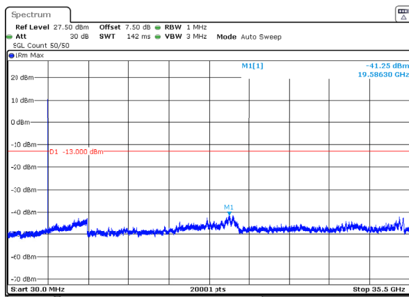
n77_1_20MHz_30kHz_3540MHz_DFT-s-OFDM QPSK_RB1@0 -41.25dBm
