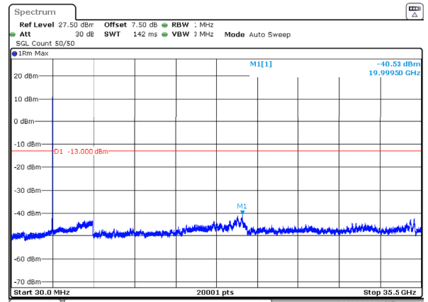
n77_1_50MHz_30kHz_3525MHz_DFT-s-OFDM QPSK_RB1@132 -40.53dBm
