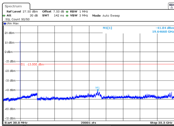
n77_1_15MHz_30kHz_3500MHz_DFT-s-OFDM QPSK_RB1@0 -41.04dBm
