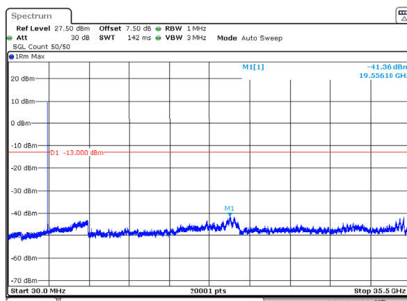
n77_1_15MHz_30kHz_3457.5MHz_DFT-s-OFDM QPSK_RB1@0 -41.36dBm
