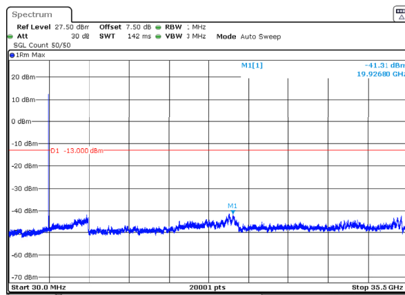
n77_1_50MHz_30kHz_3500MHz_DFT-s-OFDM QPSK_RB1@0 -41.31dBm
