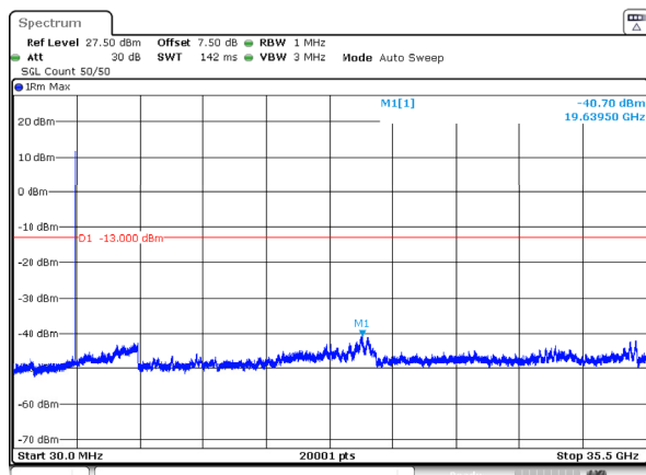
n77_1_10MHz_30kHz_3500MHz_DFT-s-OFDM QPSK_RB1@23 -40.70dBm
