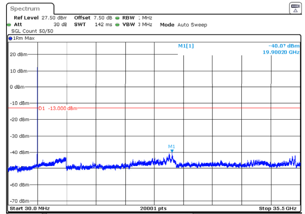
n77_1_30MHz_30kHz_3500MHz_DFT-s-OFDM QPSK_RB1@77 -40.07dBm
