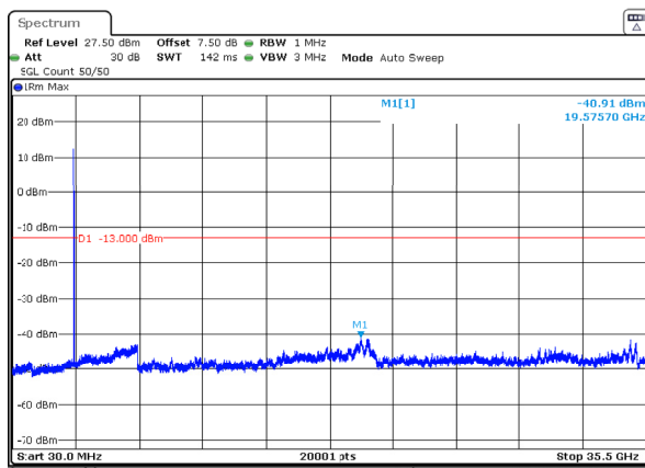
n77_1_15MHz_30kHz_3457.5MHz_DFT-s-OFDM QPSK_RB1@37 -40.91dBm
