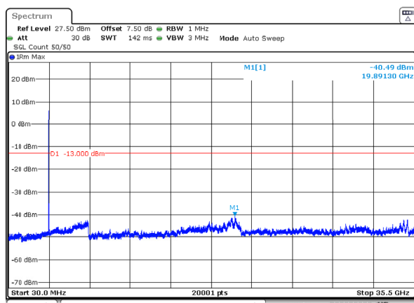
n77_1_10MHz_30kHz_3545MHz_DFT-s-OFDM QPSK_RB24@0 -40.49dBm
