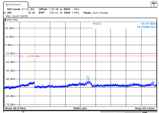
n77_1_30MHz_30kHz_3535MHz_DFT-s-OFDM QPSK_RB75@0 -40.97dBm
