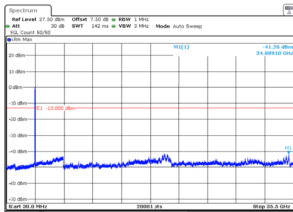
n77_1_50MHz_30kHz_3500MHz_DFT-s-OFDM QPSK_RB128@0 -41.26dBm
