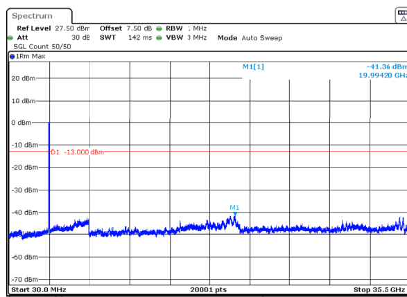
n77_1_50MHz_30kHz_3525MHz_DFT-s-OFDM QPSK_RB128@0 -41.36dBm
