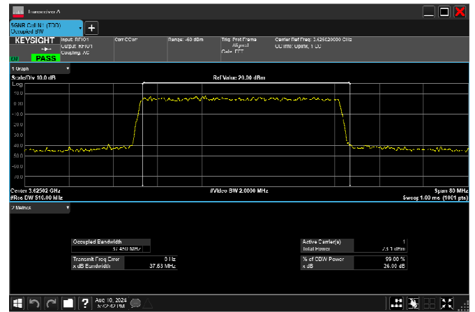
n77_2_40MHz_30kHz_3625MHz_DFT-s-OFDM 64 QAM_RB100@0 37.126MHz
