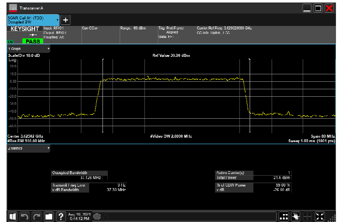
n77_2_40MHz_30kHz_3625MHz_CP-OFDM QPSK_RB106@0 37.676MHz
