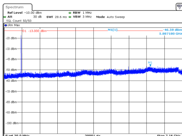
n12_5MHz_15kHz_713.5MHz_DFT-s-OFDM QPSK_RB1@0 -46.59dBm
