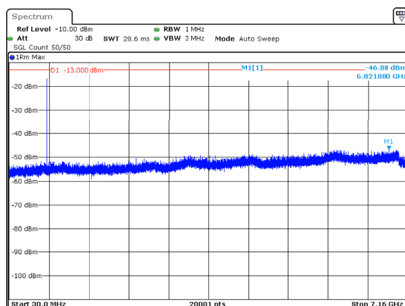
n12_10MHz_15kHz_704MHz_DFT-s-OFDM QPSK_RB1@0 -46.80dBm
