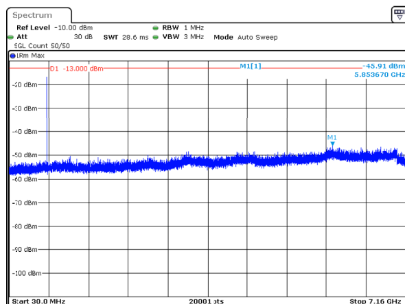
n12_10MHz_15kHz_704MHz_DFT-s-OFDM QPSK_RB1@51 -45.91dBm
