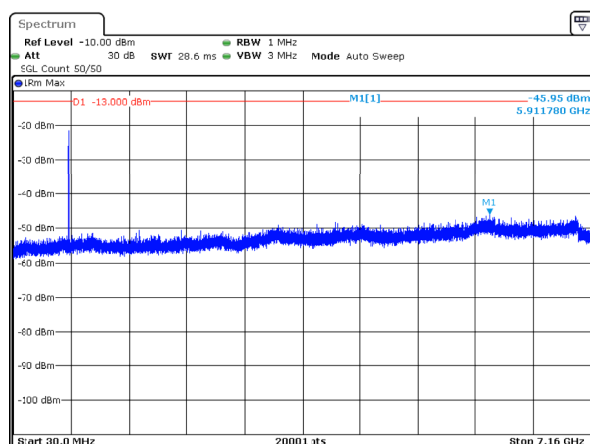
n12_5MHz_15kHz_713.5MHz_DFT-s-OFDM QPSK_RB25@0 -45.95dBm
