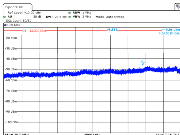
n12_5MHz_15kHz_713.5MHz_DFT-s-OFDM QPSK_RB1@24 -46.06dBm
