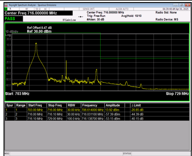
Band17-10MHz-64QAM-23800-50RB#0
