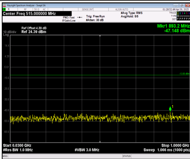
Band2-20MHz-64QAM-19100-1RB#0-Range1:30~1000MHz
