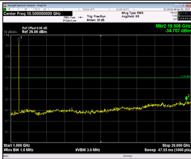
Band2-20MHz-64QAM-19100-1RB#0-Range2:1000~20000MHz
