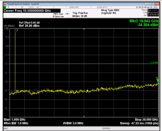
Band4-1.4MHz-64QAM-20393-1RB#0-Range2:1000~20000MHz
