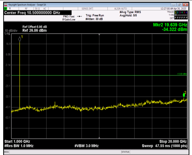
Band2-1.4MHz-64QAM-18607-1RB#0-Range2:1000~20000MHz
