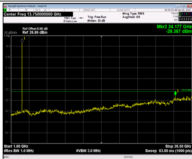
Band7-20MHz-16QAM-20850-1RB#0-Range2:1000~ 26500MHz
