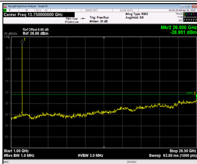
Band7-20MHz-64QAM-21350-1RB#0-Range2:1000~26500MHz
