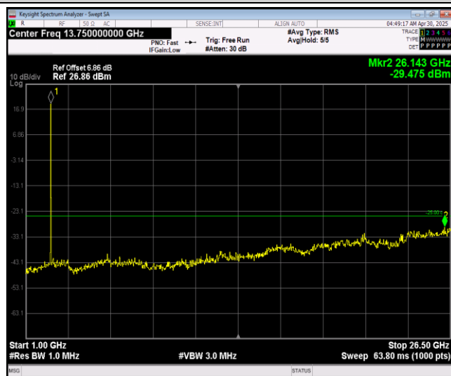
Band7-20MHz-16QAM-21100-1RB#0-Range2:1000~ 26500MHz
