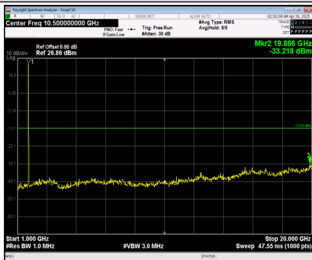
Band4-20MHz-16QAM-20300-1RB#0-Range2:1000~20000MHz
