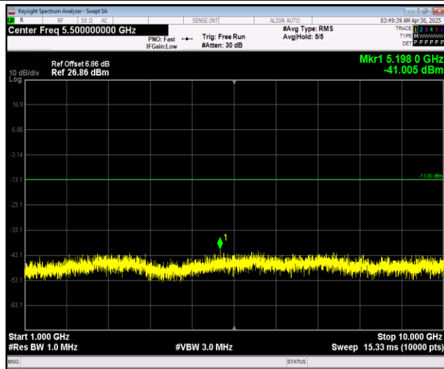
Band5-10MHz-64QAM-20450-1RB#0-Range2:1000~10000MHz
