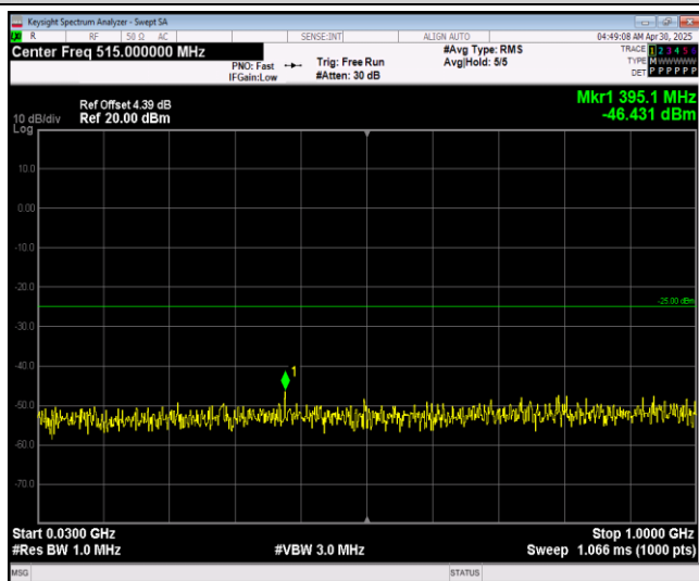
Band7-20MHz-16QAM-21100-1RB#0-Range1:30~10 00MHz
