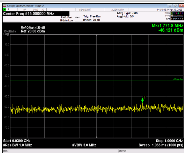
Band7-20MHz-16QAM-20850-1RB#0-Range1:30~10 00MHz
