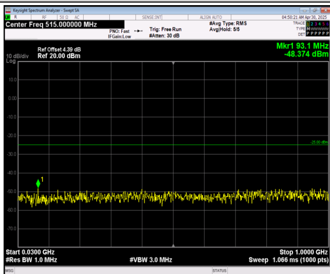
Band7-20MHz-64QAM-21350-1RB#0-Range1:30~1000MHz
