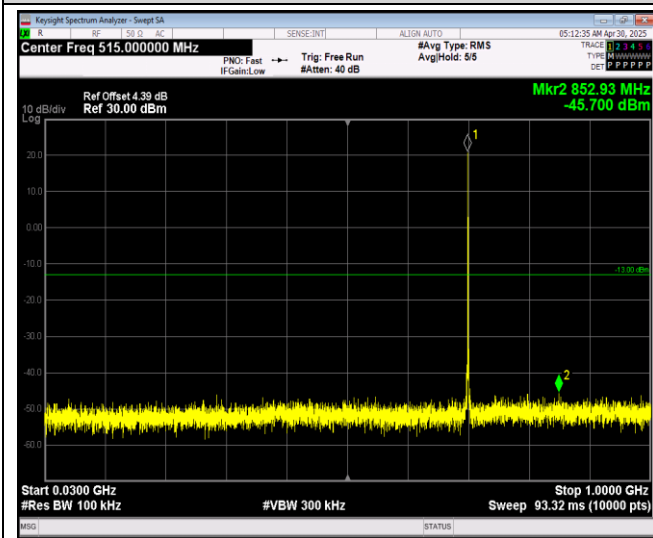
Band12-1.4MHz-64QAM-23095-1RB#0-Range1:30~1 000MHz
