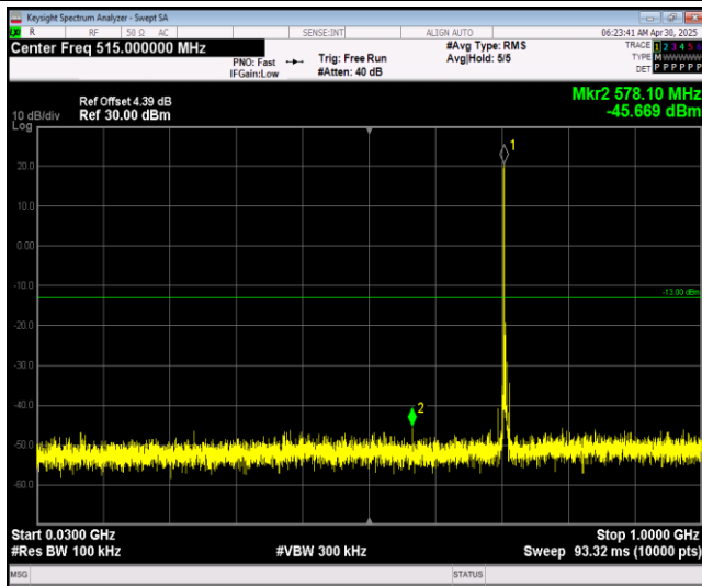
Band17-5MHz-64QAM-23755-1RB#0-Range1:30~1000MHz
