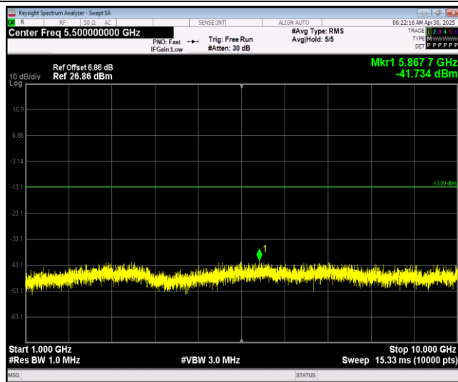
Band17-5MHz-64QAM-23790-1RB#0-Range2:1000~10000MHz
