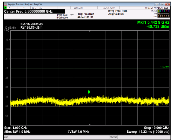
Band12-1.4MHz-16QAM-23095-1RB#0-Range2:1000 ~10000MHz
