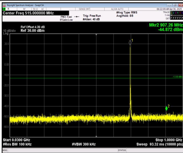
Band17-5MHz-64QAM-23790-1RB#0-Range1:30~1000MHz
