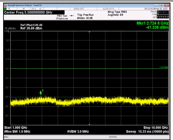
Band12-1.4MHz-64QAM-23095-1RB#0-Range2:1000 ~10000MHz
