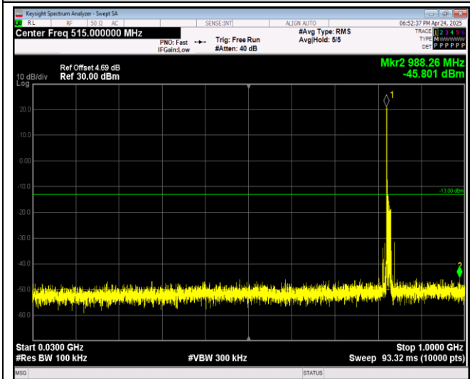
Band5-10MHz-16QAM-20525-1RB#0-Range1:30~1000MHz
