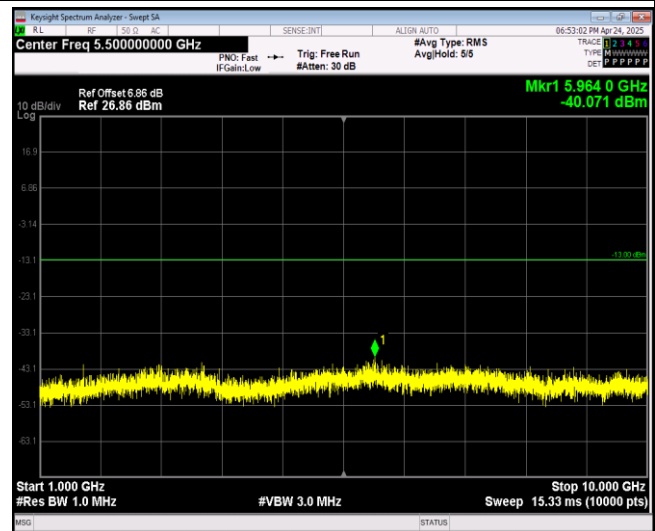
Band5-10MHz-64QAM-20525-1RB#0-Range2:1000~10000MHz
