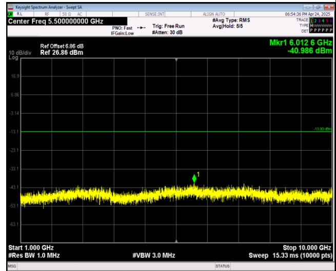
Band5-10MHz-64QAM-20450-1RB#0-Range2:1000~10000MHz
