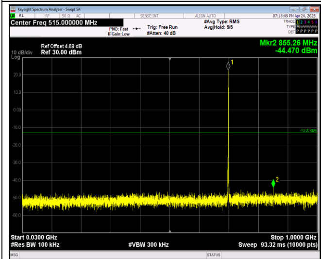
Band12-1.4MHz-QPSK-23173-1RB#0-Range1:30~1000MHz
