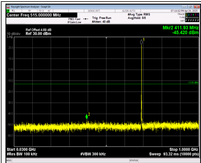
Band12-1.4MHz-QPSK-23095-1RB#0-Range1:30~1000MHz
