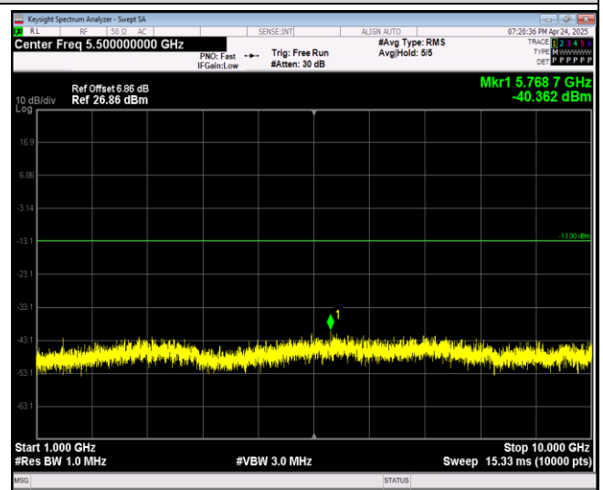
Band12-1.4MHz-QPSK-23173-1RB#0-Range2:1000~10000MHz
