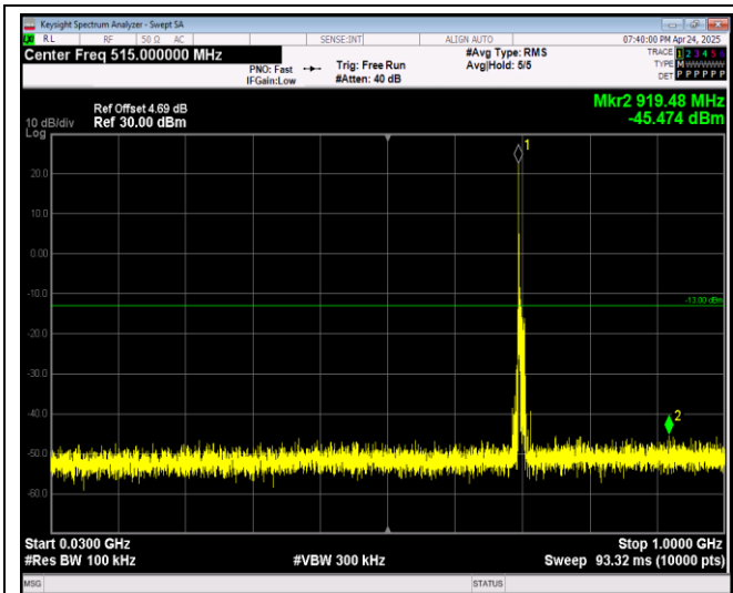
Band12-10MHz-QPSK-23130-1RB#0-Range1:30~1000MHz
