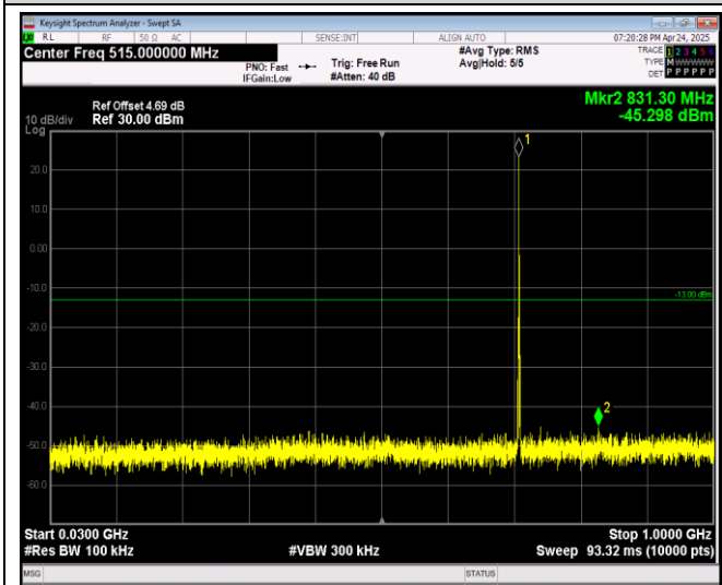
Band12-1.4MHz-QPSK-23173-1RB#0-Range1:30~1000MHz
