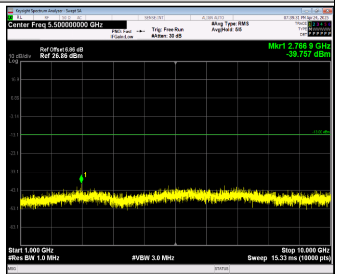
Band12-10MHz-16QAM-23060-1RB#0-Range2:1000~10000MHz
