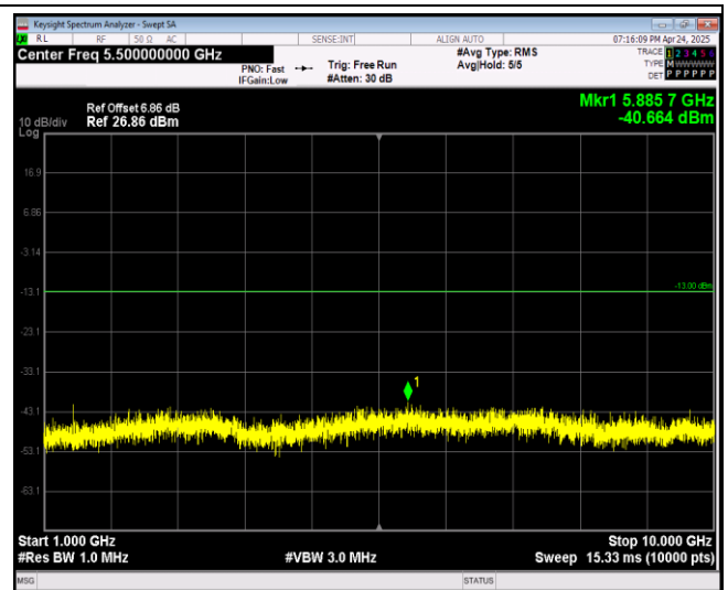
Band12-1.4MHz-QPSK-23095-1RB#0-Range2:1000~10000MHz
