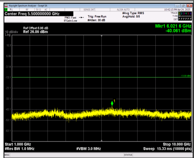
Band26-1.4MHz-64QAM-26783-1RB#0-Range2:1000~10000MHz
