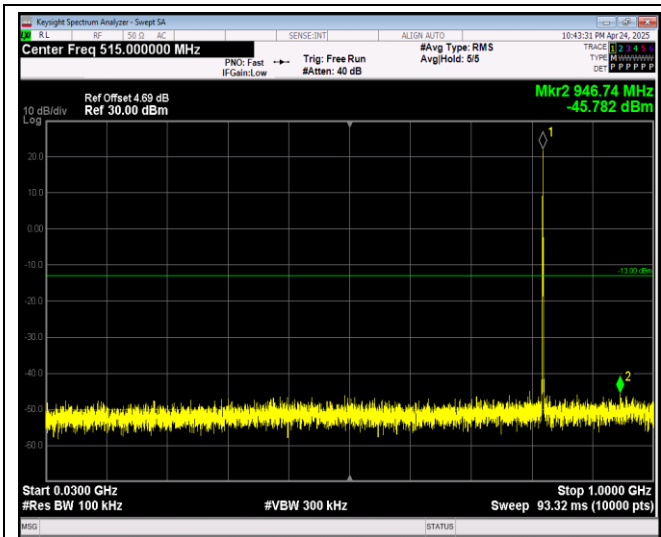
Band26-1.4MHz-QPSK-26797-1RB#0-Range1:30~1000MHz
