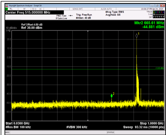
Band26-15MHz-64QAM-26915-1RB#0-Range1:30~1 000MHz
