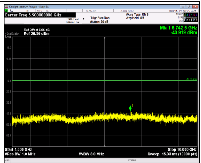
Band17-10MHz-64QAM-23790-1RB#0-Range2:1000 ~10000MHz
