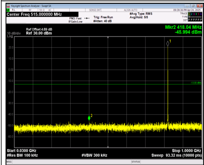
Band26-1.4MHz-QPSK-26915-1RB#0-Range1:30~1000MHz
