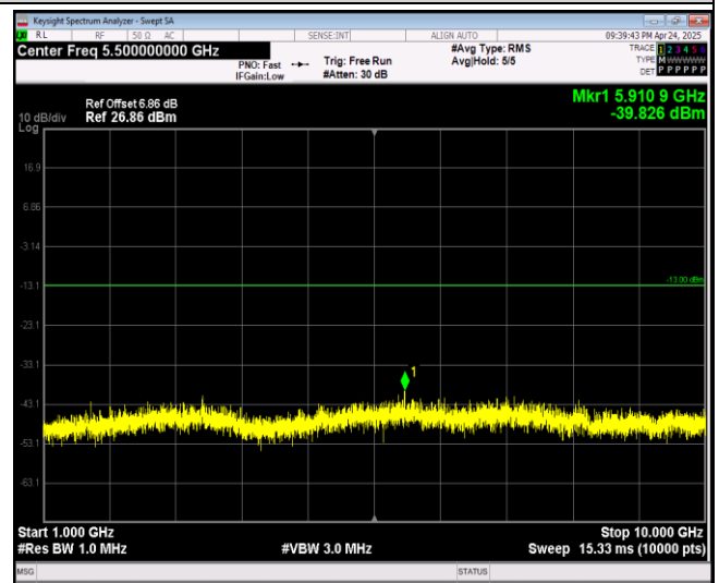
Band26-1.4MHz-QPSK-26915-1RB#0-Range2:1000~10000MHz
