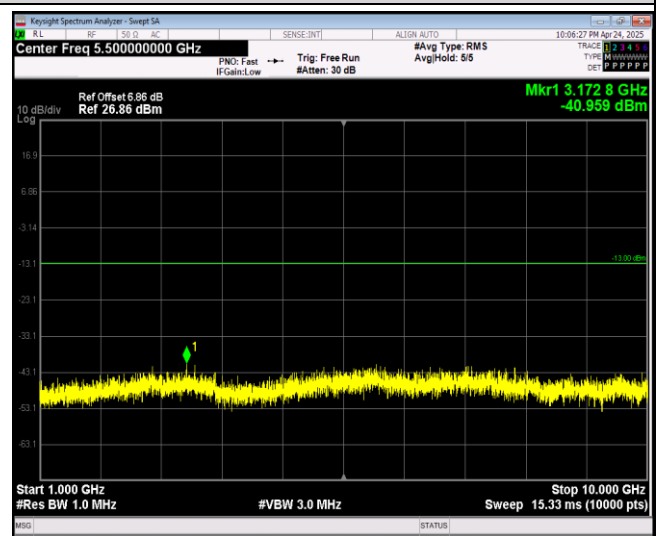
Band26-15MHz-16QAM-26865-1RB#0-Range2:1000~10000MHz
