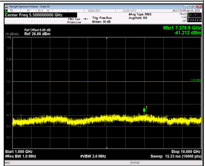
Band17-10MHz-64QAM-23800-1RB#0-Range2:1000 ~10000MHz
