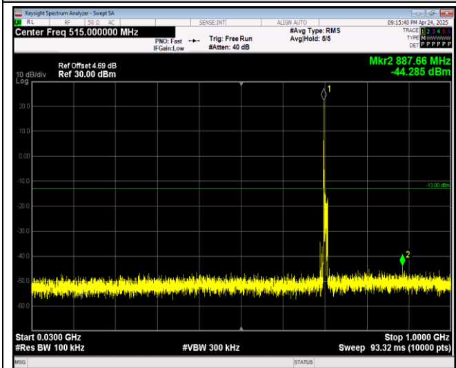
Band17-10MHz-64QAM-23800-1RB#0-Range1:30~1 000MHz
