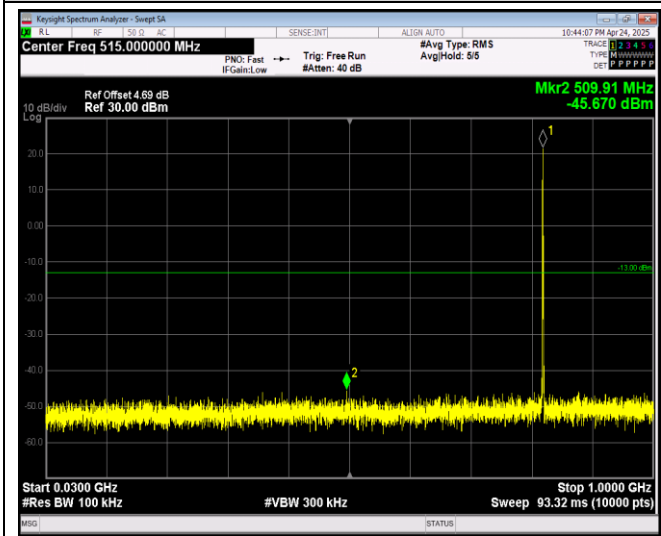
Band26-1.4MHz-64QAM-26783-1RB#0-Range1:30~1000MHz
