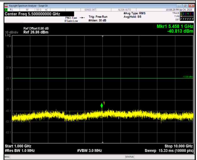
Band26-15MHz-64QAM-26965-1RB#0-Range2:1000 ~10000MHz
