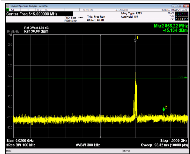
Band17-10MHz-64QAM-23800-1RB#0-Range1:30~1 000MHz
