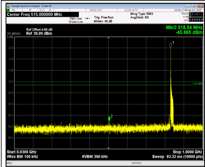
Band26-15MHz-64QAM-26965-1RB#0-Range1:30~1 000MHz
