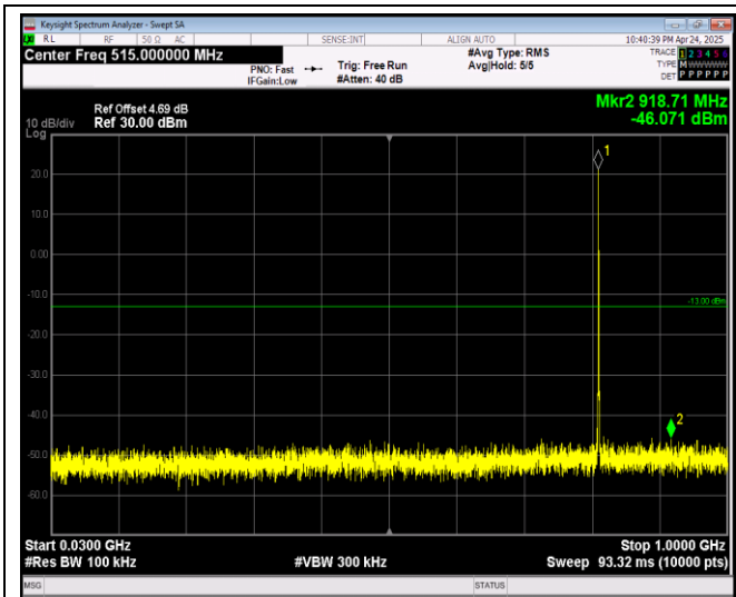
Band26-1.4MHz-64QAM-26740-1RB#0-Range1:30~1000MHz
