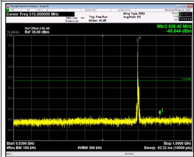
Band17-10MHz-16QAM-23780-1RB#0-Range1:30~1000MHz
