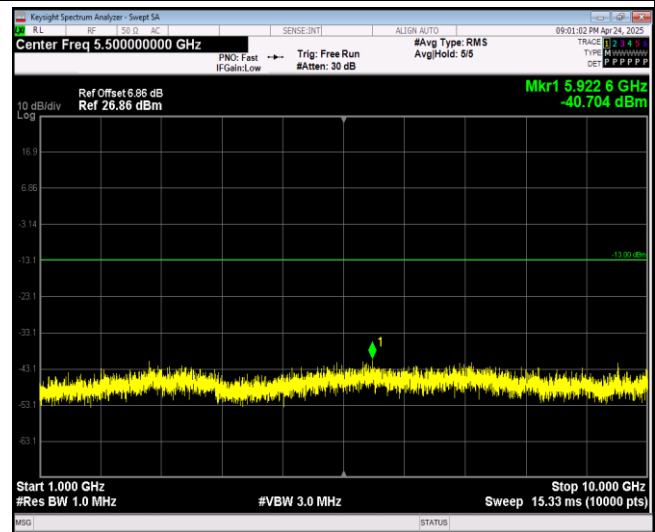
Band17-10MHz-QPSK-23780-1RB#0-Range2:1000~10000MHz
