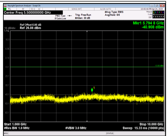
Band26-1.4MHz-64QAM-26740-1RB#0-Range2:1000~10000MHz
