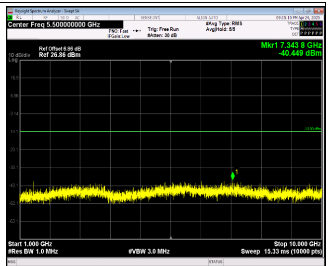
Band17-10MHz-QPSK-23800-1RB#0-Range2:1000~10000MHz
