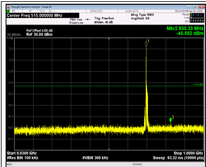
Band17-10MHz-64QAM-23790-1RB#0-Range1:30~1 000MHz
