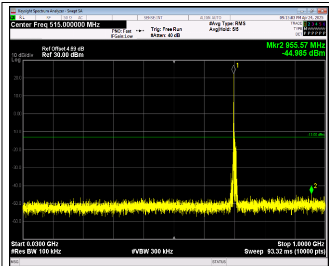
Band17-10MHz-QPSK-23800-1RB#0-Range1:30~1000MHz
