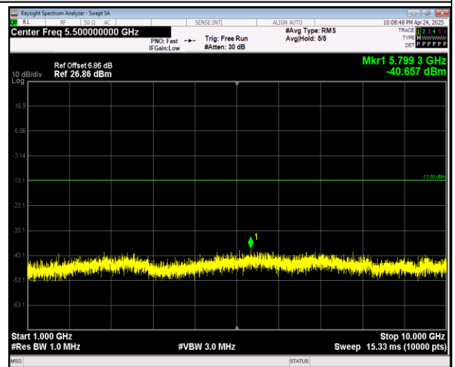
Band26-15MHz-16QAM-26865-1RB#0-Range2:1000~10000MHz
