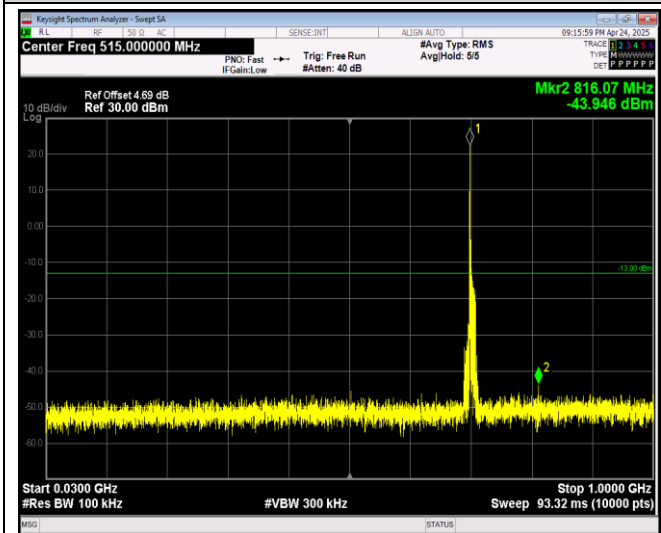
Band17-10MHz-16QAM-23780-1RB#0-Range1:30~1000MHz
