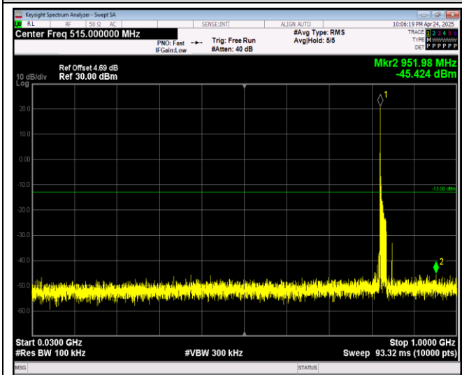
Band26-15MHz-16QAM-26865-1RB#0-Range1:30~1000MHz
