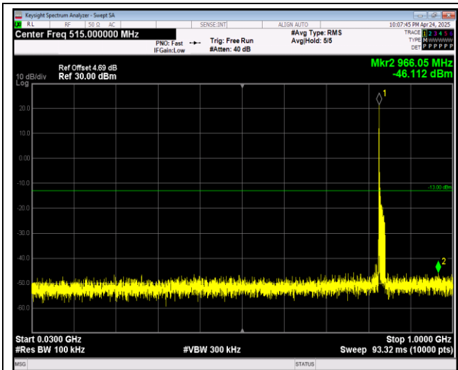
Band26-15MHz-QPSK-26965-1RB#0-Range1:30~1000MHz
