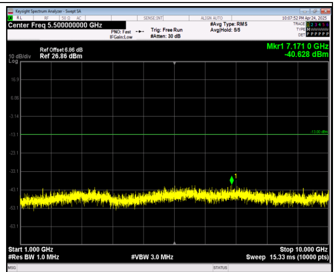
Band26-15MHz-QPSK-26965-1RB#0-Range2:1000~10000MHz
