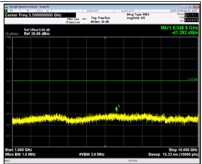
Band26-15MHz-64QAM-26915-1RB#0-Range2:1000 ~10000MHz
