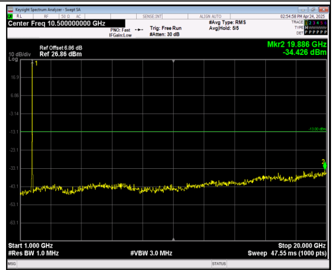
Band66-20MHz-16QAM-132572-1RB#0-Range2:1000~20000MHz
