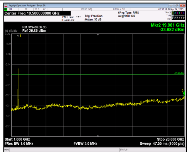
Band66-20MHz-16QAM-132572-1RB#0-Range2:1000~20000MHz
