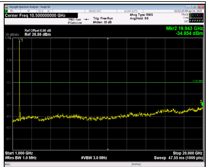
Band66-20MHz-16QAM-132322-1RB#0-Range2:1000~20000MHz
