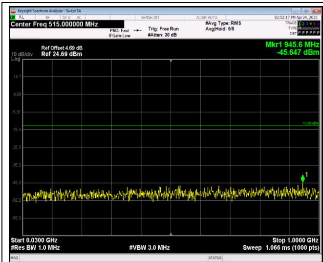
Band66-20MHz-16QAM-132322-1RB#0-Range1:30~1000MHz
