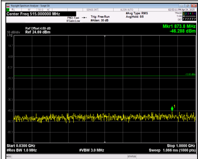
Band66-20MHz-16QAM-132572-1RB#0-Range1:30~1000MHz
