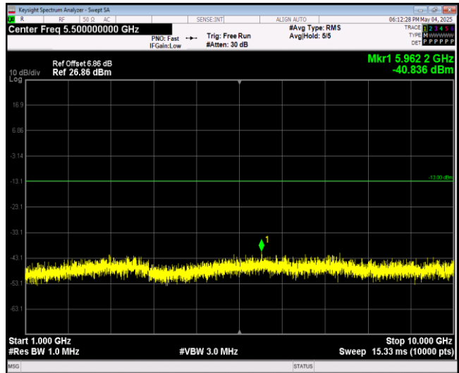
Band17-5MHz-16QAM-23790-1RB#0-Range2:1000~10000MHz
