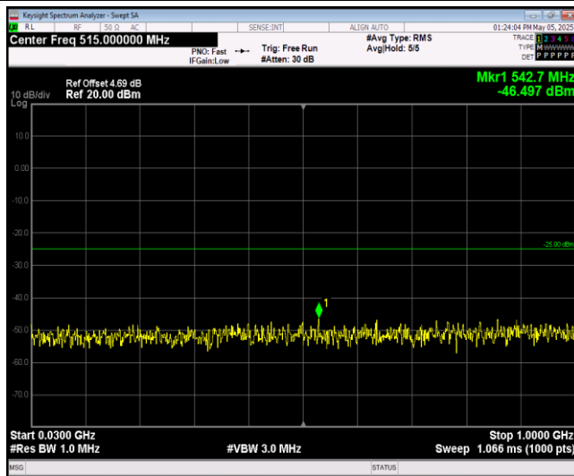
Band38-20MHz-QPSK-38150-1RB#0-Range1:30~1000MHz
