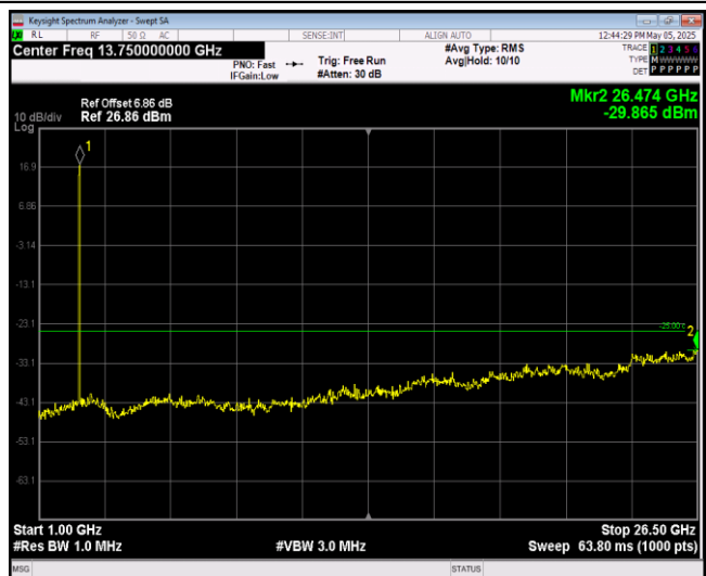
Band38-5MHz-64QAM-38000-1RB#0-Range2:1000~26500MHz
