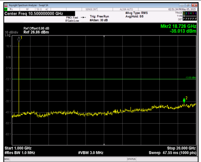
Band66-1.4MHz-16QAM-132665-1RB#0-Range2:1000~20000MHz
