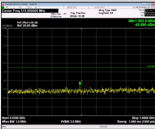
Band41-5MHz-64QAM-41215-1RB#0-Range1:30~1000MHz
