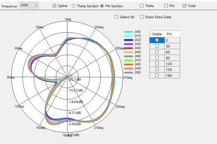
2.4G WIFI Phi=0deg
