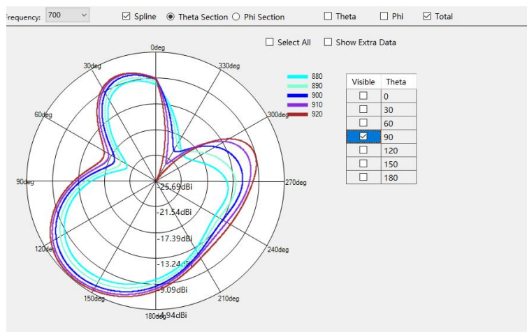
GSM900 WCDMA B8 LTE B8 Theta=90deg
