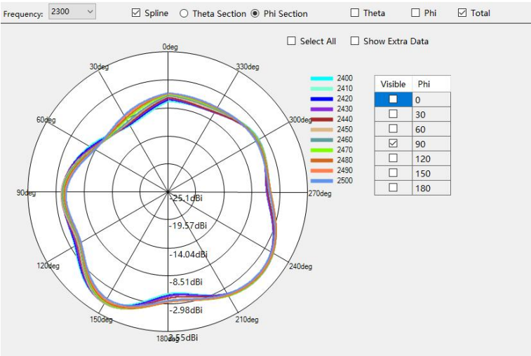
2.4G WIFI Phi=90deg
