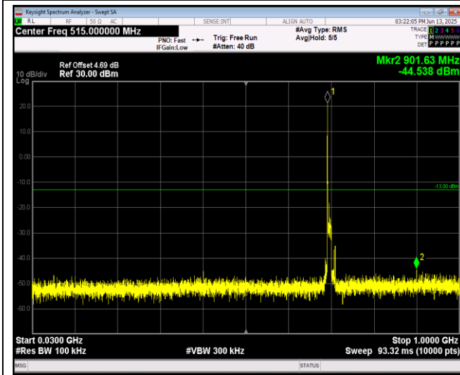
Band12-10MHz-16QAM-23060-1RB#0-Range1:30~1000MHz
