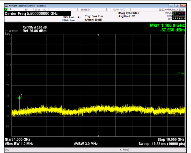
Band12-10MHz-QPSK-23130-1RB#0-Range2:1000~10000MHz
