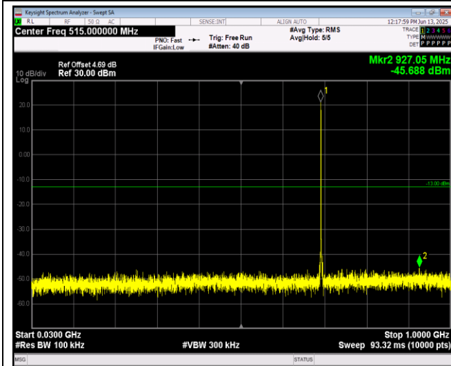
Band12-1.4MHz-64QAM-23095-1RB#0-Range1:30~1000MHz
