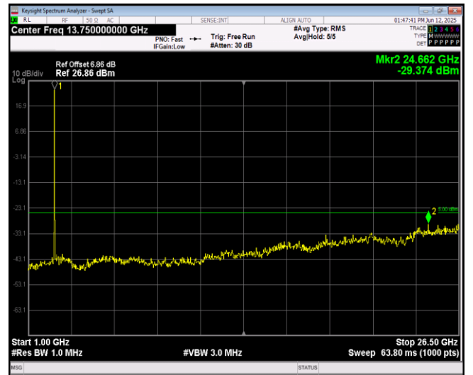
Band7-20MHz-16QAM-20850-1RB#0-Range2:1000~2 6500MHz
