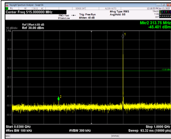
Band12-1.4MHz-64QAM-23095-1RB#0-Range1:30~1000MHz
