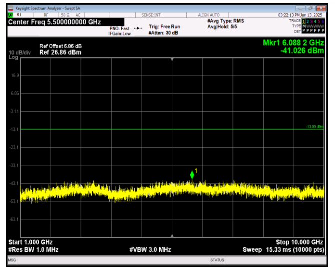
Band12-10MHz-16QAM-23060-1RB#0-Range2:1000~10000MHz
