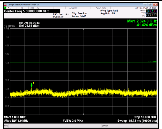
Band5-10MHz-16QAM-20525-1RB#0-Range2:1000~10000MHz
