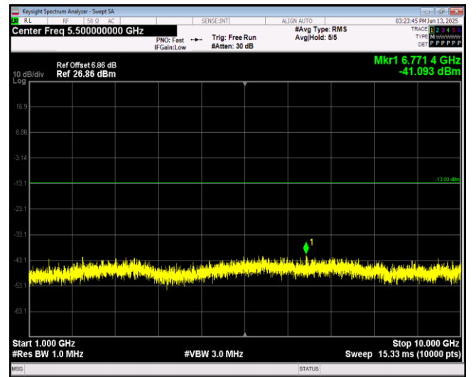
Band12-10MHz-16QAM-23060-1RB#0-Range2:1000~10000MHz
