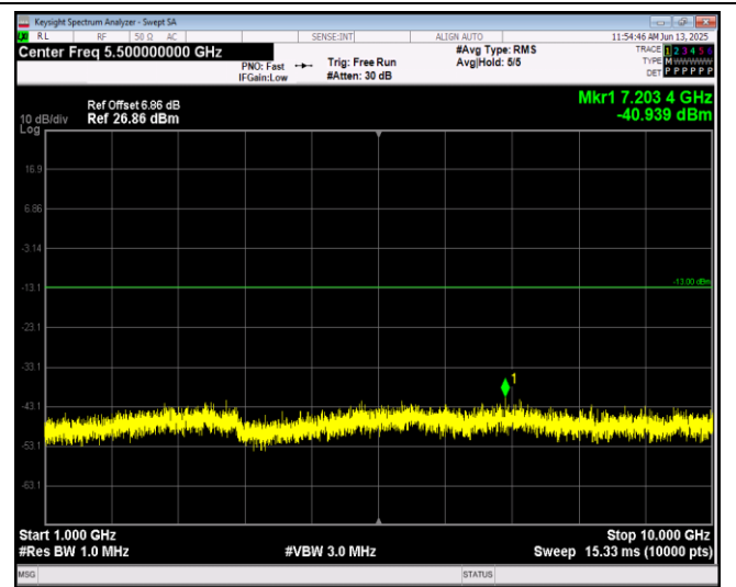
Band5-10MHz-16QAM-20450-1RB#0-Range2:1000~10000MHz
