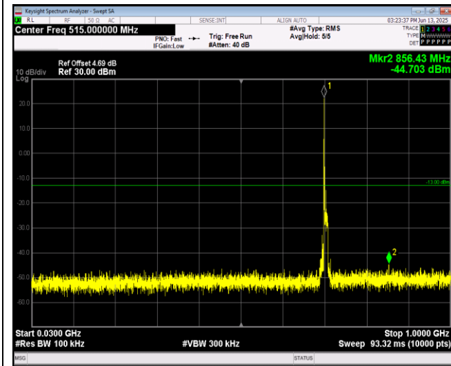
Band12-10MHz-16QAM-23060-1RB#0-Range1:30~1000MHz
