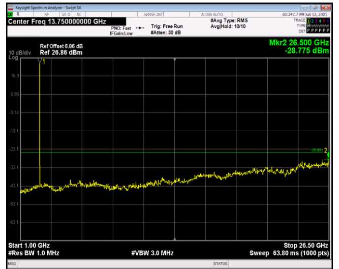
Band38-5MHz-16QAM-37775-1RB#0-Range2:1000~2 6500MHz
