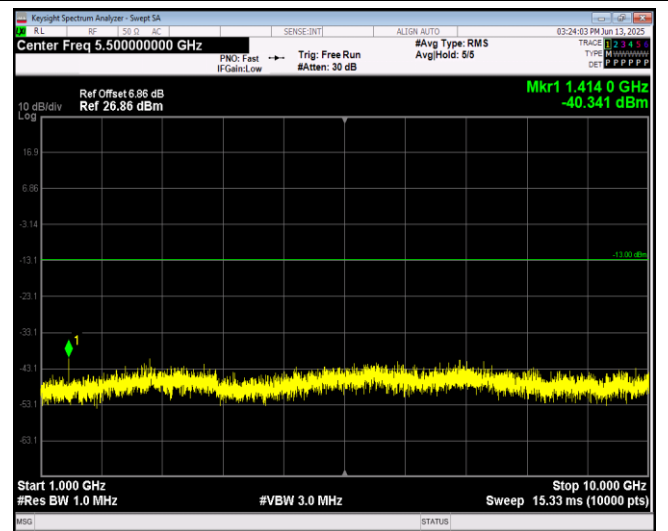
Band12-10MHz-64QAM-23060-1RB#0-Range2:1000~ 10000MHz
