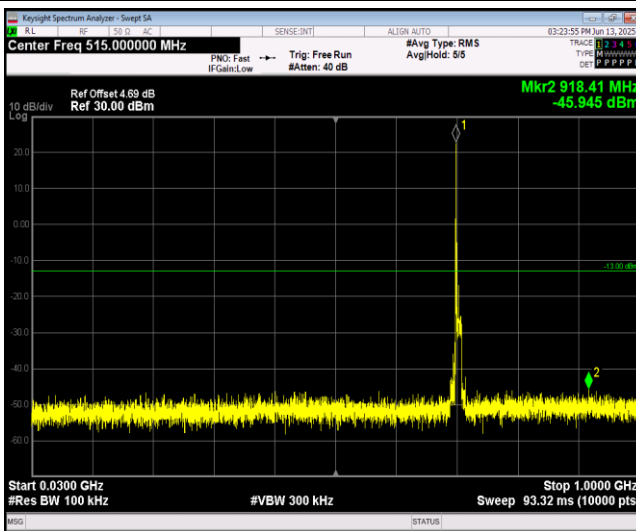
Band12-10MHz-64QAM-23060-1RB#0-Range1:30~1 000MHz
