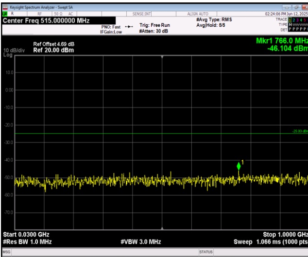
Band38-5MHz-16QAM-37775-1RB#0-Range1:30~10 00MHz
