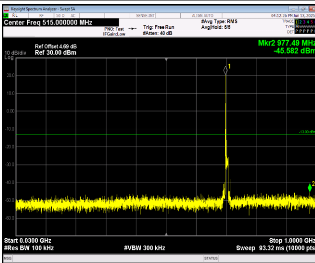
Band17-10MHz-64QAM-23800-1RB#0-Range1:30~1 000MHz
