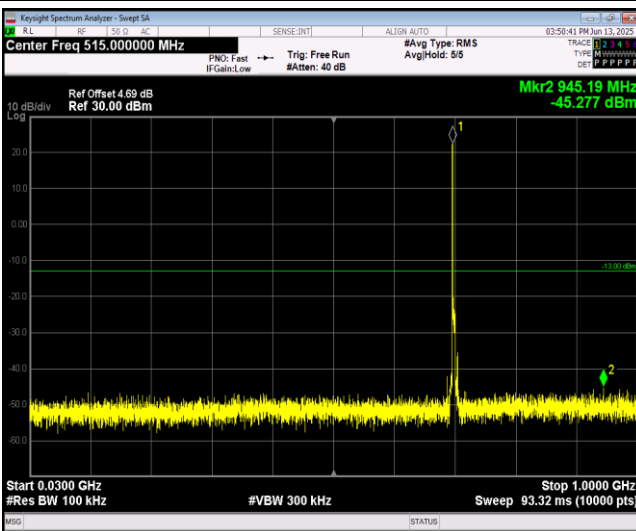
Band17-5MHz-64QAM-23790-1RB#0-Range1:30~1000MHz
