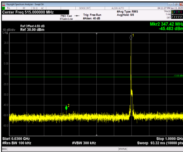
Band17-10MHz-64QAM-23790-1RB#0-Range1:30~1 000MHz
