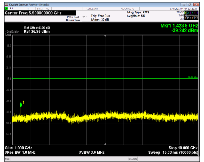
Band17-5MHz-64QAM-23755-1RB#0-Range2:1000~10000MHz
