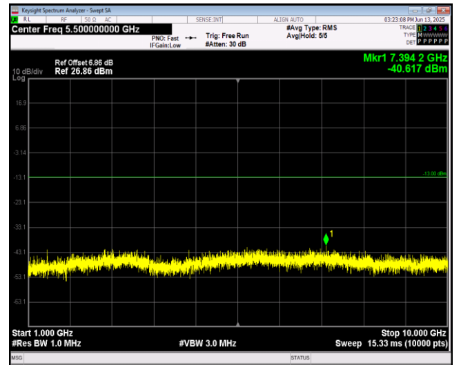
Band12-10MHz-16QAM-23130-1RB#0-Range2:1000~ 10000MHz
