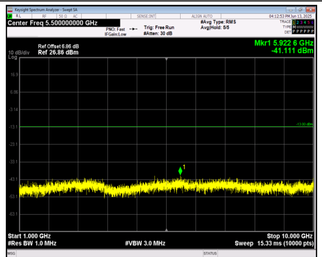
Band17-10MHz-16QAM-23780-1RB#0-Range2:1000~10000MHz
