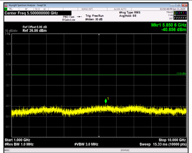
Band17-5MHz-64QAM-23790-1RB#0-Range2:1000~10000MHz
