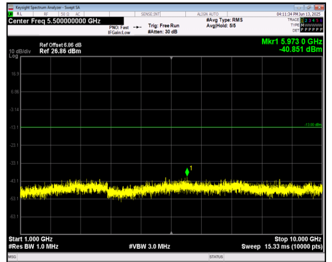
Band17-10MHz-64QAM-23790-1RB#0-Range2:1000~ 10000MHz
