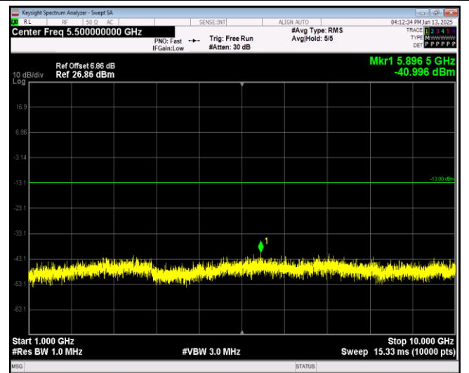
Band17-10MHz-64QAM-23800-1RB#0-Range2:1000~ 10000MHz
