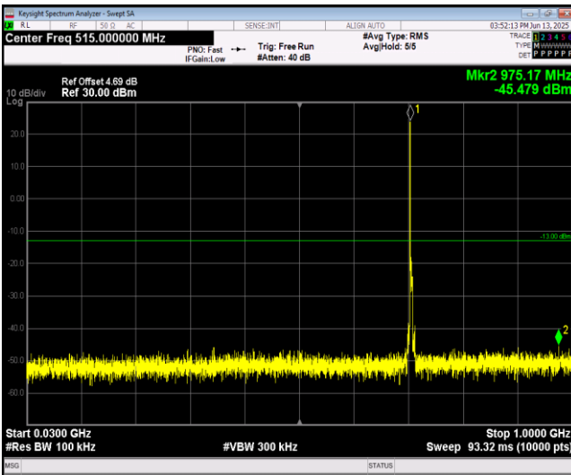
Band17-5MHz-64QAM-23755-1RB#0-Range1:30~1000MHz
