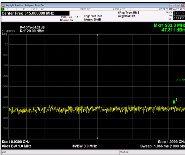
Band38-5MHz-16QAM-38000-1RB#0-Range1:30~10 00MHz
