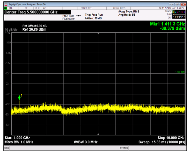
Band17-10MHz-QPSK-23800-1RB#0-Range2:1000~10000MHz
