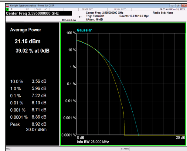
38-38-15MHz-15MHz-16QAM-16QAM-38025-38175-75RB #0-75RB#0-PASS
