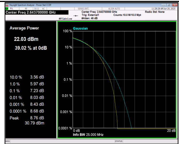
41(2555-2655)-41(2555-2655)-15MHz-15MHz-16QAM-16 QAM-40315-40465-75RB#0-75RB#0-PASS
