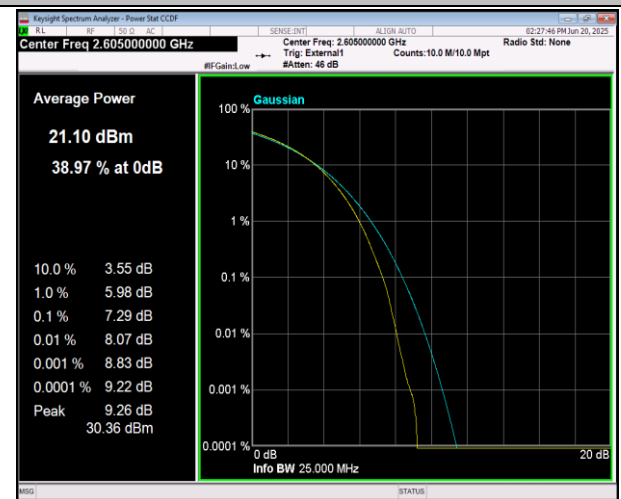
41(2555-2655)-41(2555-2655)-15MHz-15MHz-16QAM-16 QAM-41015-41165-75RB#0-75RB#0-PASS
