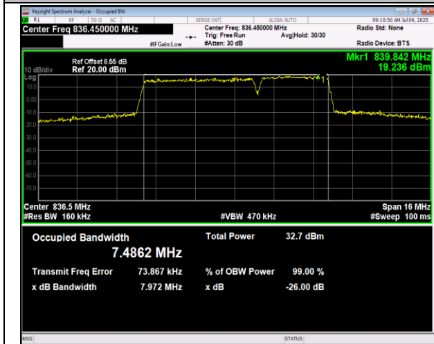
5-5-5MHz-3MHz-QPSK-QPSK-20595-20634-25RB#0-15 RB#0-PASS
