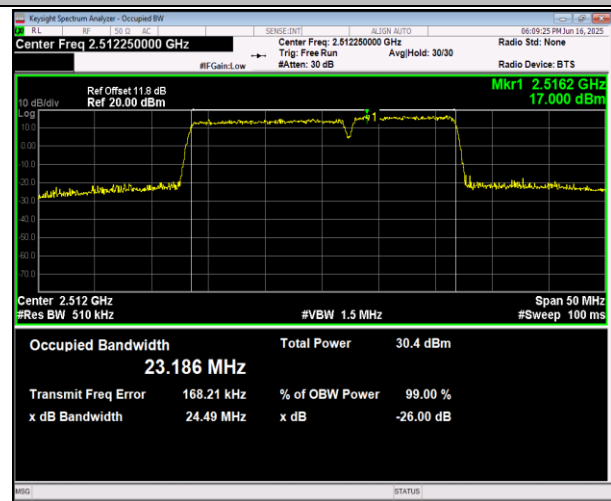
7-7-15MHz-10MHz-16QAM-16QAM-21051-21171-75RB#0-5 50RB#0-PASS
