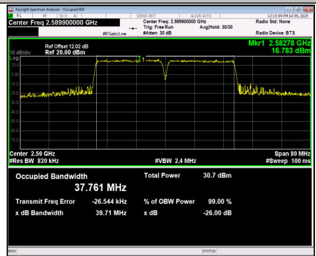
38-38-20MHz-20MHz-16QAM-16QAM-37901-38099-100RB B#0-100RB#0-PASS
