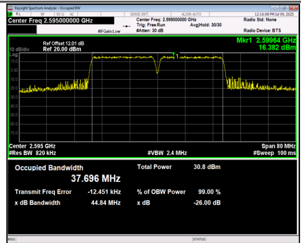
38-38-20MHz-20MHz-16QAM-16QAM-37952-38150-100RB B#0-100RB#0-PASS
