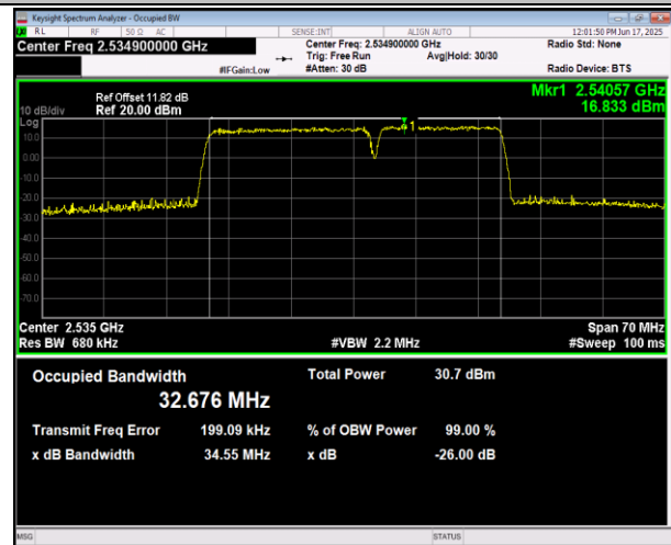
7-7-20MHz-15MHz-16QAM-16QAM-21201-21372-100RB#0-75RB#0-PASS
