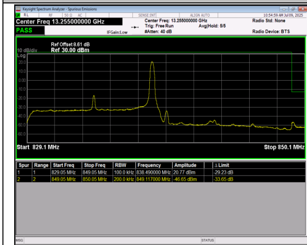
5-5-10MHz-10MHz-16QAM@16QAM-16QAM@16QAM-20501-20600-1RB#0@50RB#0-0RB#0@50RB#0-PASS
