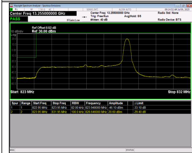
5-5-5MHz-3MHz-16QAM@16QAM-16QAM@16QAM-204 25-20464-1RB#0@25RB#0-0RB#0@15RB#0-PASS
