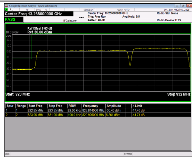
5-5-5MHz-3MHz-16QAM@16QAM-16QAM@16QAM-2042 5-20464-1RB#0@25RB#0-1RB#15@15RB#0-PASS
