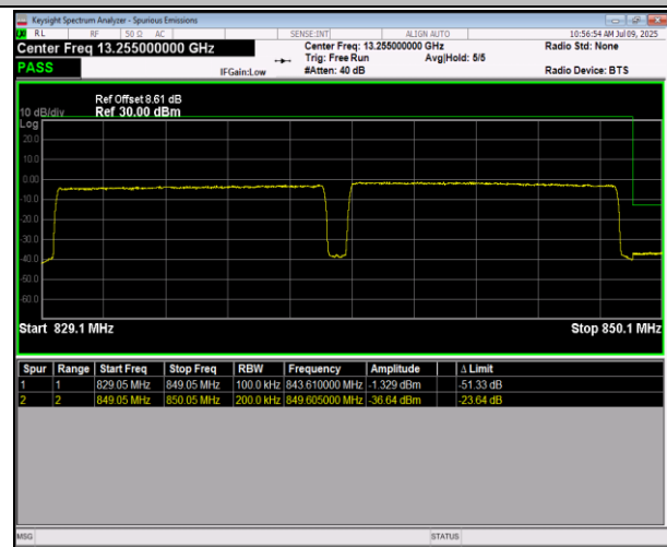
5-5-10MHz-10MHz-16QAM@16QAM-16QAM@16QAM-20501-20600-1RB#0@50RB#0-1RB#49@50RB#0-PASS
