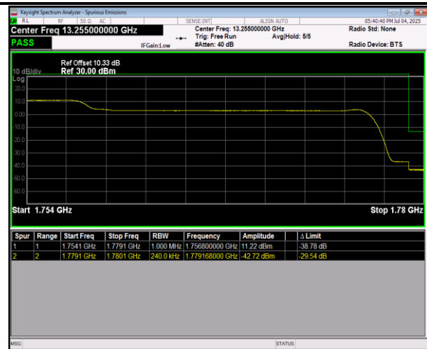
66-66-5MHz-20MHz-16QAM@16QAM-16QAM@16QAM-132428-132572-1RB#0@25RB#0-1RB#99@100RB#0-PAS S
