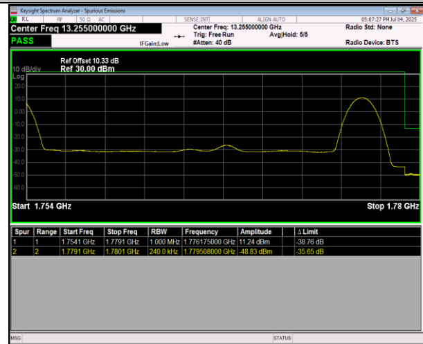
66-66-5MHz-20MHz-16QAM@16QAM-16QAM@16QAM-132428-132572-25RB#0@25RB#0-100RB#0@100RB#0-PA SS
