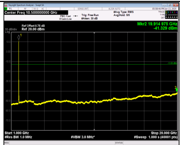
2-2-5MHz-20MHz-16QAM-16QAM-18633-18750-1RB#24-0 RB#0-1000~20000MHz-PASS
