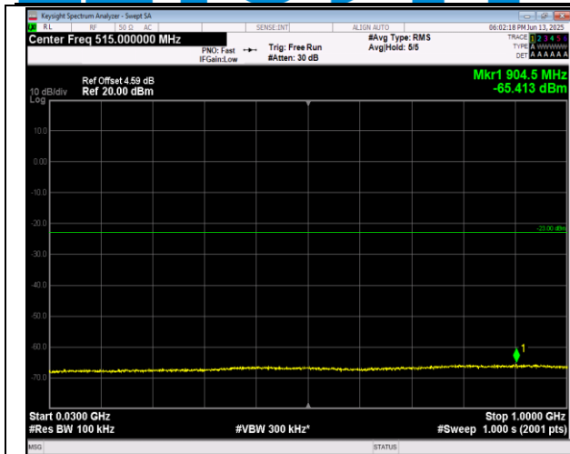
2-2-5MHz-20MHz-16QAM-16QAM-18808-18925-25RB#0 -100RB#0-30~1000MHz-PASS
