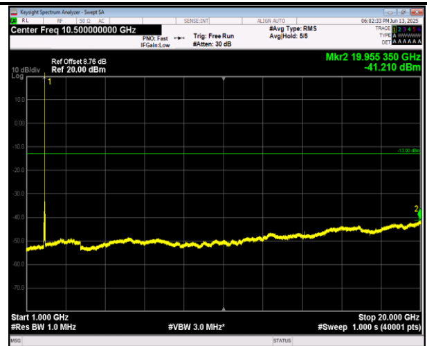
2-2-5MHz-20MHz-16QAM-16QAM-18808-18925-25RB#0-1 00RB#0-1000~20000MHz-PASS
