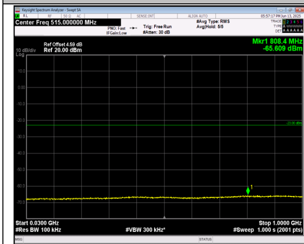
2-2-5MHz-20MHz-16QAM-16QAM-18633-18750-25RB#0 -100RB#0-30~1000MHz-PASS
