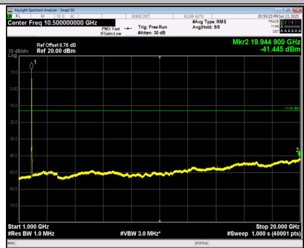
2-2-5MHz-20MHz-16QAM-16QAM-18633-18750-1RB#0-OR B#0-1000~20000MHz-PASS
