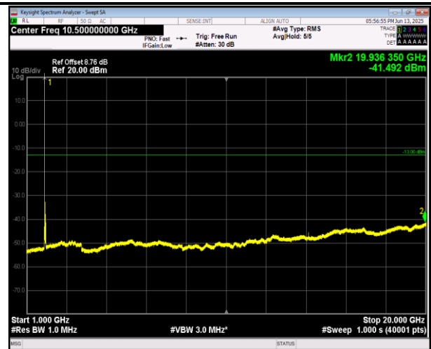
2-2-5MHz-20MHz-QPSK-QPSK-18633-18750-25RB#0-100 RB#0-1000~20000MHz-PASS
