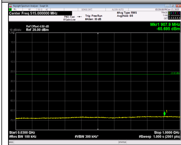
2-2-5MHz-20MHz-16QAM-16QAM-18633-18750-1RB#0- ORB#0-30~1000MHz-PASS
