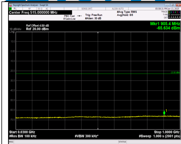
2-2-5MHz-20MHz-16QAM-16QAM-18633-18750-1RB#24 -0RB#0-30~1000MHz-PASS
