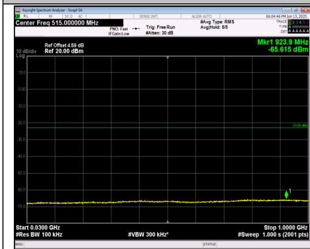
2-2-5MHz-20MHz-QPSK-QPSK-18983-19100-1RB#0-0R B#0-30~1000MHz-PASS
