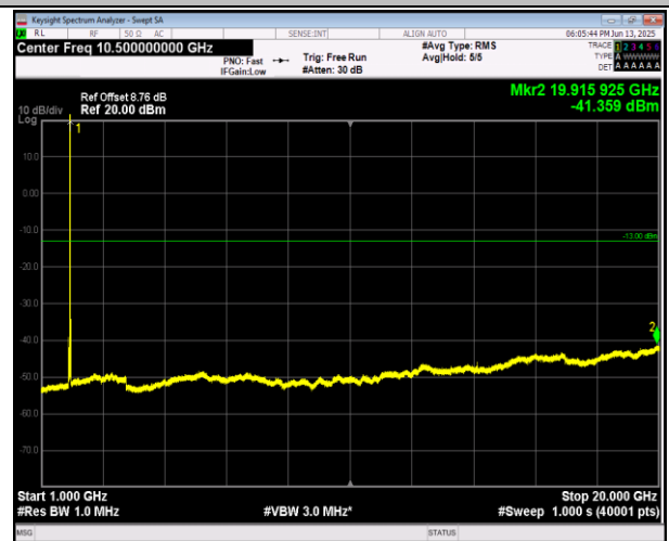
2-2-5MHz-20MHz-QPSK-QPSK-18983-19100-1RB#0-1RB# 99-1000~20000MHz-PASS
