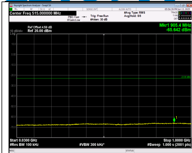
2-2-5MHz-20MHz-QPSK-QPSK-18633-18750-25RB#0-10 ORB#0-30~1000MHz-PASS
