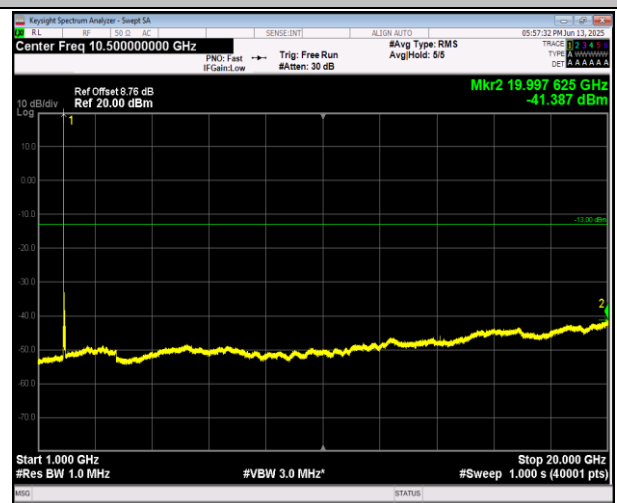
2-2-5MHz-20MHz-16QAM-16QAM-18633-18750-25RB#0-1 00RB#0-1000~20000MHz-PASS
