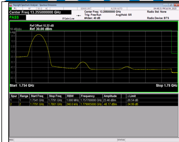
66-66-5MHz-20MHz-16QAM@16QAM-16QAM@16QAM-132428-132572-1RB#0@25RB#0-0RB#0@100RB#0-PA SS
