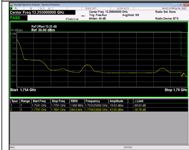
66-66-5MHz-20MHz-16QAM@16QAM-16QAM@16QAM-132428-132572-1RB#24@25RB#0-0RB#0@100RB#0-PA SS
