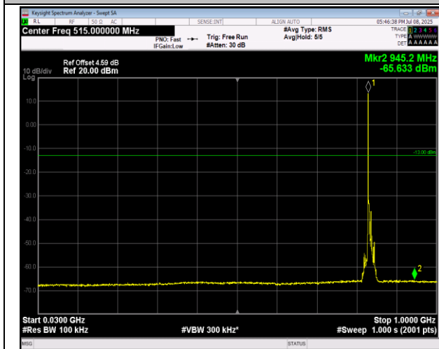
5-5-3MHz-5MHz-16QAM-16QAM-20501-20540-1RB#14-0 ORB#0-30~1000MHz-PASS
