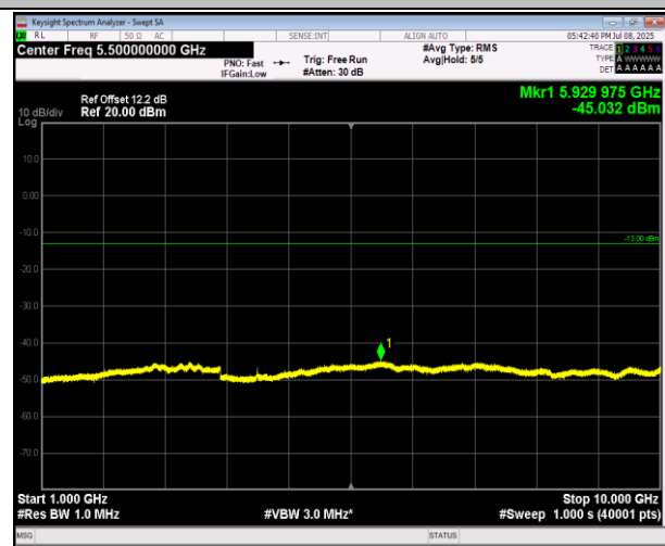
5-5-3MHz-5MHz-16QAM-16QAM-20416-20455-1RB#0-0R B#0-1000~10000MHz-PASS
