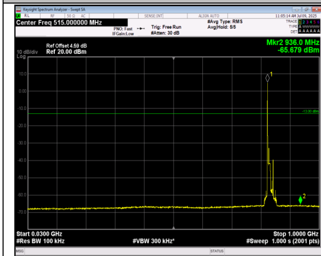
5-5-10MHz-10MHz-QPSK-QPSK-20476-20575-1RB#49-0 RB#0-30~1000MHz-PASS
