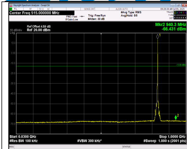
5-5-5MHz-3MHz-16QAM-16QAM-20510-20549-25RB#0-15RB#0-30~1000MHz-PASS
