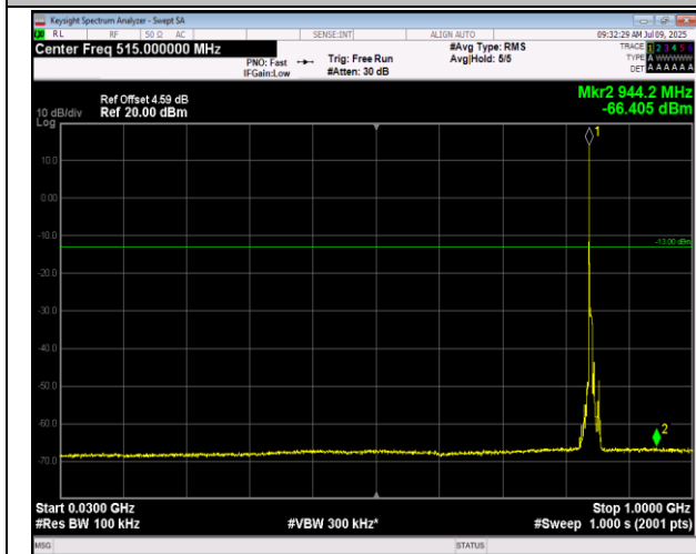
5-5-5MHz-3MHz-QPSK-QPSK-20595-20634-1RB#0-1RB#15-30~1000MHz-PASS
