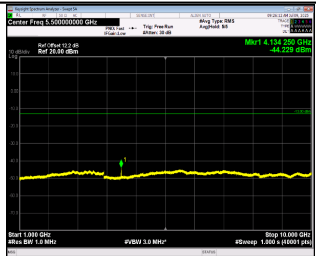
5-5-5MHz-3MHz-16QAM-16QAM-20425-20464-1RB#24-0RB#0-1000~10000MHz-PASS
