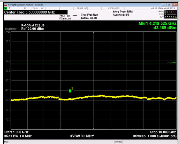
5-5-3MHz-5MHz-16QAM-16QAM-20586-20625-15RB#0-25 RB#0-1000~10000MHz-PASS
