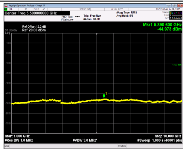
5-5-5MHz-3MHz-QPSK-QPSK-20595-20634-1RB#0-0RB#0-1000~10000MHz-PASS
