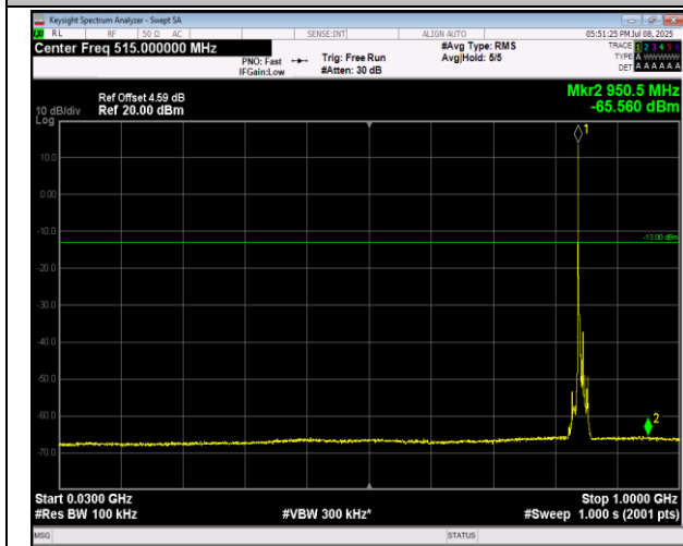
5-5-3MHz-5MHz-16QAM-16QAM-20586-20625-1RB#14- 0RB#0-30~1000MHz-PASS
