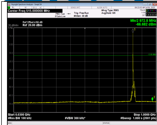
5-5-5MHz-3MHz-16QAM-16QAM-20595-20634-1RB#0-1 RB#15-30~1000MHz-PASS
