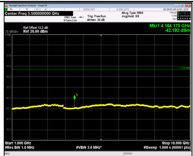
5-5-5MHz-3MHz-QPSK-QPSK-20510-20549-1RB#0-1RB#1 5-1000~10000MHz-PASS
