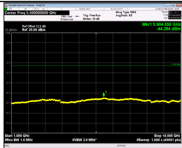
5-5-10MHz-10MHz-16QAM-16QAM-20476-20575-1RB#0-0 RB#0-1000~10000MHz-PASS
