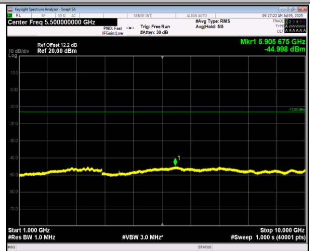
5-5-5MHz-3MHz-QPSK-QPSK-20510-20549-1RB#0-0RB#0-1000~10000MHz-PASS
