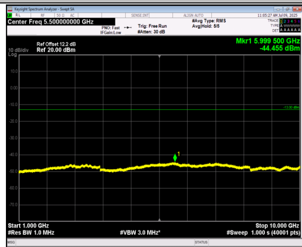
5-5-10MHz-10MHz-QPSK-QPSK-20476-20575-1RB#49-0R B#0-1000~10000MHz-PASS
