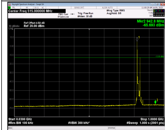
5-5-10MHz-10MHz-QPSK-QPSK-20450-20549-1RB#49-0 RB#0-30~1000MHz-PASS
