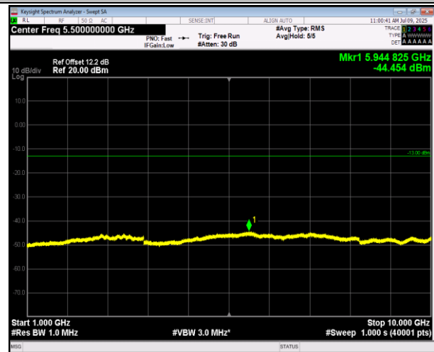
5-5-10MHz-10MHz-QPSK-QPSK-20450-20549-1RB#49-0R B#0-1000~10000MHz-PASS
