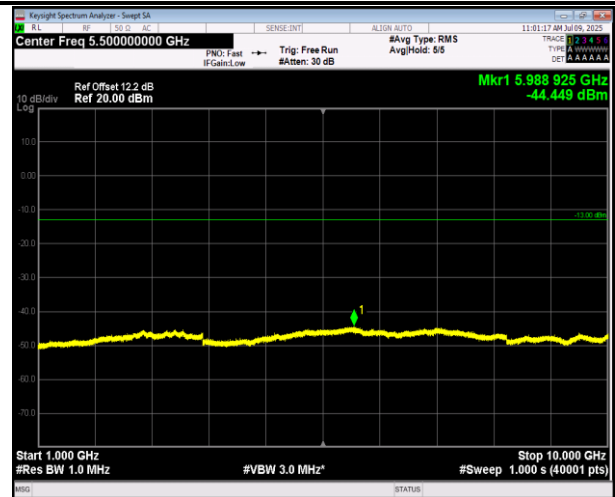
5-5-10MHz-10MHz-16QAM-16QAM-20450-20549-1RB#49- 0RB#0-1000~10000MHz-PASS
