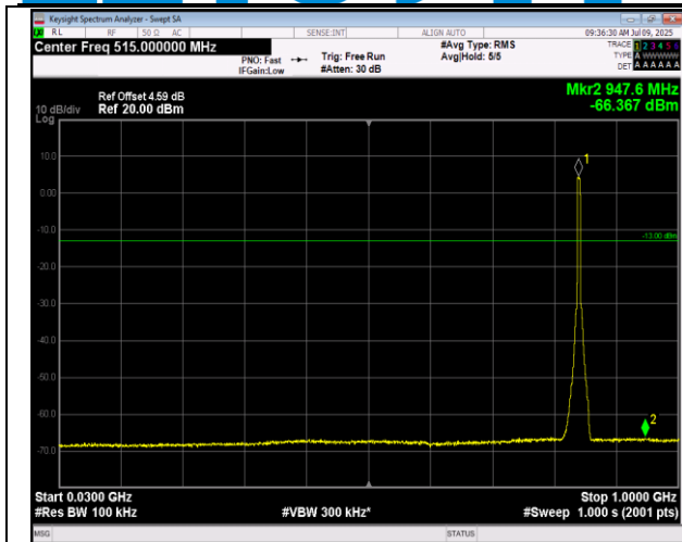
5-5-10MHz-10MHz-QPSK-QPSK-20450-20549-1RB#0-0 RB#0-30~1000MHz-PASS
