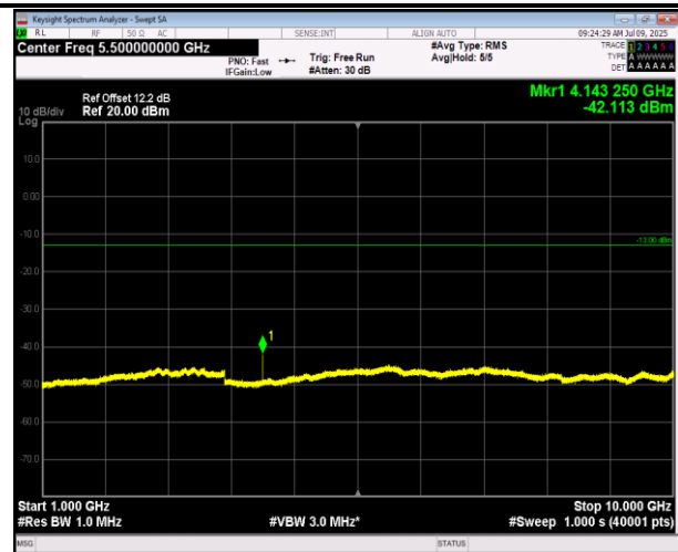
5-5-5MHz-3MHz-QPSK-QPSK-20425-20464-25RB#0-15RB #0-1000~10000MHz-PASS
