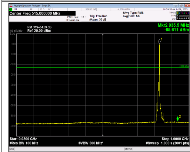
5-5-10MHz-10MHz-16QAM-16QAM-20450-20549-50RB#- 0-50RB#0-30~1000MHz-PASS
