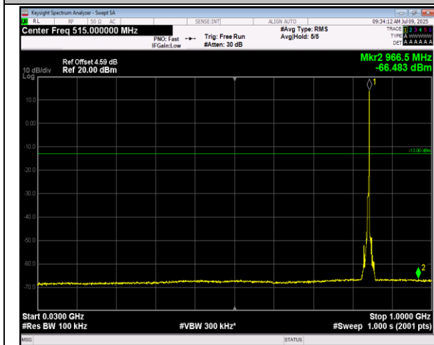
5-5-5MHz-3MHz-16QAM-16QAM-20595-20634-25RB#0- 15RB#0-30~1000MHz-PASS
