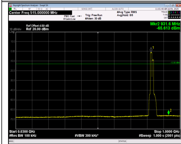
5-5-10MHz-10MHz-16QAM-16QAM-20450-20549-1RB#0 -ORB#0-30~1000MHz-PASS
