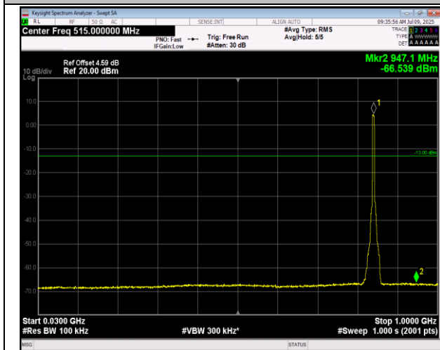
5-5-5MHz-3MHz-16QAM-16QAM-20595-20634-1RB#0-0 RB#0-30~1000MHz-PASS
