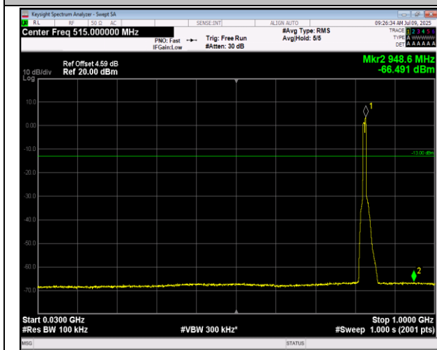
5-5-5MHz-3MHz-16QAM-16QAM-20425-20464-1RB#0-0 RB#0-30~1000MHz-PASS
