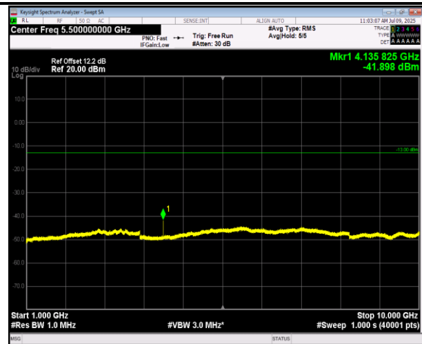
5-5-10MHz-10MHz-QPSK-QPSK-20476-20575-1RB#0-1RB #49-1000~10000MHz-PASS
