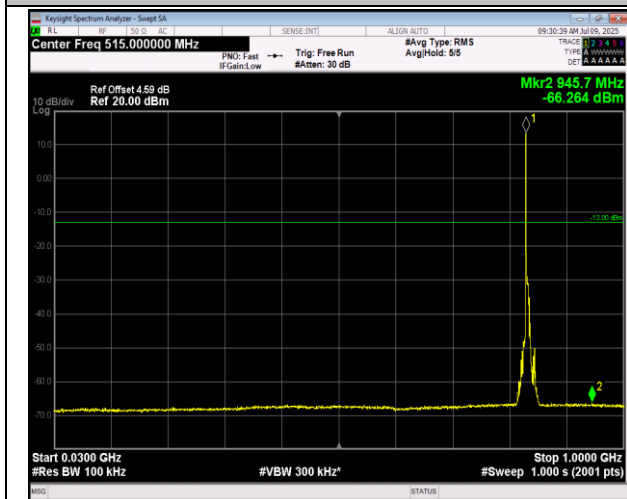
5-5-5MHz-3MHz-16QAM-16QAM-20510-20549-1RB#24- ORB#0-30~1000MHz-PASS
