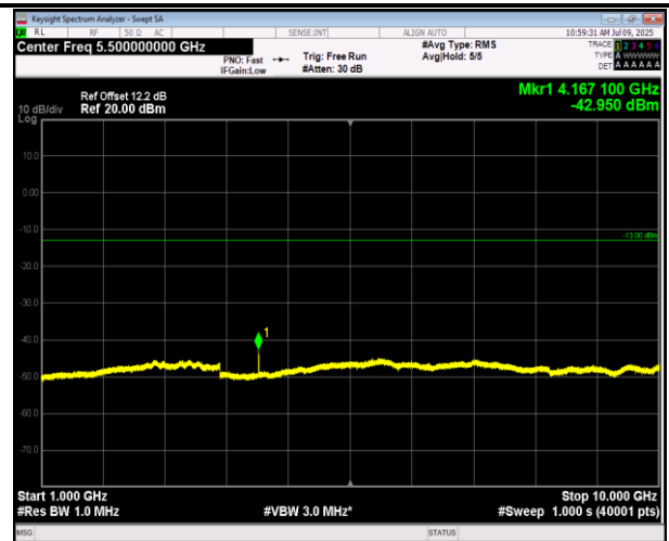
5-5-10MHz-10MHz-QPSK-QPSK-20450-20549-50RB#0-50 RB#0-1000~10000MHz-PASS
