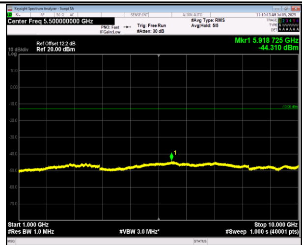
5-5-10MHz-10MHz-QPSK-QPSK-20501-20600-1RB#49-0R B#0-1000~10000MHz-PASS
