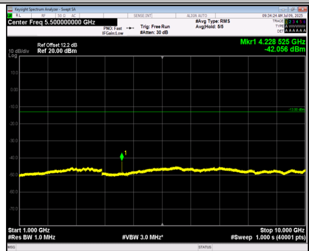
5-5-5MHz-3MHz-16QAM-16QAM-20595-20634-25RB#0-15 RB#0-1000~10000MHz-PASS
