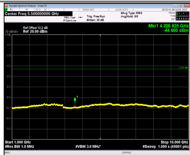
5-5-5MHz-3MHz-QPSK-QPSK-20595-20634-1RB#0-1RB#15-1000~10000MHz-PASS
