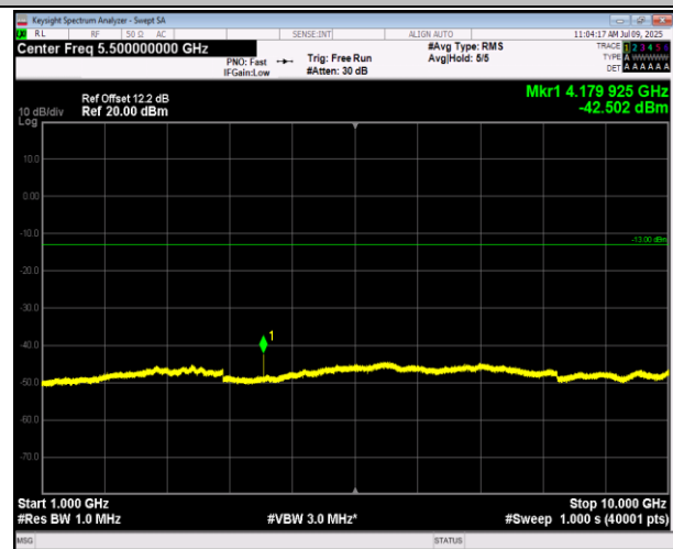
5-5-10MHz-10MHz-QPSK-QPSK-20476-20575-50RB#0-50 RB#0-1000~10000MHz-PASS
