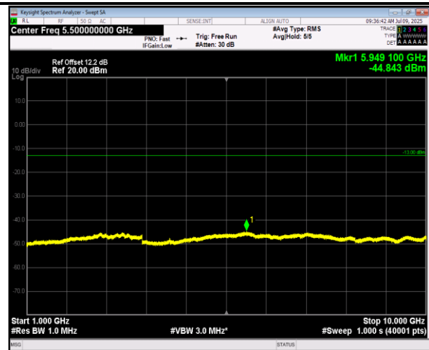
5-5-10MHz-10MHz-QPSK-QPSK-20450-20549-1RB#0-0RB #0-1000~10000MHz-PASS
