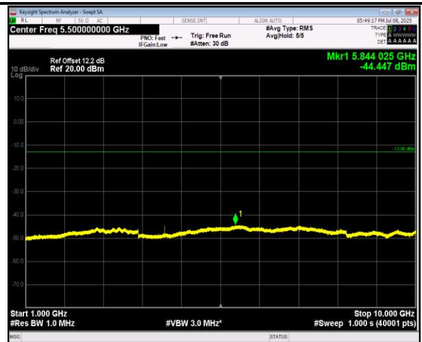
5-5-3MHz-5MHz-16QAM-16QAM-20586-20625-1RB#0-1R B#24-1000~10000MHz-PASS
