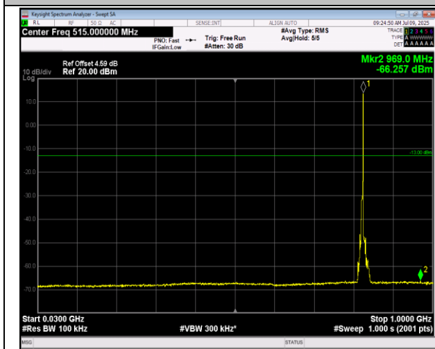
5-5-5MHz-3MHz-16QAM-16QAM-20425-20464-25RB#0-15RB#0-30~1000MHz-PASS
