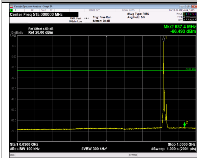
5-5-5MHz-3MHz-QPSK-QPSK-20425-20464-1RB#0-1RB #15-30~1000MHz-PASS
