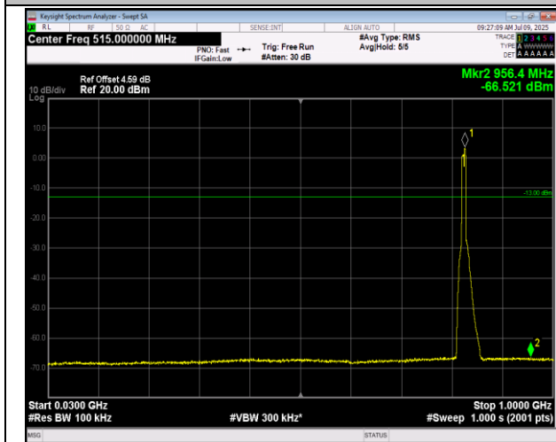
5-5-5MHz-3MHz-QPSK-QPSK-20510-20549-1RB#0-0RB#0-30~1000MHz-PASS
