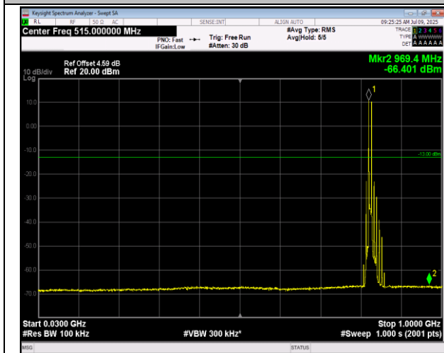
5-5-5MHz-3MHz-QPSK-QPSK-20425-20464-1RB#24-0R B#0-30~1000MHz-PASS
