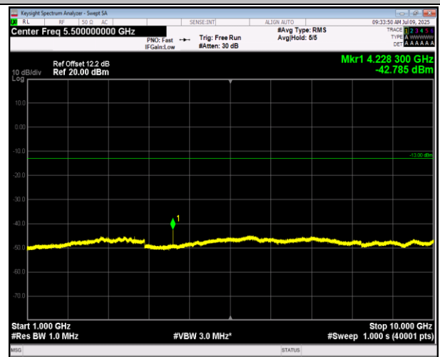
5-5-5MHz-3MHz-QPSK-QPSK-20595-20634-25RB#0-15RB #0-1000~10000MHz-PASS
