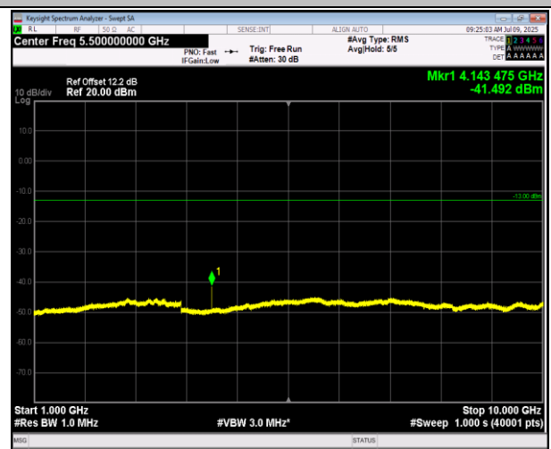
5-5-5MHz-3MHz-16QAM-16QAM-20425-20464-25RB#0-15RB#0-1000~10000MHz-PASS
