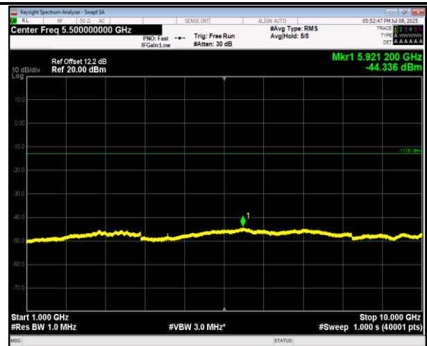
5-5-5MHz-3MHz-QPSK-QPSK-20425-20464-1RB#0-0RB#0 -1000~10000MHz-PASS
