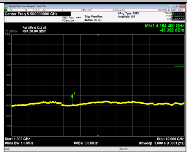
5-5-5MHz-3MHz-16QAM-16QAM-20510-20549-1RB#0-1R B#15-1000~10000MHz-PASS
