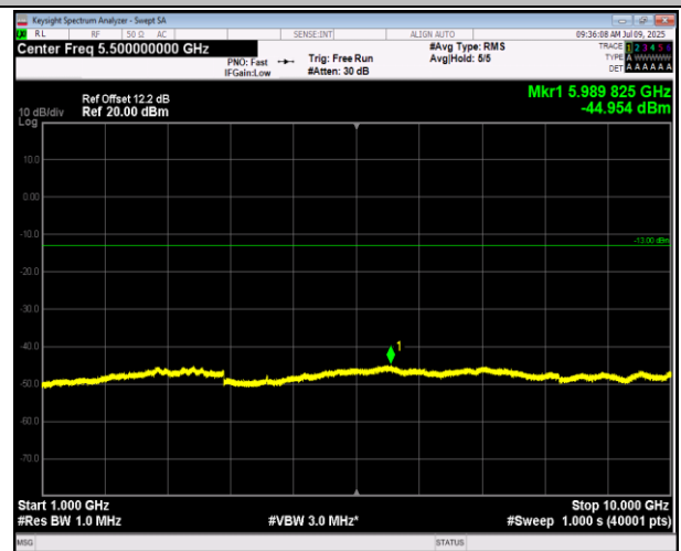
5-5-5MHz-3MHz-16QAM-16QAM-20595-20634-1RB#0-0R B#0-1000~10000MHz-PASS
