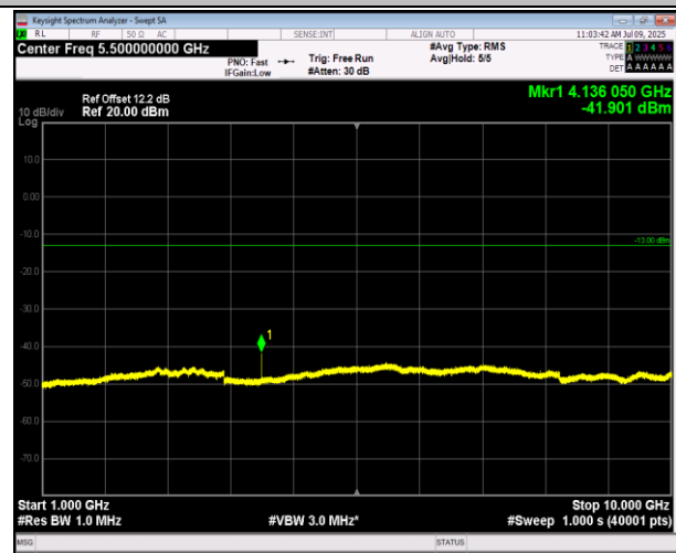
5-5-10MHz-10MHz-16QAM-16QAM-20476-20575-1RB#0-1 RB#49-1000~10000MHz-PASS
