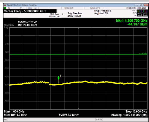
5-5-5MHz-3MHz-16QAM-16QAM-20595-20634-1RB#24-0R B#0-1000~10000MHz-PASS
