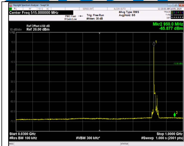
5-5-10MHz-10MHz-QPSK-QPSK-20501-20600-1RB#49-0 RB#0-30~1000MHz-PASS
