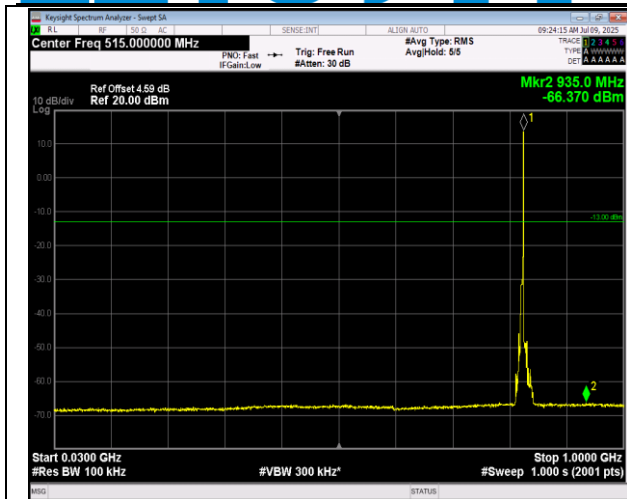
5-5-5MHz-3MHz-QPSK-QPSK-20425-20464-25RB#0-15 RB#0-30~1000MHz-PASS
