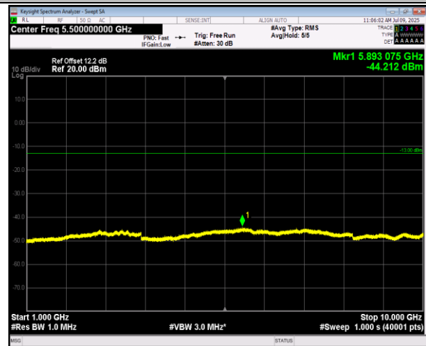
5-5-10MHz-10MHz-16QAM-16QAM-20476-20575-1RB#49- 0RB#0-1000~10000MHz-PASS
