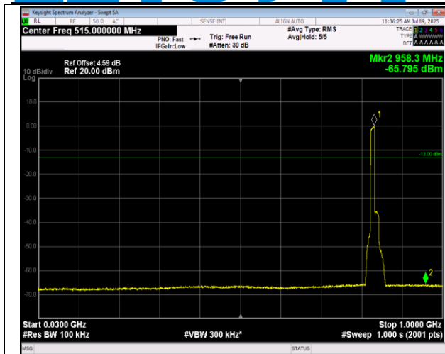
5-5-10MHz-10MHz-16QAM-16QAM-20476-20575-1RB#0 -0RB#0-30~1000MHz-PASS
