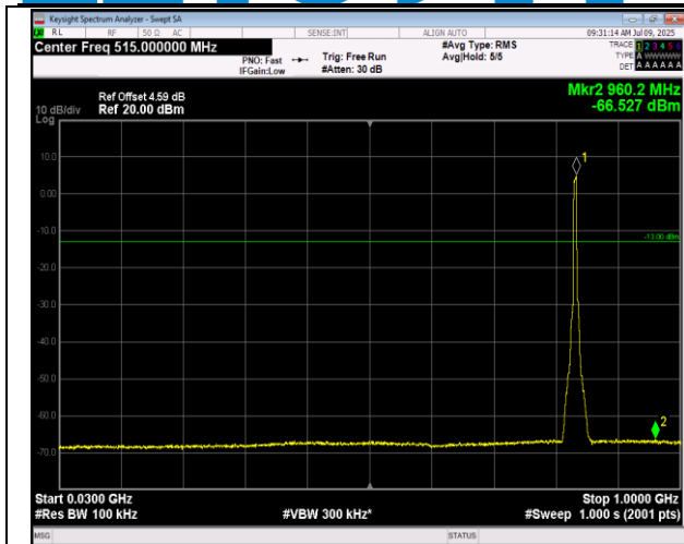
5-5-5MHz-3MHz-16QAM-16QAM-20510-20549-1RB#0-0 RB#0-30~1000MHz-PASS
