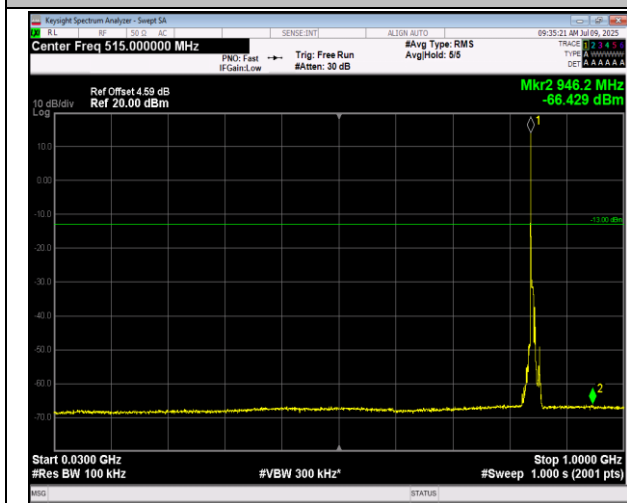
5-5-5MHz-3MHz-16QAM-16QAM-20595-20634-1RB#24- 0RB#0-30~1000MHz-PASS
