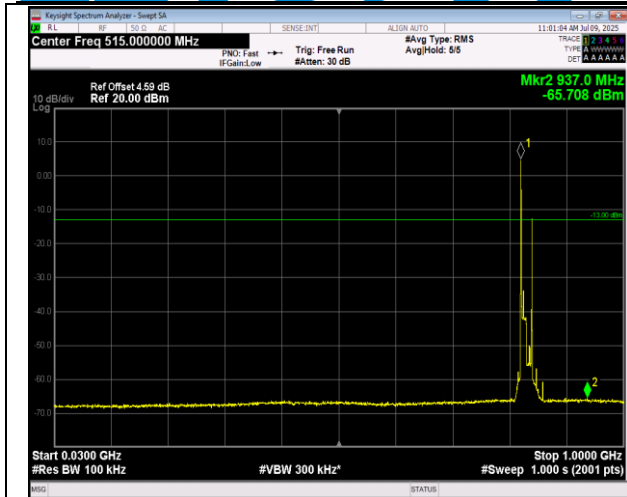
5-5-10MHz-10MHz-16QAM-16QAM-20450-20549-1RB#4 9-0RB#0-30~1000MHz-PASS
