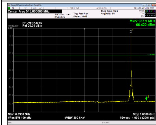
5-5-5MHz-3MHz-16QAM-16QAM-20510-20549-1RB#0-1 RB#15-30~1000MHz-PASS
