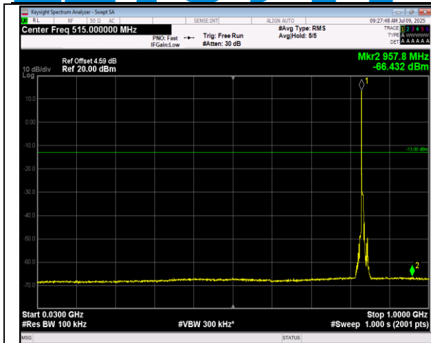
5-5-5MHz-3MHz-QPSK-QPSK-20510-20549-1RB#0-1RB #15-30~1000MHz-PASS
