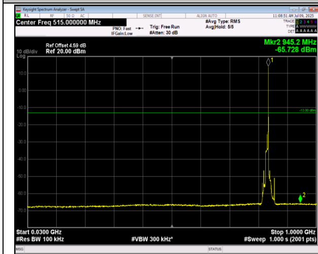
5-5-10MHz-10MHz-QPSK-QPSK-20501-20600-50RB#0-5 ORB#0-30~1000MHz-PASS
