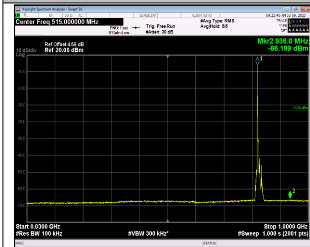
5-5-5MHz-3MHz-16QAM-16QAM-20425-20464-1RB#0-1 RB#15-30~1000MHz-PASS
