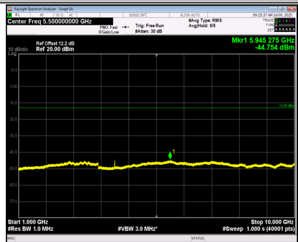
5-5-5MHz-3MHz-QPSK-QPSK-20425-20464-1RB#24-0RB# 0-1000~10000MHz-PASS
