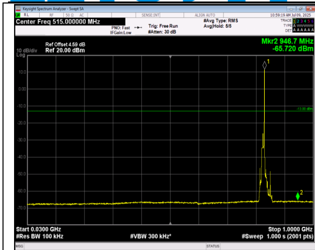
5-5-10MHz-10MHz-QPSK-QPSK-20450-20549-50RB#0-5 ORB#0-30~1000MHz-PASS
