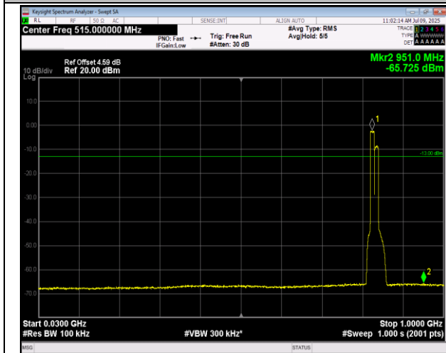
5-5-10MHz-10MHz-QPSK-QPSK-20476-20575-1RB#0-0 RB#0-30~1000MHz-PASS
