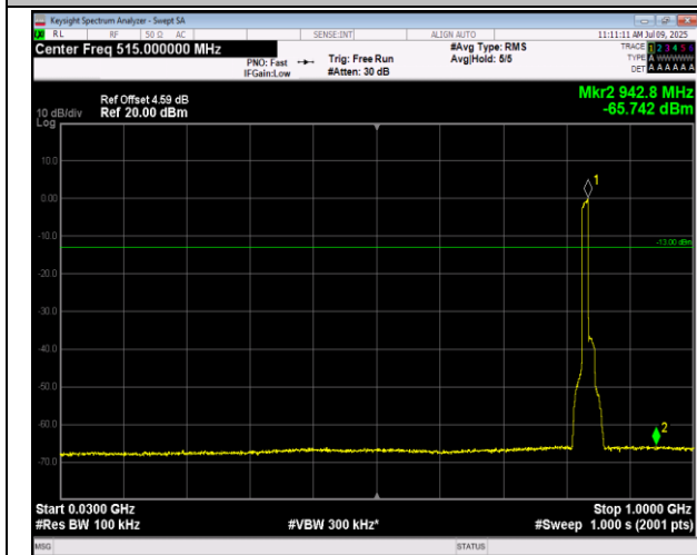
5-5-10MHz-10MHz-16QAM-16QAM-20501-20600-1RB#0-0RB#0-30~1000MHz-PASS
