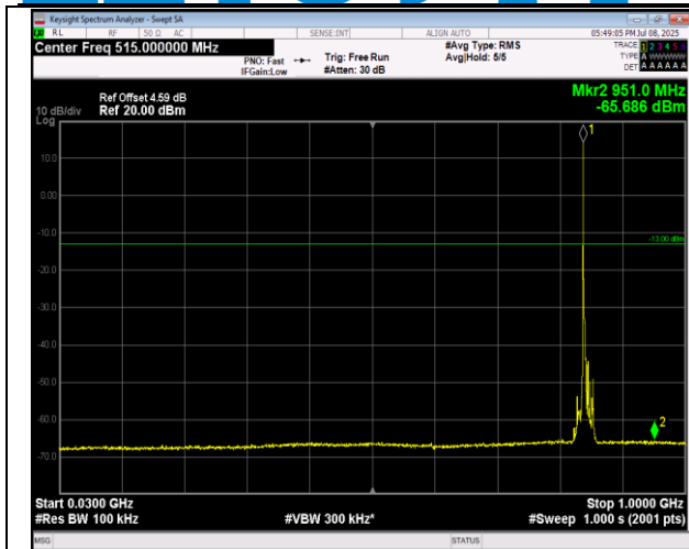
5-5-3MHz-5MHz-16QAM-16QAM-20586-20625-1RB#0-1 RB#24-30~1000MHz-PASS
