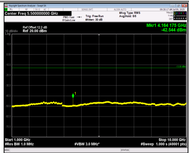
5-5-5MHz-3MHz-QPSK-QPSK-20510-20549-1RB#24-0RB# 0-1000~10000MHz-PASS
