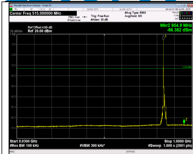
5-5-5MHz-3MHz-QPSK-QPSK-20595-20634-1RB#24-0R B#0-30~1000MHz-PASS
