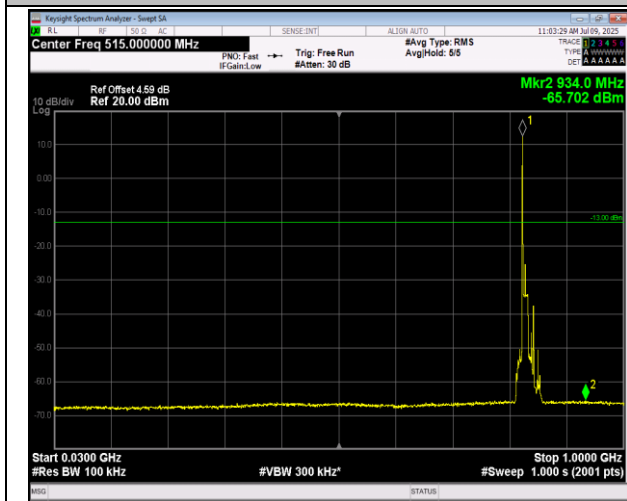
5-5-10MHz-10MHz-16QAM-16QAM-20476-20575-1RB#0 -1RB#49-30~1000MHz-PASS
