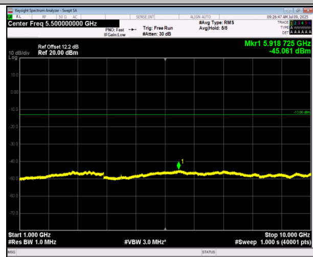
5-5-5MHz-3MHz-16QAM-16QAM-20425-20464-1RB#0-0R B#0-1000~10000MHz-PASS
