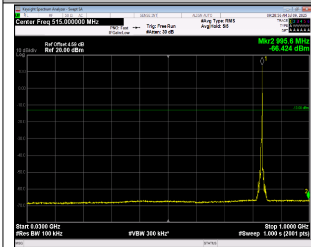
5-5-5MHz-3MHz-QPSK-QPSK-20510-20549-25RB#0-15 RB#0-30~1000MHz-PASS
