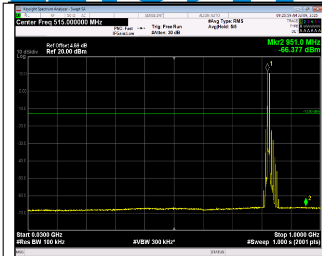
5-5-5MHz-3MHz-16QAM-16QAM-20425-20464-1RB#24-0RB#0-30~1000MHz-PASS
