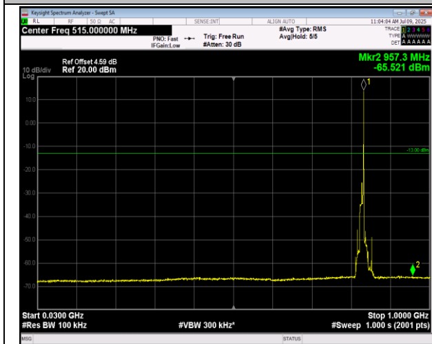
5-5-10MHz-10MHz-QPSK-QPSK-20476-20575-50RB#0-5 ORB#0-30~1000MHz-PASS
