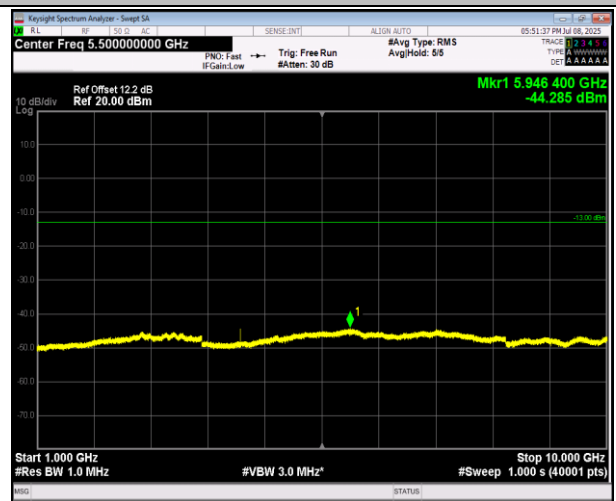
5-5-3MHz-5MHz-16QAM-16QAM-20586-20625-1RB#14-0R B#0-1000~10000MHz-PASS
