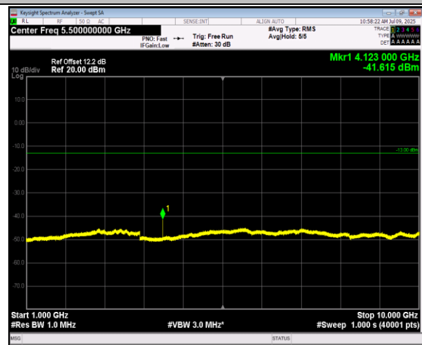
5-5-10MHz-10MHz-QPSK-QPSK-20450-20549-1RB#0-1RB #49-1000~10000MHz-PASS
