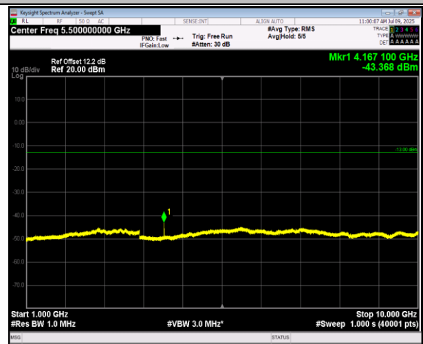
5-5-10MHz-10MHz-16QAM-16QAM-20450-20549-50RB#0- 50RB#0-1000~10000MHz-PASS
