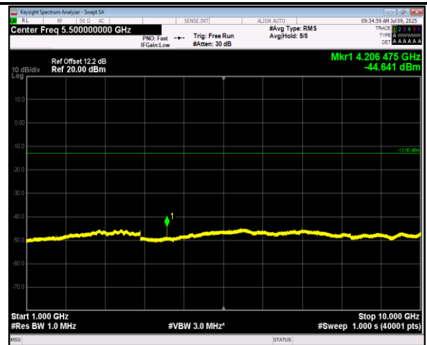
5-5-5MHz-3MHz-QPSK-QPSK-20595-20634-1RB#24-0RB# 0-1000~10000MHz-PASS
