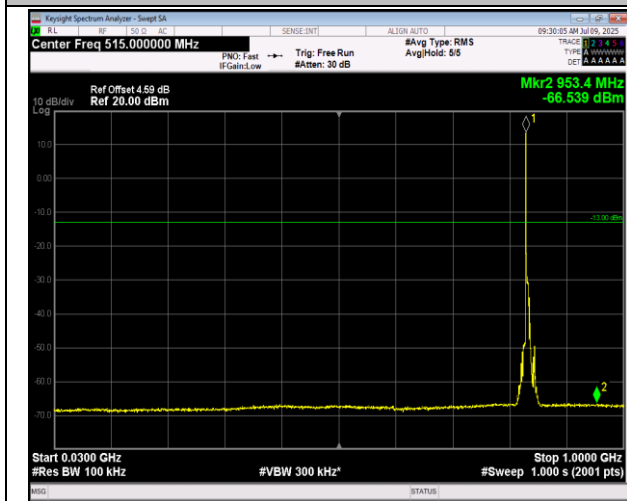
5-5-5MHz-3MHz-QPSK-QPSK-20510-20549-1RB#24-0R B#0-30~1000MHz-PASS
