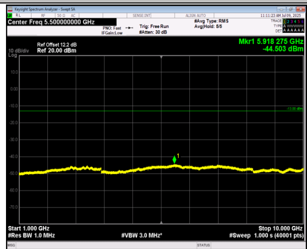
5-5-10MHz-10MHz-16QAM-16QAM-20501-20600-1RB#0-0RB#0-1000~10000MHz-PASS
