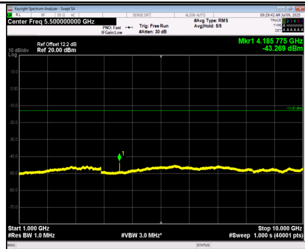
5-5-5MHz-3MHz-16QAM-16QAM-20510-20549-25RB#0-15RB#0-1000~10000MHz-PASS
