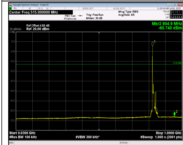
5-5-10MHz-10MHz-16QAM-16QAM-20476-20575-1RB#4 9-0RB#0-30~1000MHz-PASS
