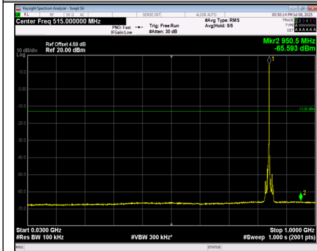
5-5-3MHz-5MHz-16QAM-16QAM-20586-20625-15RB#0- 25RB#0-30~1000MHz-PASS
