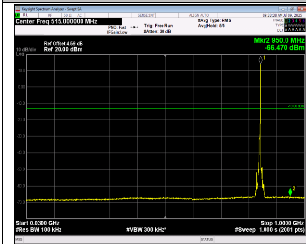
5-5-5MHz-3MHz-QPSK-QPSK-20595-20634-25RB#0-15 RB#0-30~1000MHz-PASS
