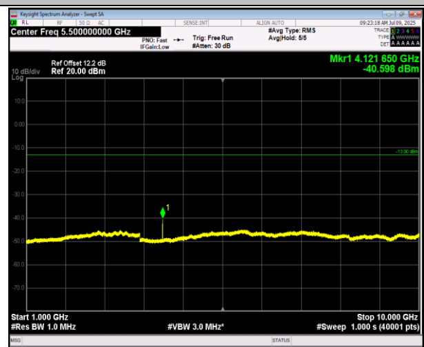
5-5-5MHz-3MHz-QPSK-QPSK-20425-20464-1RB#0-1RB#1 5-1000~10000MHz-PASS
