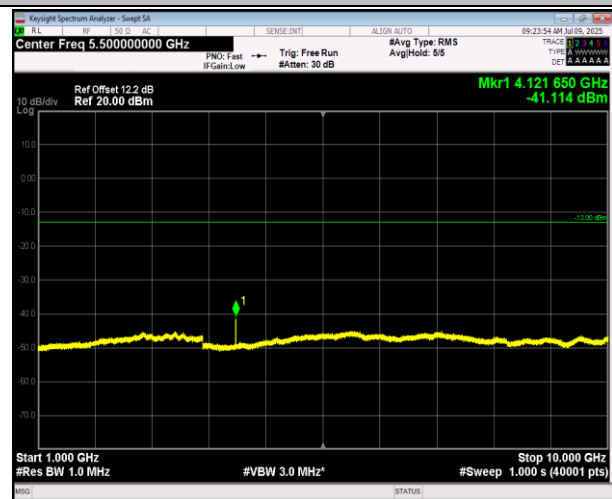
5-5-5MHz-3MHz-16QAM-16QAM-20425-20464-1RB#0-1R B#15-1000~10000MHz-PASS
