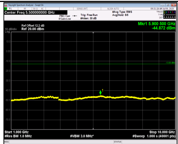
5-5-5MHz-3MHz-16QAM-16QAM-20510-20549-1RB#0-0R B#0-1000~10000MHz-PASS
