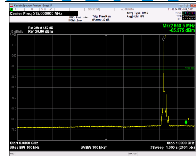
5-5-10MHz-10MHz-QPSK-QPSK-20476-20575-1RB#0-1 RB#49-30~1000MHz-PASS
