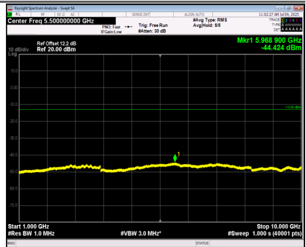
5-5-10MHz-10MHz-QPSK-QPSK-20476-20575-1RB#0-0RB #0-1000~10000MHz-PASS
