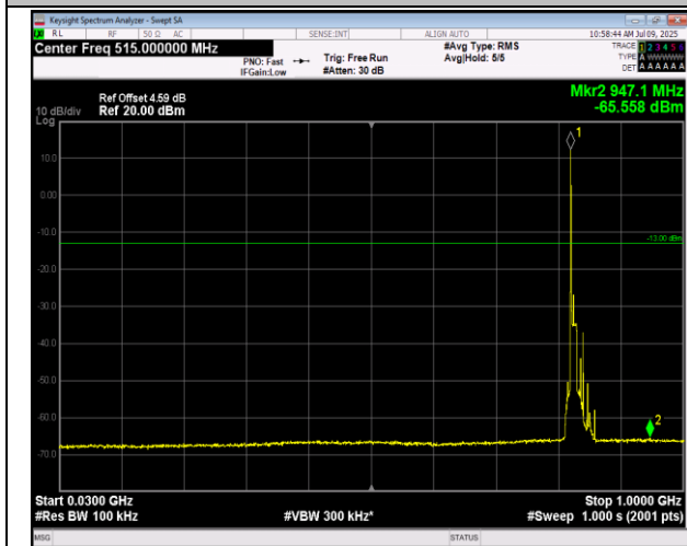
5-5-10MHz-10MHz-16QAM-16QAM-20450-20549-1RB#0 -1RB#49-30~1000MHz-PASS
