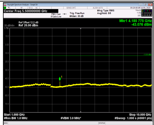
5-5-5MHz-3MHz-QPSK-QPSK-20510-20549-25RB#0-15RB #0-1000~10000MHz-PASS
