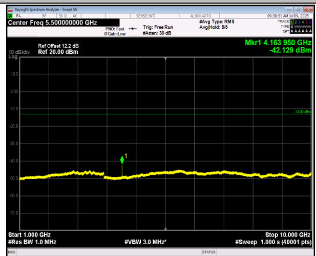
5-5-5MHz-3MHz-16QAM-16QAM-20510-20549-1RB#24-0R B#0-1000~10000MHz-PASS
