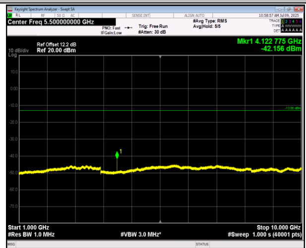
5-5-10MHz-10MHz-16QAM-16QAM-20450-20549-1RB#0-1 RB#49-1000~10000MHz-PASS
