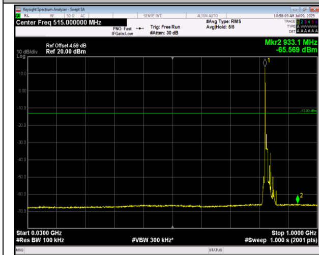
5-5-10MHz-10MHz-QPSK-QPSK-20450-20549-1RB#0-1 RB#49-30~1000MHz-PASS
