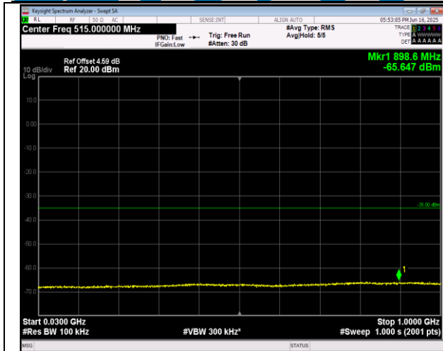
7-7-20MHz-10MHz-QPSK-QPSK-20850-20994-1RB#0-0 RB#0-30~1000MHz-PASS
