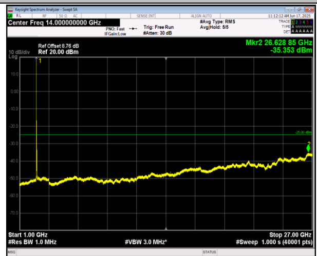
7-7-20MHz-10MHz-16QAM-16QAM-20850-20994-1RB#0-1RB#49-1000~27000MHz-PASS
