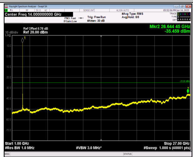
7-7-10MHz-20MHz-16QAM-16QAM-21206-21350-1RB#49- 0RB#0-1000~27000MHz-PASS
