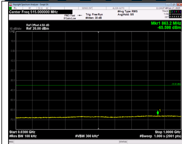
7-7-20MHz-10MHz-16QAM-16QAM-20850-20994-1RB#9 9-0RB#0-30~1000MHz-PASS
