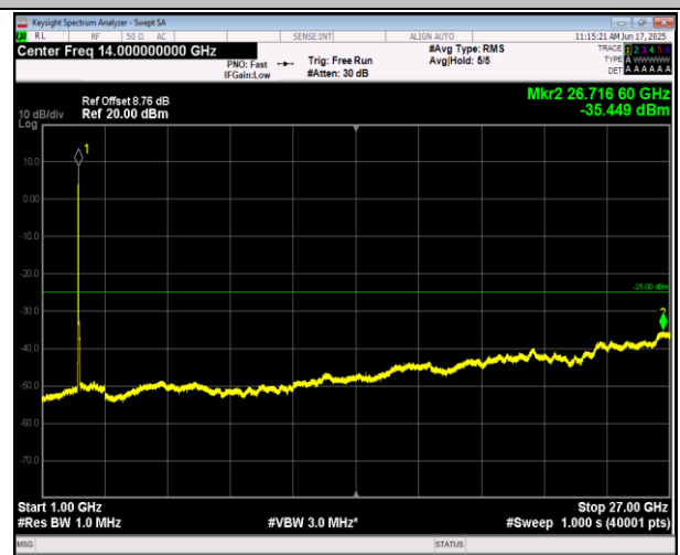
7-7-20MHz-10MHz-16QAM-16QAM-20850-20994-1RB#0-0RB#0-1000~27000MHz-PASS
