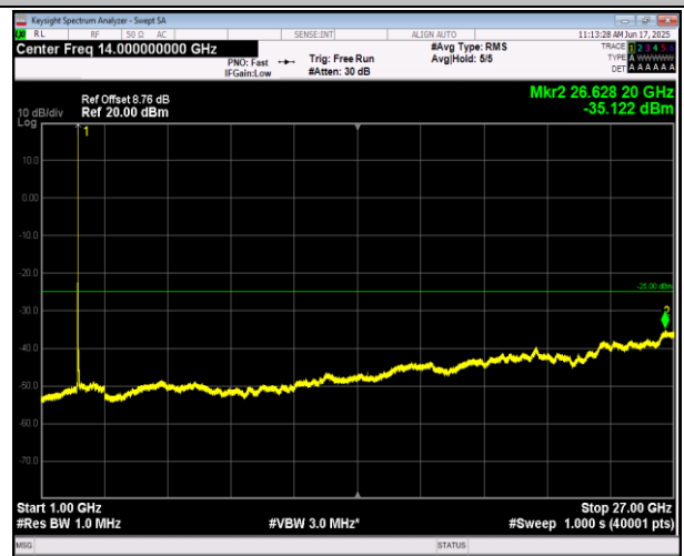
7-7-20MHz-10MHz-16QAM-16QAM-20850-20994-100RB# 0-50RB#0-1000~27000MHz-PASS
