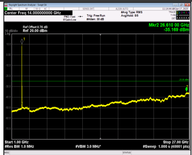
7-7-20MHz-10MHz-16QAM-16QAM-20850-20994-1RB#99- 0RB#0-1000~27000MHz-PASS
