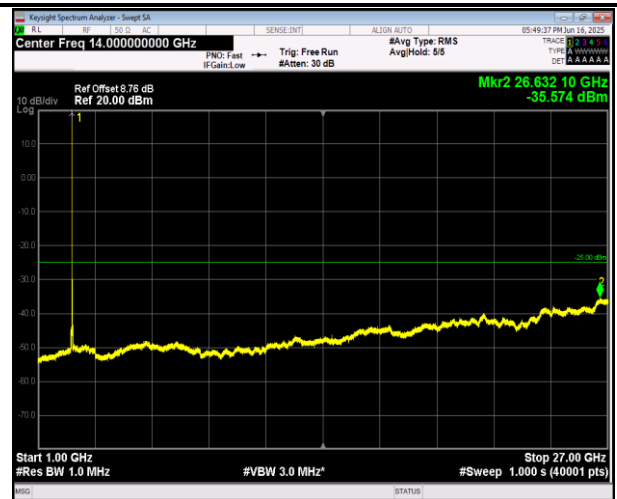
7-7-10MHz-20MHz-16QAM-16QAM-21206-21350-1RB#0-1 RB#99-1000~27000MHz-PASS
