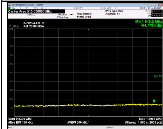
38-38-15MHz-15MHz-16QAM-16QAM-38025-38175-1RB #0-ORB#0-30~1000MHz-PASS
