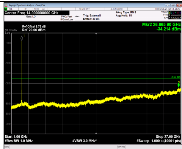
38-38-15MHz-15MHz-QPSK-QPSK-38025-38175-1RB#74- ORB#0-1000~27000MHz-PASS
