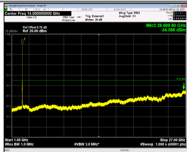
38-38-15MHz-15MHz-16QAM-16QAM-38025-38175-1RB# 0-ORB#0-1000~27000MHz-PASS
