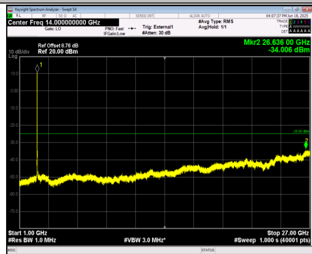
38-38-20MHz-20MHz-16QAM-16QAM-37952-38150-1RB# 0-0RB#0-1000~27000MHz-PASS
