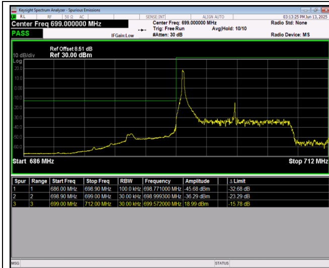
Band12-10MHz-QPSK-23060-50RB#0
