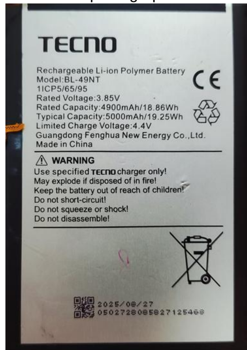
Internal photograph of EUT
