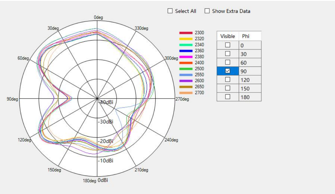
LTE B7/B38/B40/41 Phi=90deg
