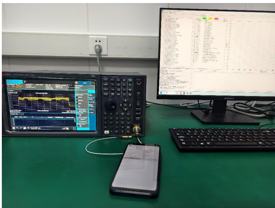
Conducted Test-BT
