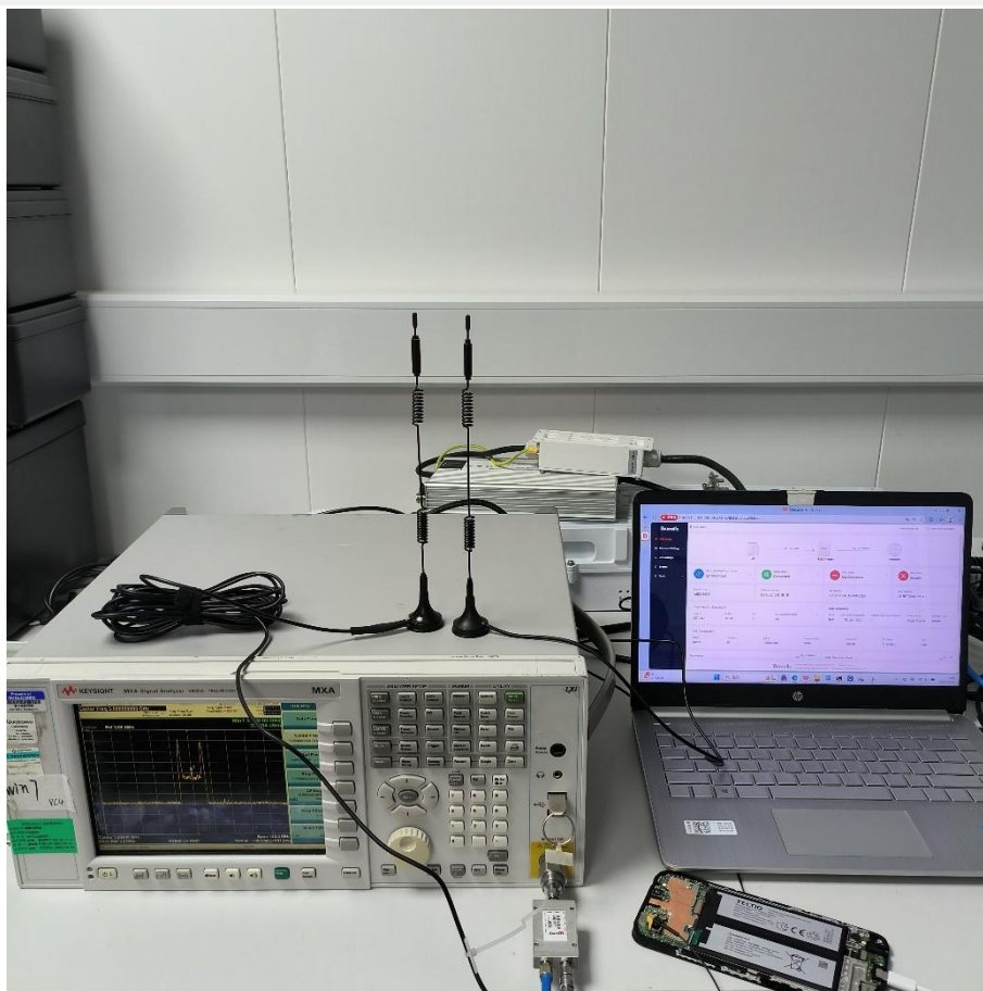
Conducted Test-CBRS
