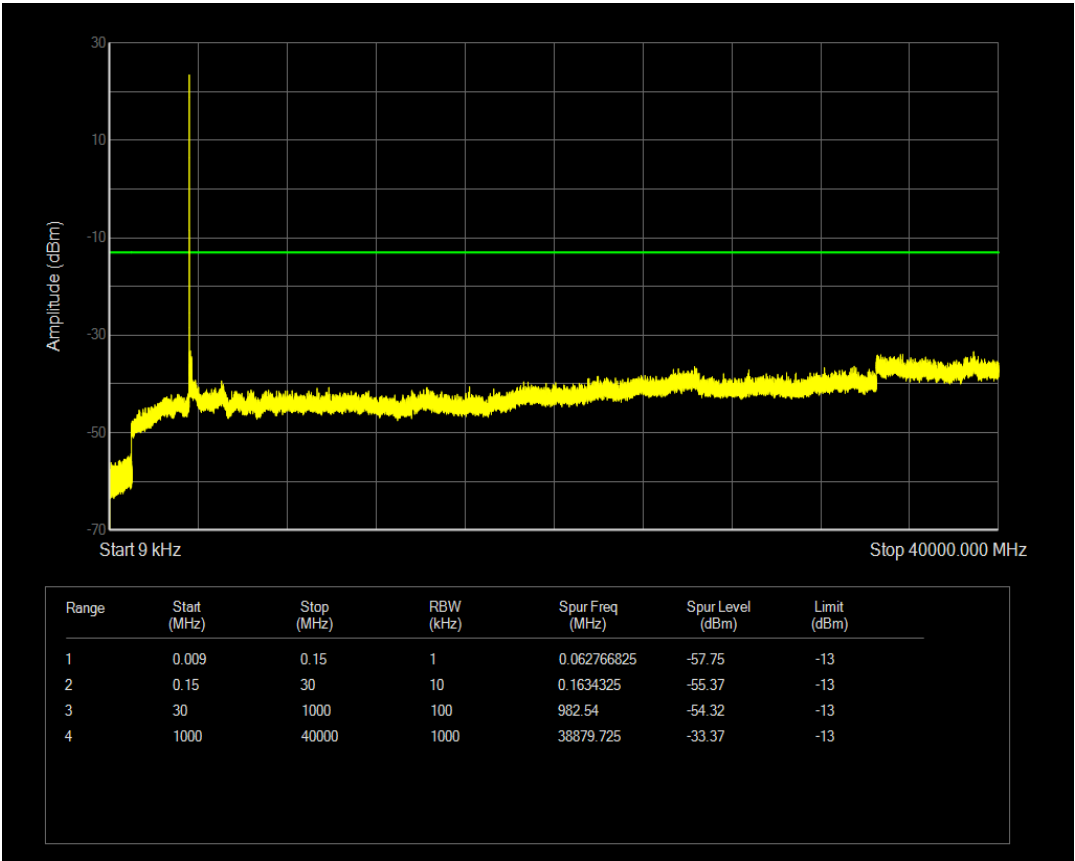
n48 SCS=30kHz CP_QPSK BW=100MHz Channel=643332 RB=1@0
