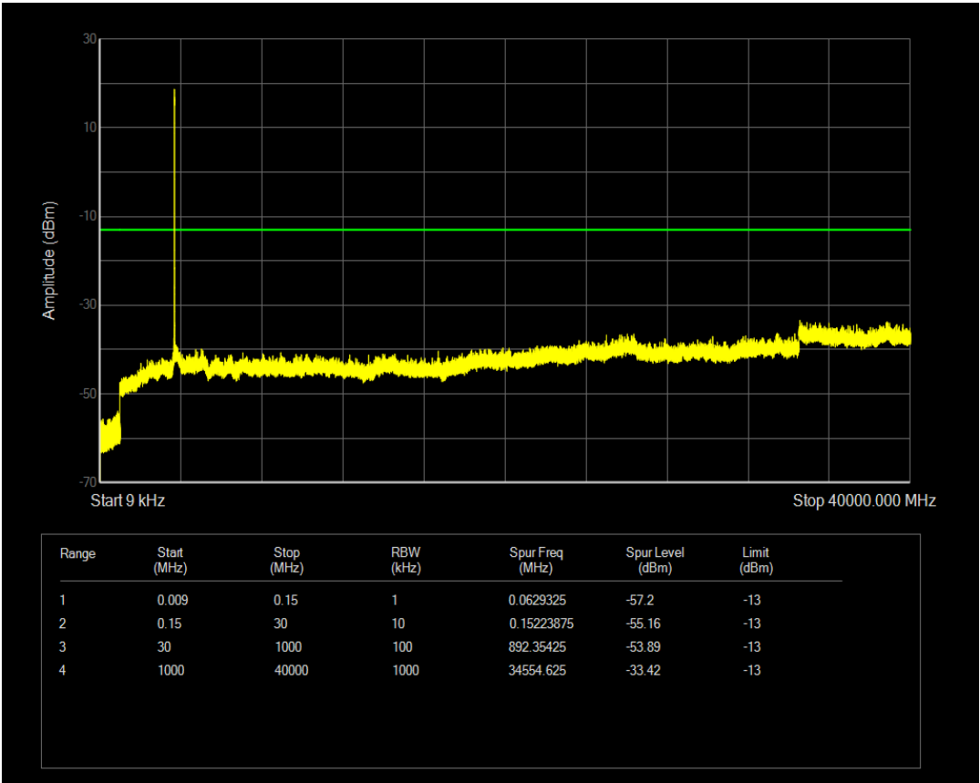
n48 SCS=30kHz CP_QPSK BW=10MHz Channel=646332 RB=1@0
