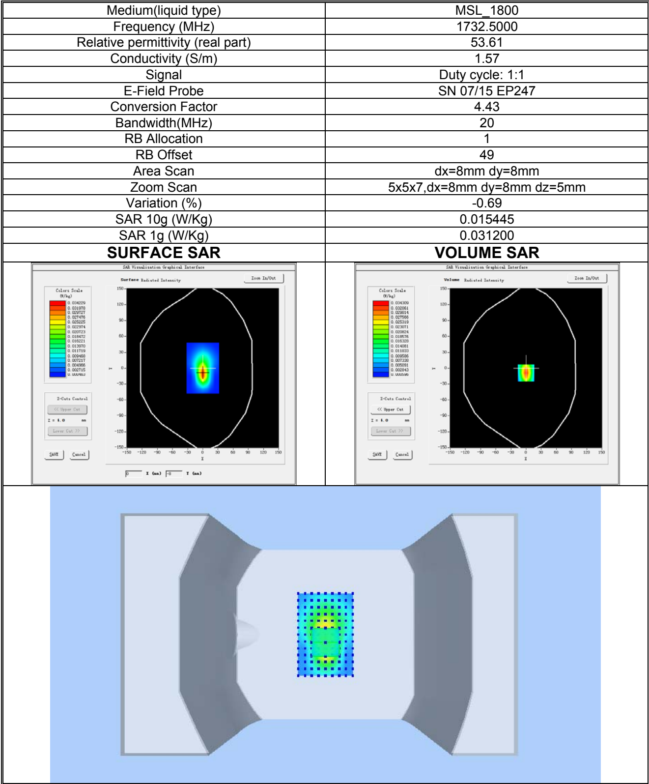
Plot 18:LTE BAND 4, Middle channel (Hotspot, Top Edge) Product Description:Mobile Phone Test Date: 2019-12-24
