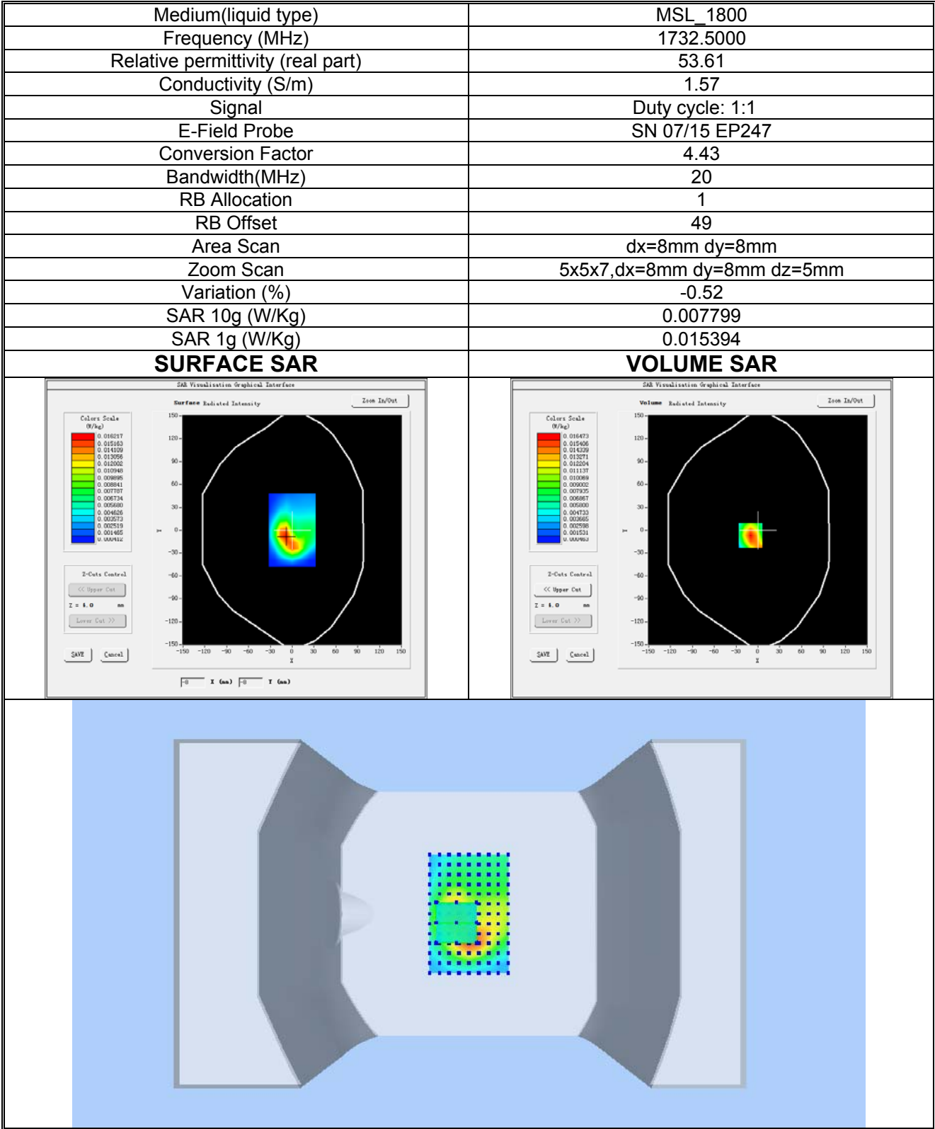
Plot 17:LTE BAND 4, Middle channel (Body-worn, Back Surface) Product Description:Mobile Phone Test Date: 2019-12-24
