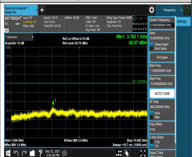
Band17-5MHz-16QAM-23825:1000~10000MHz
