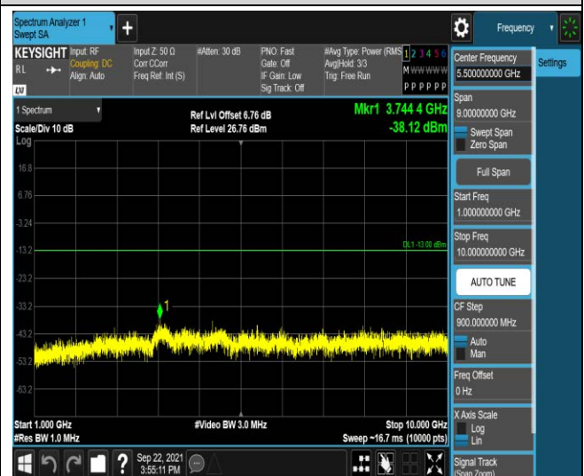
Band17-10MHz-16QAM-23800:1000~10000MHz
