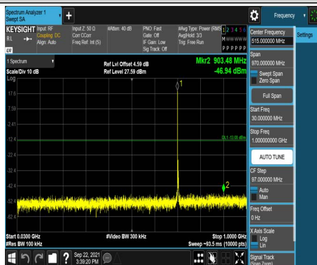
Band17-5MHz-16QAM-23825:30~1000MHz
