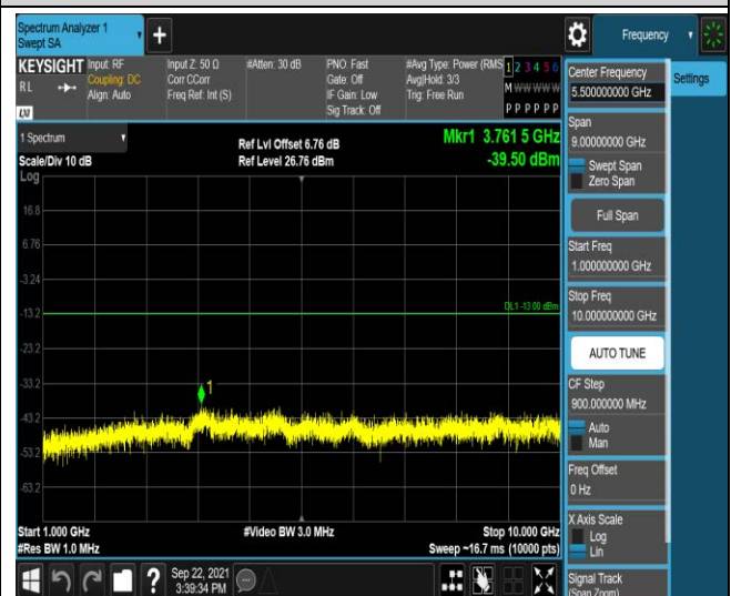
Band17-5MHz-16QAM-23825:1000~10000MHz
