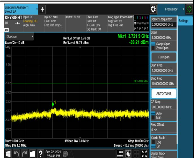
Band17-10MHz-QPSK-23800:1000~10000MHz
