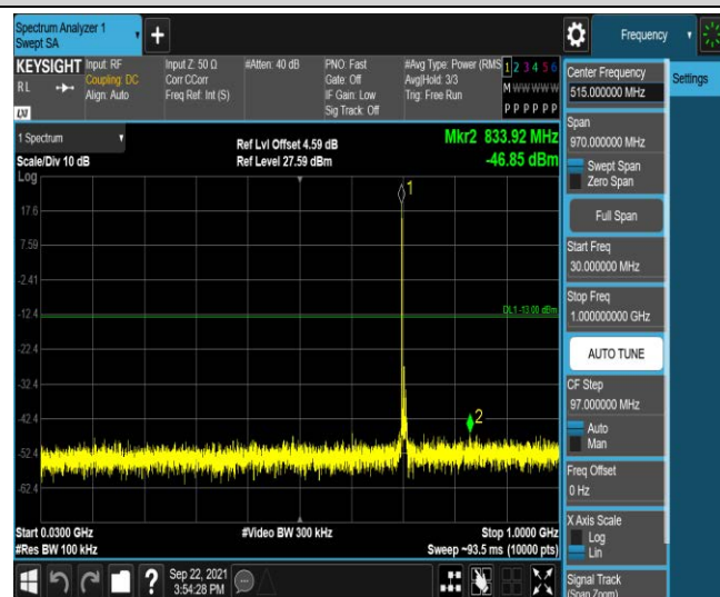
Band17-10MHz-QPSK-23800:30~1000MHz
