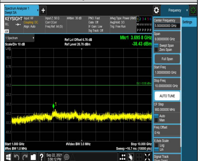
Band17-10MHz-16QAM-23800:1000~10000MHz
