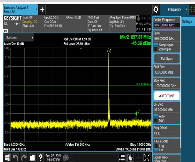
Band17-10MHz-16QAM-23800:30~1000MHz
