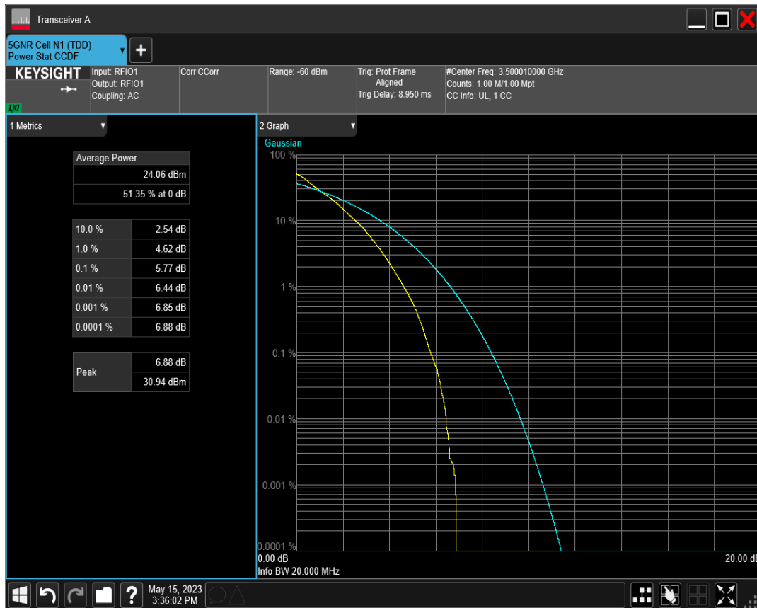
n77(3450-3550) SCS=15kHz DFT_QAM16 BW=15MHz Channel=633334 RB=75@0
