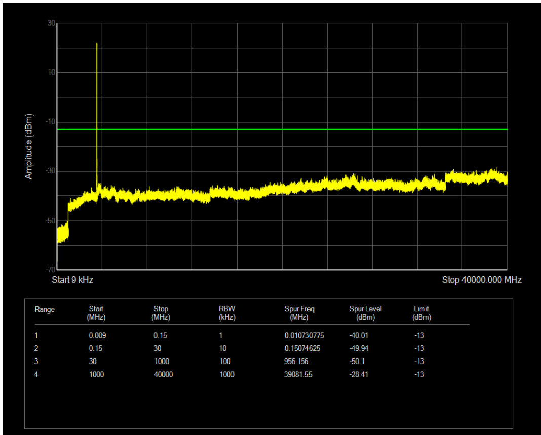
n77(3450-3550) SCS=30kHz DFT_QPSK BW=10MHz Channel=636332 RB=1@0
