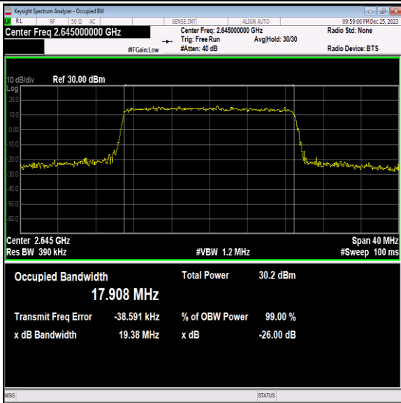
41(2535-2655)-20MHz-16QAM-41140-100RB#0-PASS
