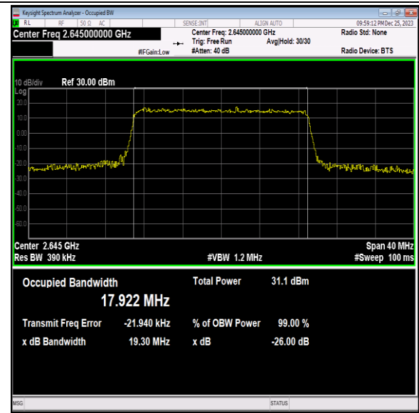
41(2535-2655)-20MHz-64QAM-41140-100RB#0-PASS
