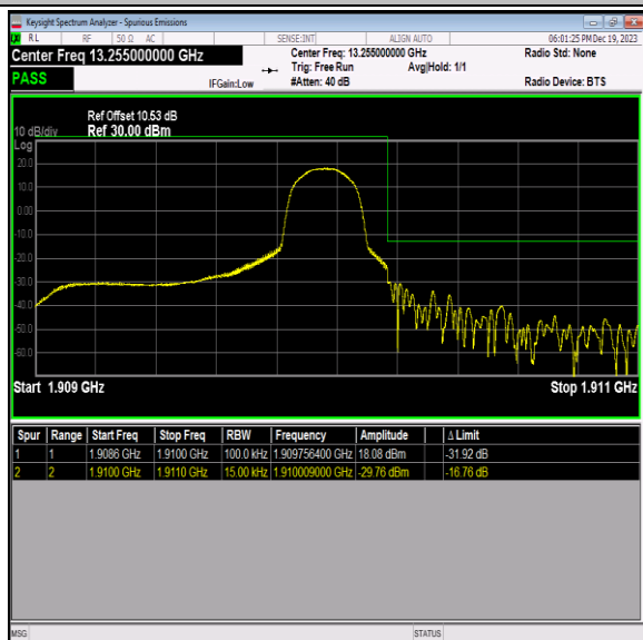
Band2_1.4MHz_16QAM_19193_1RB#5
