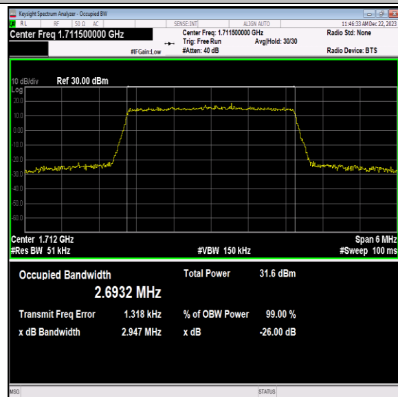
Band66-3MHz-QPSK-131987-15RB#0-PASS
