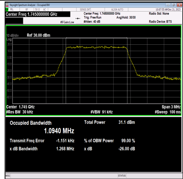
Band66-1.4MHz-QPSK-132322-6RB#0-PASS
