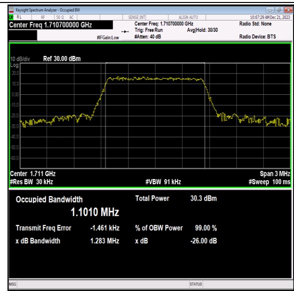
Band66-1.4MHz-16QAM-131979-6RB#0-PASS
