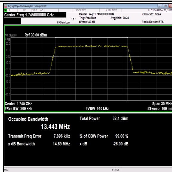
Band66-15MHz-QPSK-132322-75RB#0-PASS
