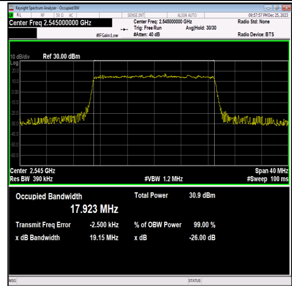
41(2535-2655)-20MHz-64QAM-40140-100RB#0-PASS
