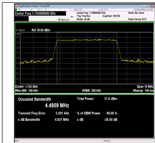
Band66-5MHz-16QAM-132322-25RB#0-PASS
