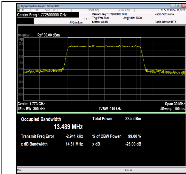
Band66-15MHz-QPSK-132597-75RB#0-PASS
