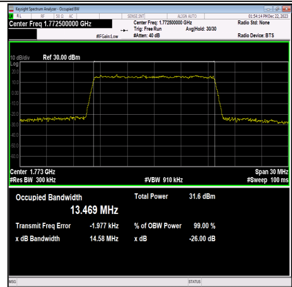
Band66-15MHz-16QAM-132597-75RB#0-PASS
