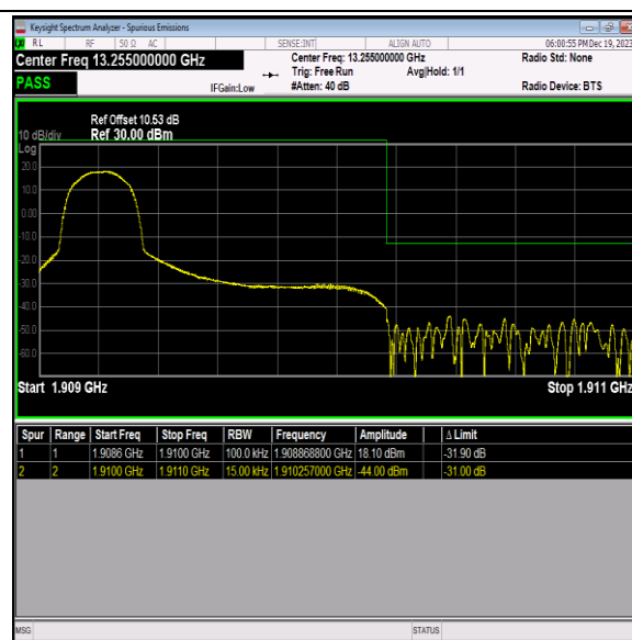
Band2_1.4MHz_16QAM_19193_1RB#0
