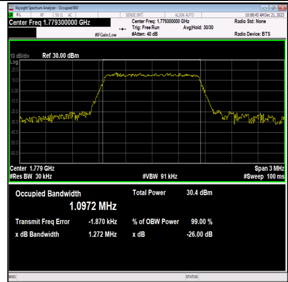
Band66-1.4MHz-16QAM-132665-6RB#0-PASS
