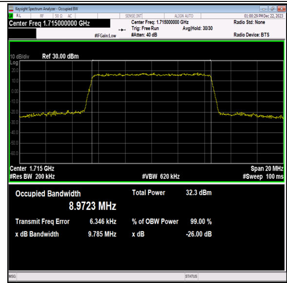
Band66-10MHz-QPSK-132022-50RB#0-PASS
