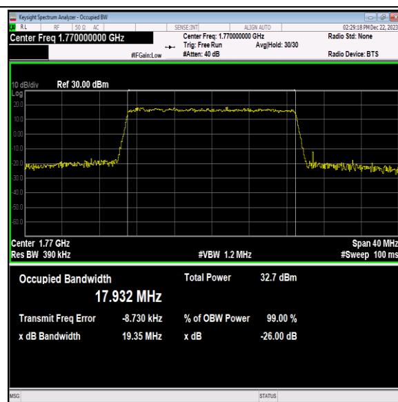
Band66-20MHz-QPSK-132572-100RB#0-PASS
