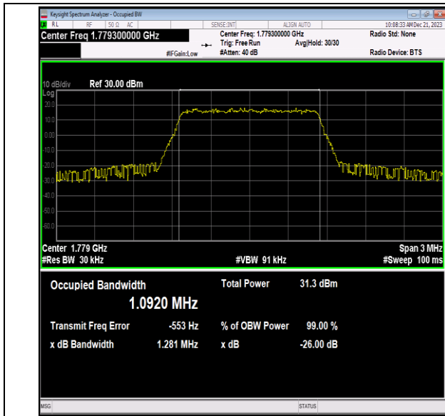
Band66-1.4MHz-QPSK-132665-6RB#0-PASS
