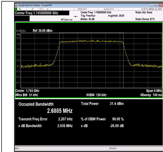
Band66-3MHz-QPSK-132322-15RB#0-PASS
