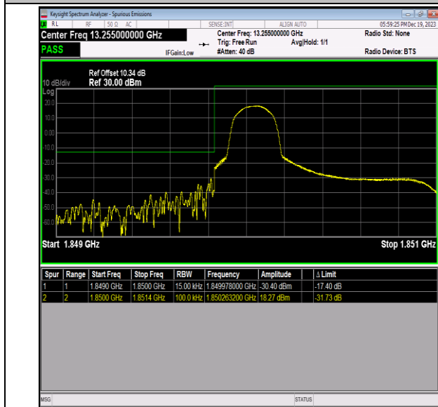
Band2_1.4MHz_16QAM_18607_1RB#0
