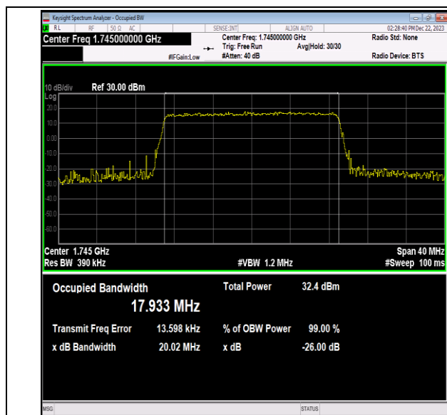
Band66-20MHz-QPSK-132322-100RB#0-PASS
