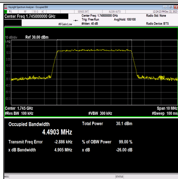
Band66-5MHz-64QAM-132322-25RB#0-PASS
