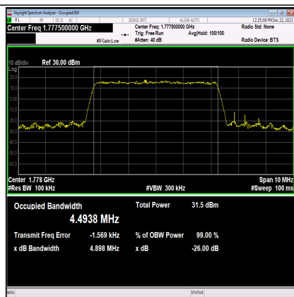
Band66-5MHz-16QAM-132647-25RB#0-PASS
