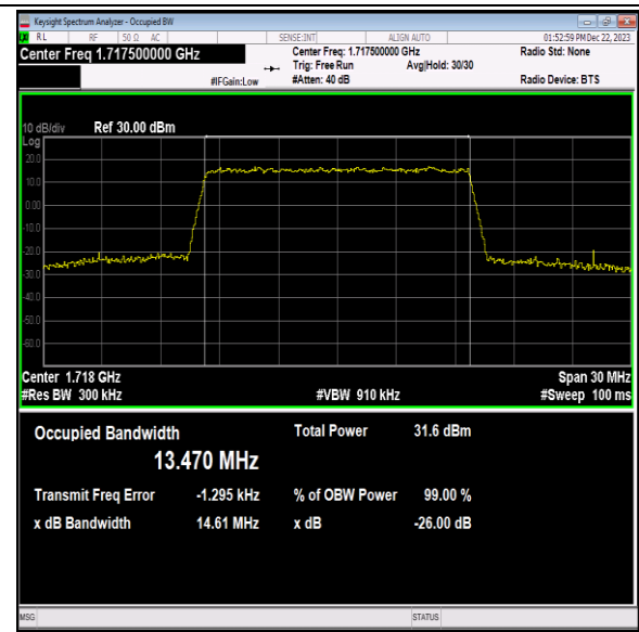
Band66-15MHz-16QAM-132047-75RB#0-PASS
