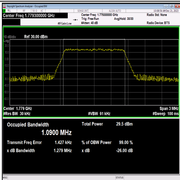
Band66-1.4MHz-64QAM-132665-6RB#0-PASS
