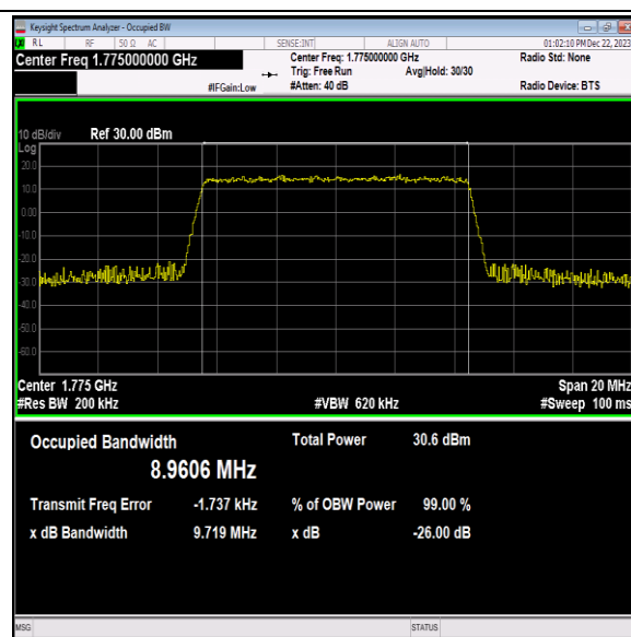
Band66-10MHz-64QAM-132622-50RB#0-PASS
