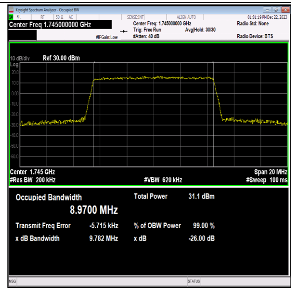
Band66-10MHz-16QAM-132322-50RB#0-PASS
