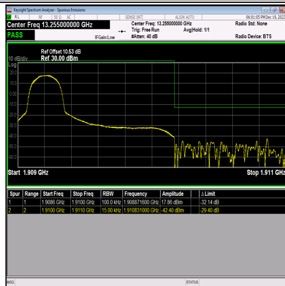
Band2_1.4MHz_64QAM_19193_1RB#0
