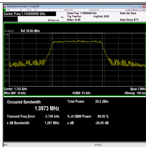
Band66-1.4MHz-64QAM-132322-6RB#0-PASS
