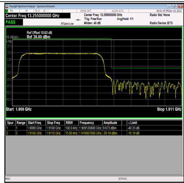
Band2_1.4MHz_QPSK_19193_6RB#0
