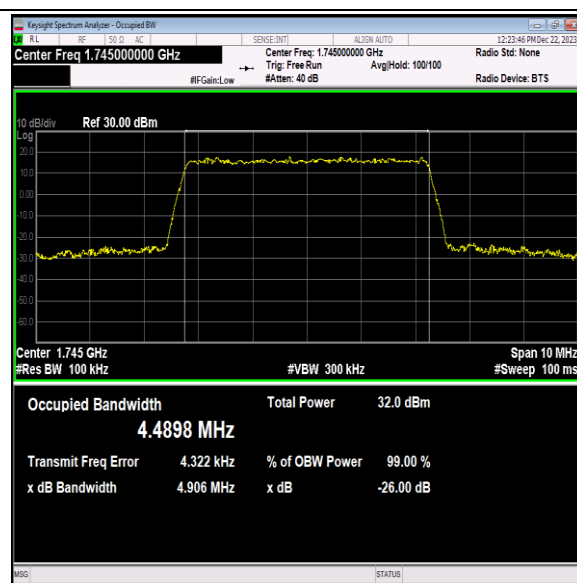
Band66-5MHz-QPSK-132322-25RB#0-PASS
