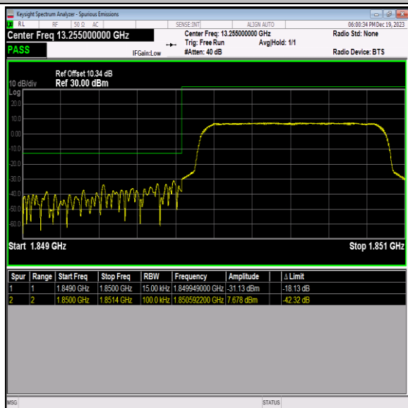
Band2_1.4MHz_64QAM_18607_6RB#0
