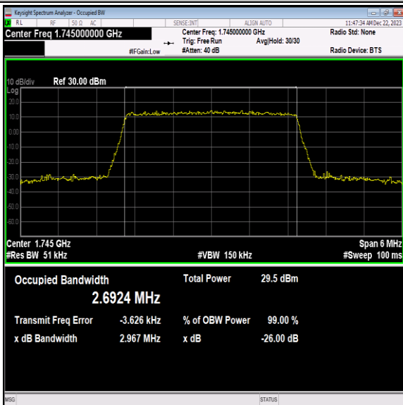
Band66-3MHz-64QAM-132322-15RB#0-PASS
