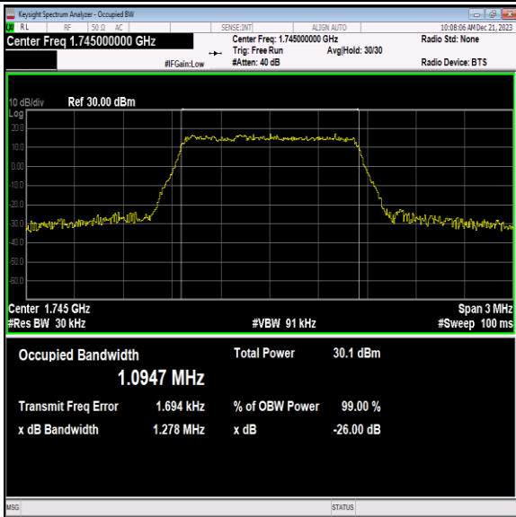
Band66-1.4MHz-16QAM-132322-6RB#0-PASS
