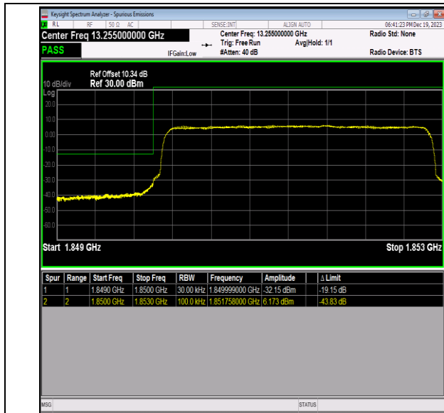
Band2_3MHz_QPSK_18615_15RB#0
