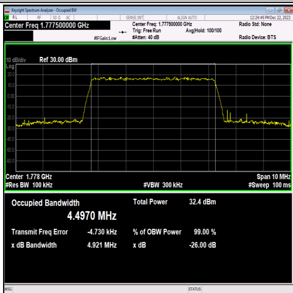
Band66-5MHz-QPSK-132647-25RB#0-PASS
