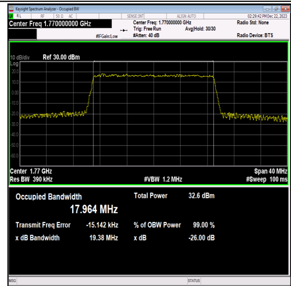
Band66-20MHz-64QAM-132572-100RB#0-PASS
