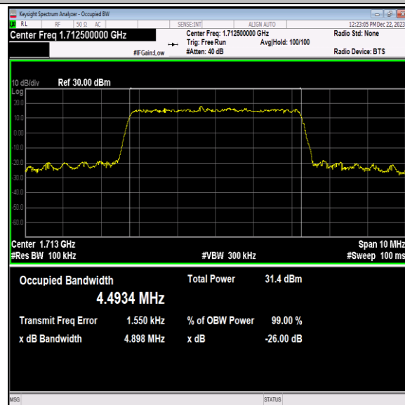
Band66-5MHz-16QAM-131997-25RB#0-PASS
