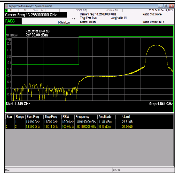
Band2_1.4MHz_16QAM_18607_1RB#5
