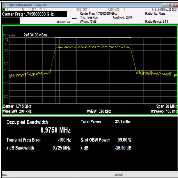
Band66-10MHz-QPSK-132322-50RB#0-PASS
