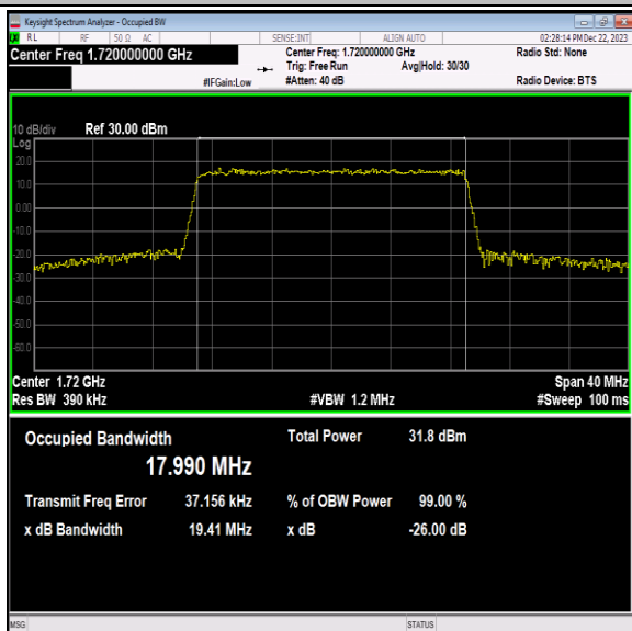
Band66-20MHz-16QAM-132072-100RB#0-PASS
