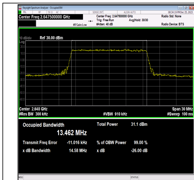
41(2535-2655)-15MHz-64QAM-41165-75RB#0-PASS
