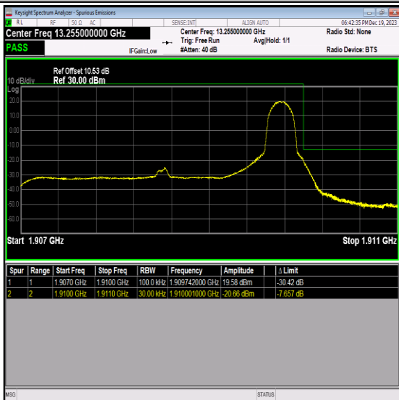
Band2_3MHz_QPSK_19185_1RB#14
