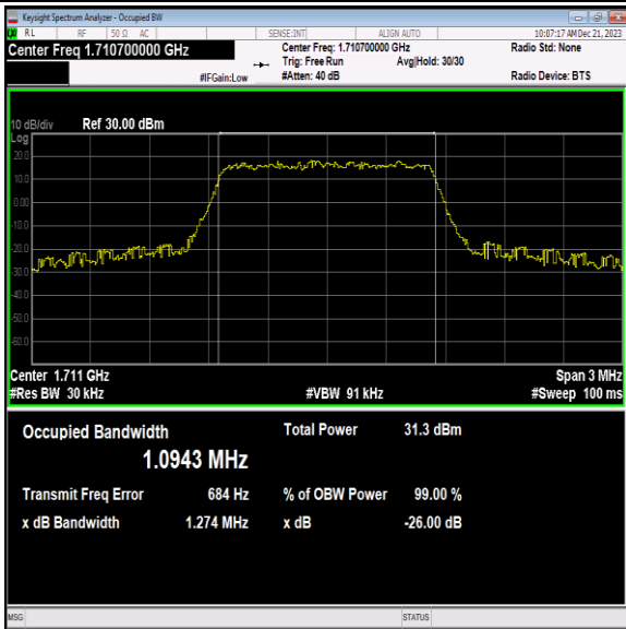
Band66-1.4MHz-QPSK-131979-6RB#0-PASS
