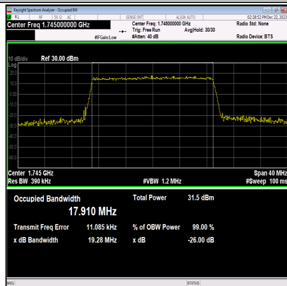
Band66-20MHz-16QAM-132322-100RB#0-PASS
