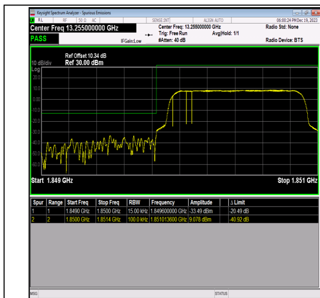
Band2_1.4MHz_16QAM_18607_6RB#0
