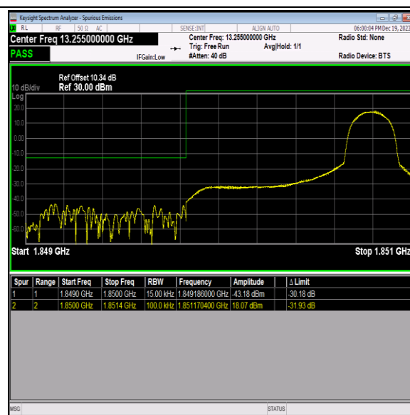
Band2_1.4MHz_64QAM_18607_1RB#5
