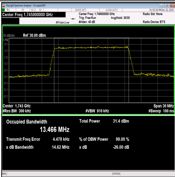
Band66-15MHz-16QAM-132322-75RB#0-PASS
