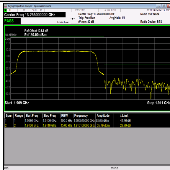
Band2_1.4MHz_16QAM_19193_6RB#0
