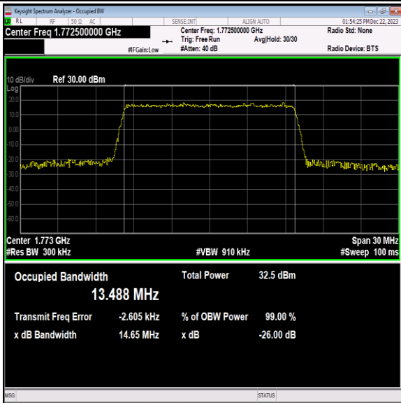
Band66-15MHz-64QAM-132597-75RB#0-PASS
