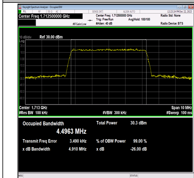
Band66-5MHz-64QAM-131997-25RB#0-PASS
