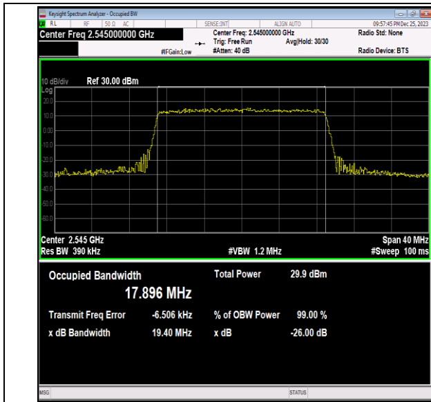
41(2535-2655)-20MHz-16QAM-40140-100RB#0-PASS
