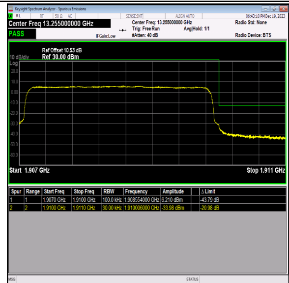
Band2_3MHz_QPSK_19185_15RB#0
