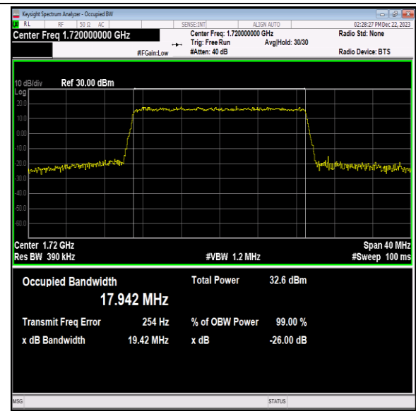
Band66-20MHz-64QAM-132072-100RB#0-PASS
