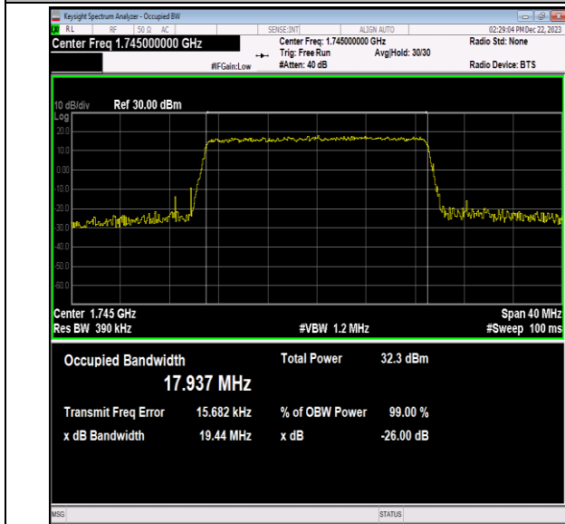
Band66-20MHz-64QAM-132322-100RB#0-PASS
