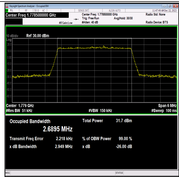
Band66-3MHz-QPSK-132657-15RB#0-PASS
