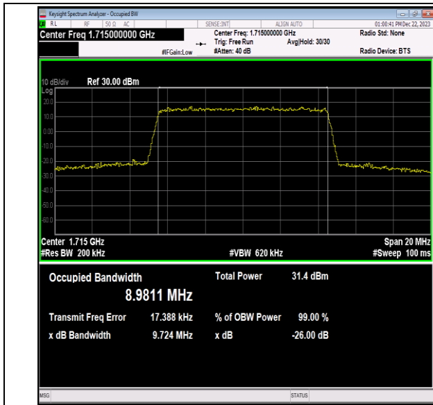
Band66-10MHz-16QAM-132022-50RB#0-PASS
