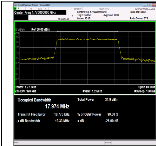
Band66-20MHz-16QAM-132572-100RB#0-PASS
