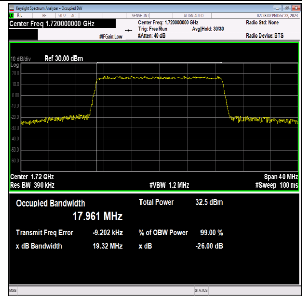
Band66-20MHz-QPSK-132072-100RB#0-PASS
