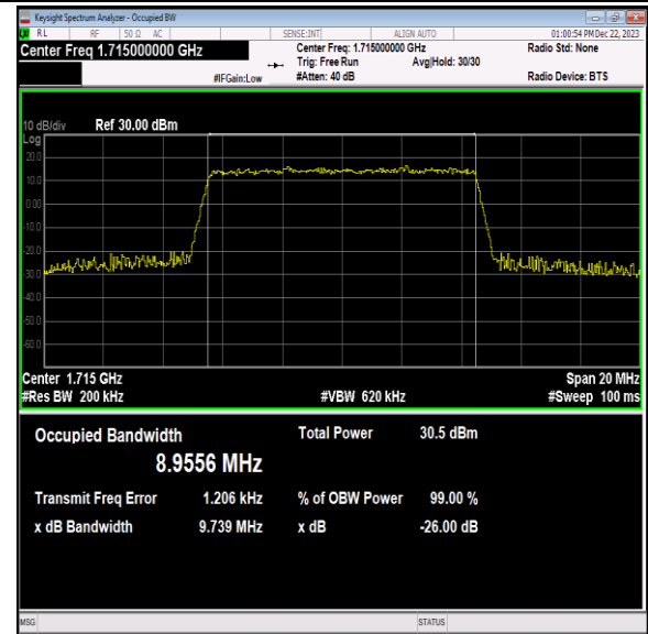
Band66-10MHz-64QAM-132022-50RB#0-PASS
