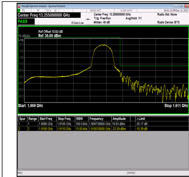
Band2_1.4MHz_QPSK_19193_1RB#5
