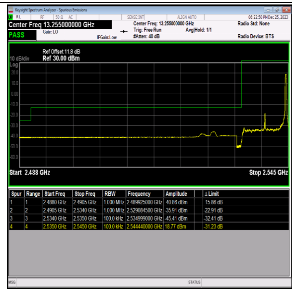
Band41_10MHz_QPSK_40090_1RB#49
