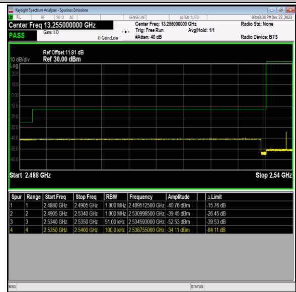
Band41_5MHz_64QAM_40065_1RB#24
