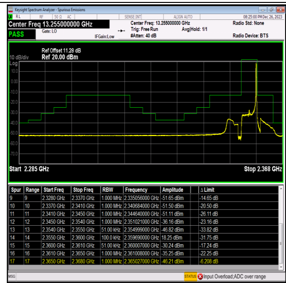
Band40_5MHz_16QAM_39225_1RB#24
