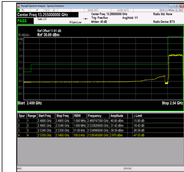
Band41_5MHz_64QAM_40065_25RB#0
