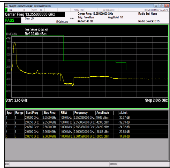
Band41_5MHz_QPSK_41215_1RB#0
