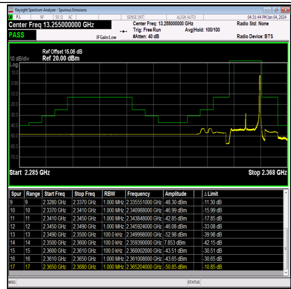
Band40_10MHz_16QAM_39200_1RB#49
