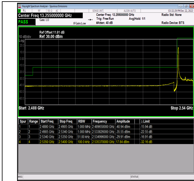
Band41_5MHz_16QAM_40065_1RB#0
