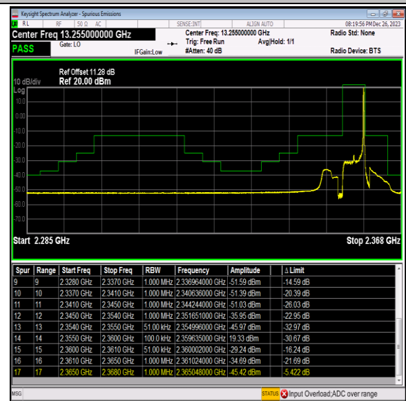
Band40_5MHz_QPSK_39225_1RB#24
