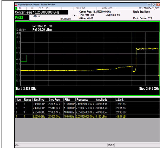
Band41_10MHz_QPSK_40090_50RB#0
