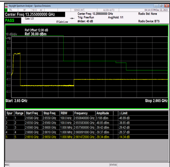
Band41_5MHz_64QAM_41215_25RB#0
