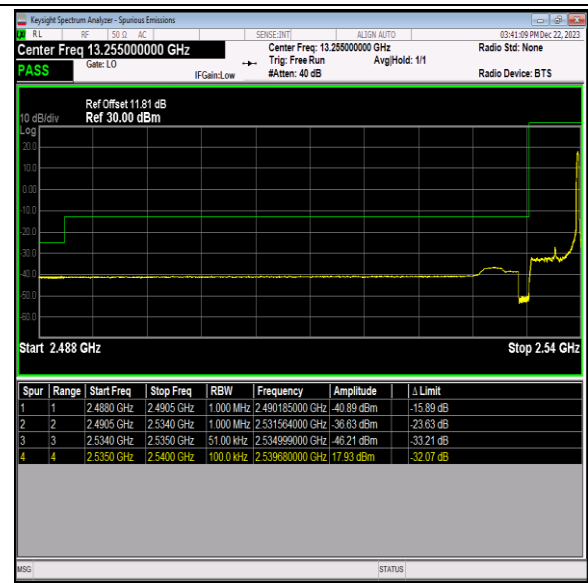
Band41_5MHz_16QAM_40065_1RB#24
