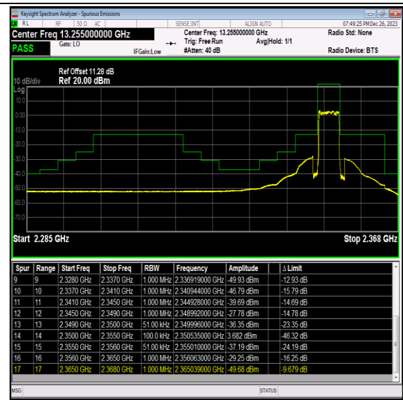
Band40_5MHz_QPSK_39175_25RB#0
