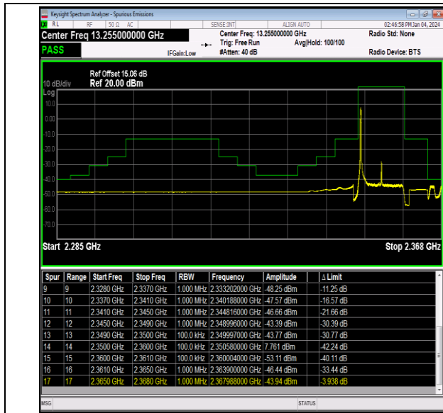
Band40_10MHz_16QAM_39200_1RB#0
