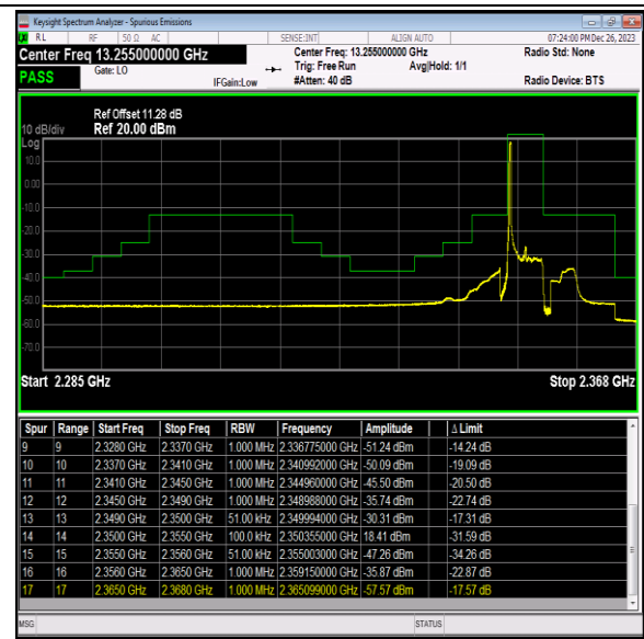
Band40_5MHz_16QAM_39175_1RB#0
