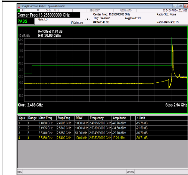
Band41_5MHz_64QAM_40065_1RB#0
