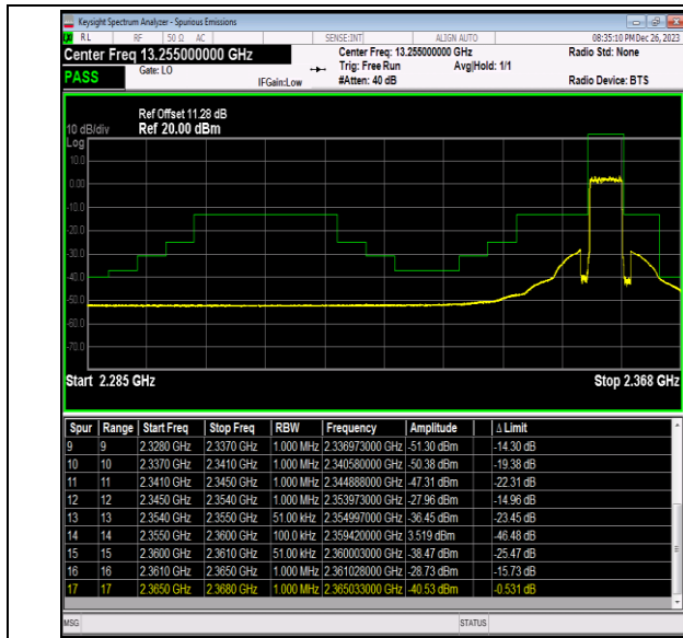
Band40_5MHz_QPSK_39225_25RB#0
