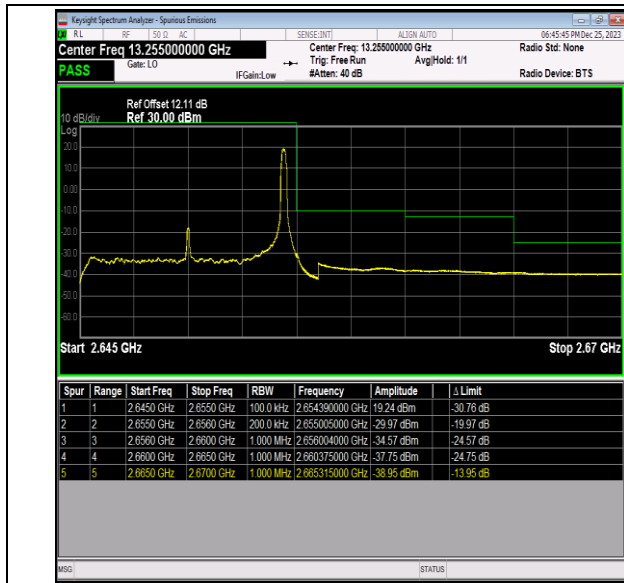
Band41_10MHz_QPSK_41190_1RB#49
