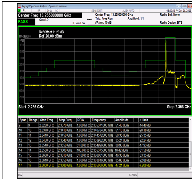
Band40_5MHz_16QAM_39225_1RB#0
