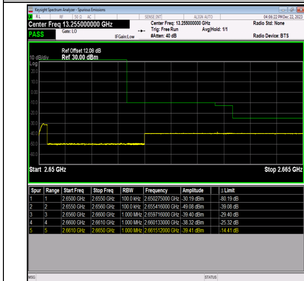
Band41_5MHz_64QAM_41215_1RB#24
