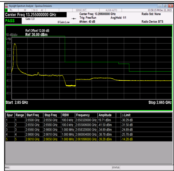
Band41_5MHz_64QAM_41215_1RB#0
