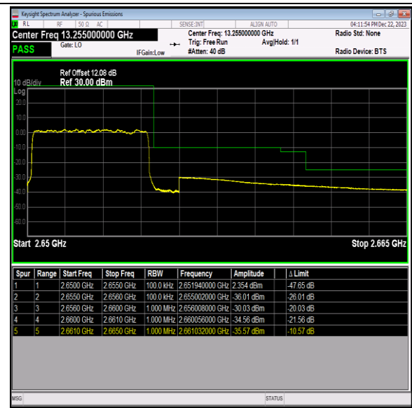
Band41_5MHz_16QAM_41215_25RB#0
