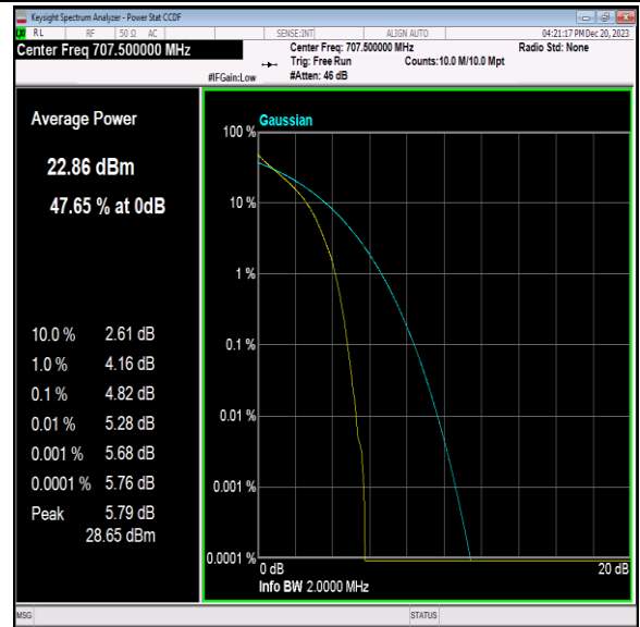
Band12-1.4MHz-QPSK-23095-6RB#0-PASS
