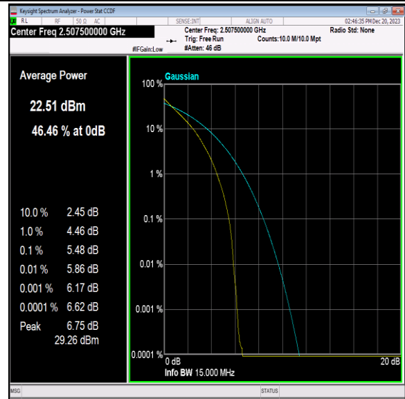
Band7-15MHz-QPSK-20825-75RB#0-PASS
