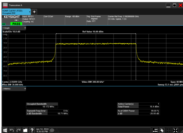
20MHz_30kHz_2592.99MHz_CP-OFDM 256 QAM_RB51@0&18.172 MHz
