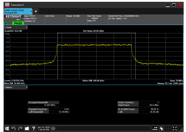
15MHz_30kHz_2503.5MHz_DFT-s-OFDM 16 QAM_RB36@0&amp;13.455 MHz
