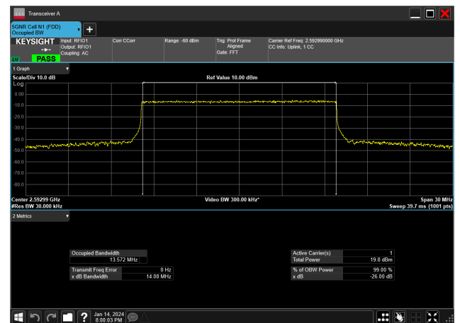
15MHz_30kHz_2592.99MHz_CP-OFDM QPSK_RB38@0&amp;13.572 MHz
