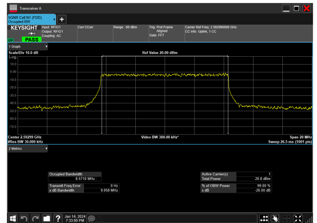
10MHz_30kHz_2592.99MHz_DFT-s-OFDM 16 QAM_RB24@0&amp;8.571 MHz
