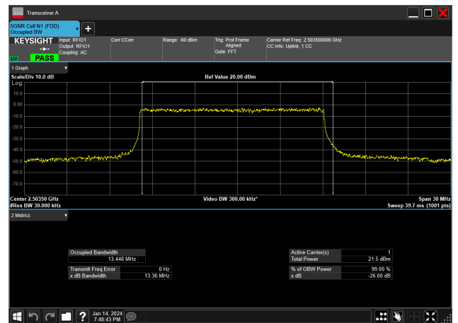
15MHz_30kHz_2503.5MHz_DFT-s-OFDM QPSK_RB36@0&amp;13.448 MHz
