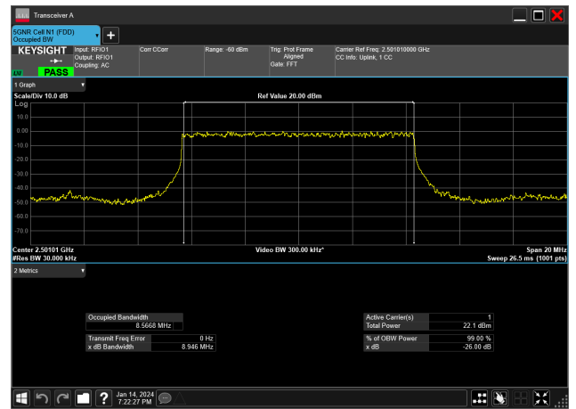
10MHz_30kHz_2501.01MHz_DFT-s-OFDM 16 BPSK_RB24@0&8.567 MHz
