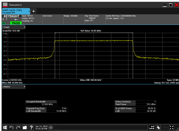
15MHz_30kHz_2503.5MHz_CP-OFDM QPSK_RB38@0&amp;13.565 MHz
