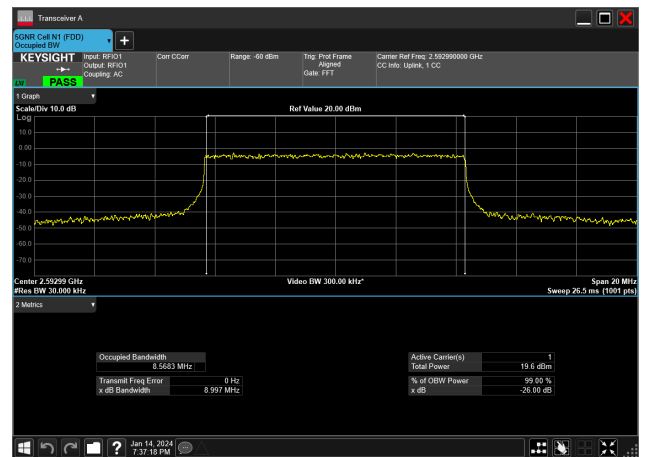
10MHz_30kHz_2592.99MHz_CP-OFDM 64 QAM_RB24@0&8.568 MHz
