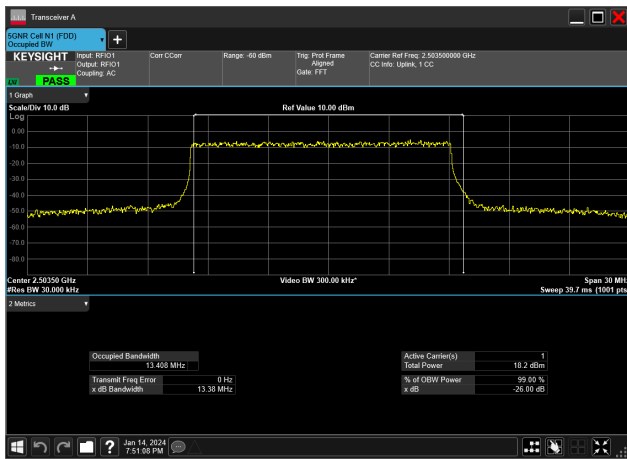
15MHz_30kHz_2503.5MHz_DFT-s-OFDM 256 QAM_RB36@0&amp;13.408 MHz
