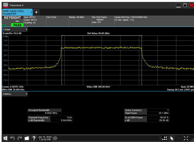
10MHz_30kHz_2501.01MHz_DFT-s-OFDM 64 QAM_RB24@0&8.569 MHz
