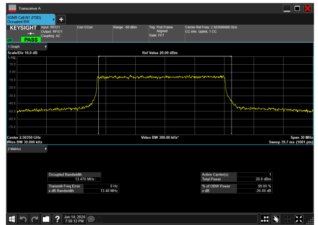
15MHz_30kHz_2503.5MHz_DFT-s-OFDM 64 QAM_RB36@0&amp;13.470 MHz
