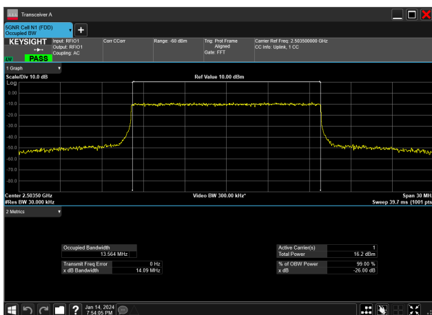
15MHz_30kHz_2503.5MHz_CP-OFDM 256 QAM_RB38@0&amp;13.564 MHz
