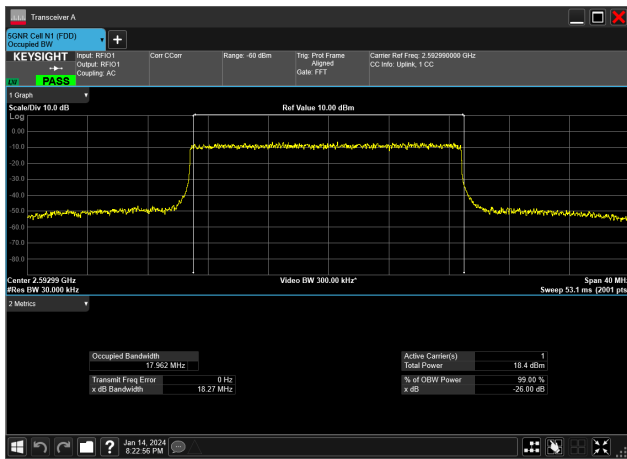
20MHz_30kHz_2592.99MHz_DFT-s-OFDM 256 QAM_RB50@0&amp;17.962 MHz
