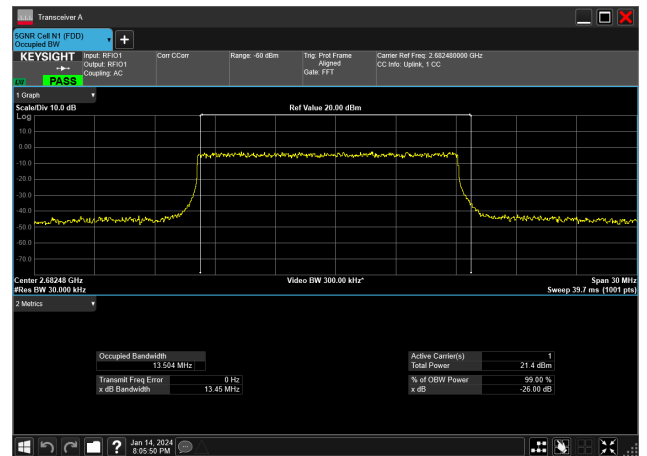
15MHz_30kHz_2682.48MHz_DFT-s-OFDM 16 QAM_RB36@0&amp;13.504 MHz
