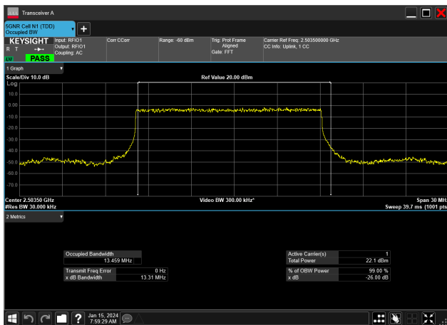
15MHz_30kHz_2503.5MHz_DFT-s-OFDM PI/2 BPSK_RB36@0&amp;13.459 MHz
