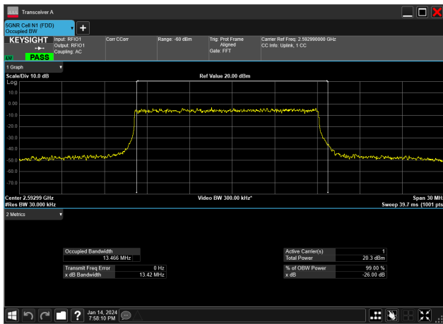
15MHz_30kHz_2592.99MHz_DFT-s-OFDM 64 QAM_RB36@0&13.466 MHz
