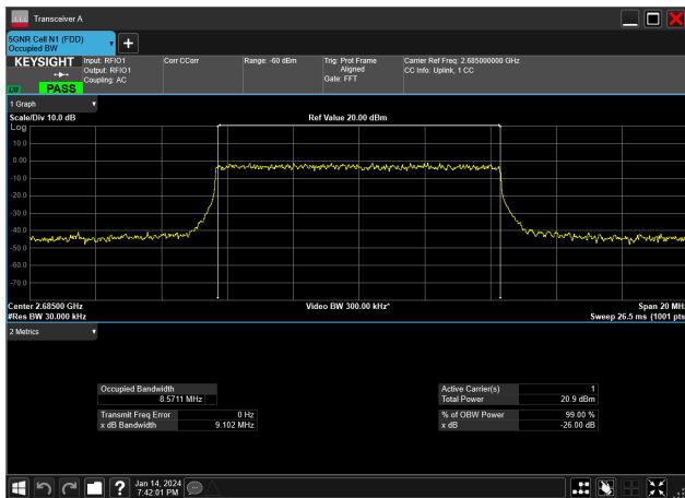
10MHz_30kHz_2685MHz_DFT-s-OFDM 64 QAM_RB24@0&amp;8.571 MHz
