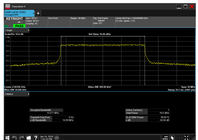
15MHz_30kHz_2503.5MHz_CP-OFDM 64 QAM_RB38@0&amp;13.571 MHz
