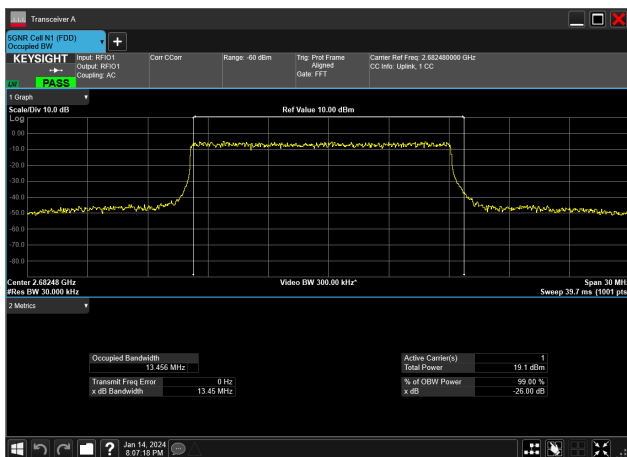
15MHz_30kHz_2682.48MHz_DFT-s-OFDM 256 QAM_RB36@0&amp;13.456 MHz
