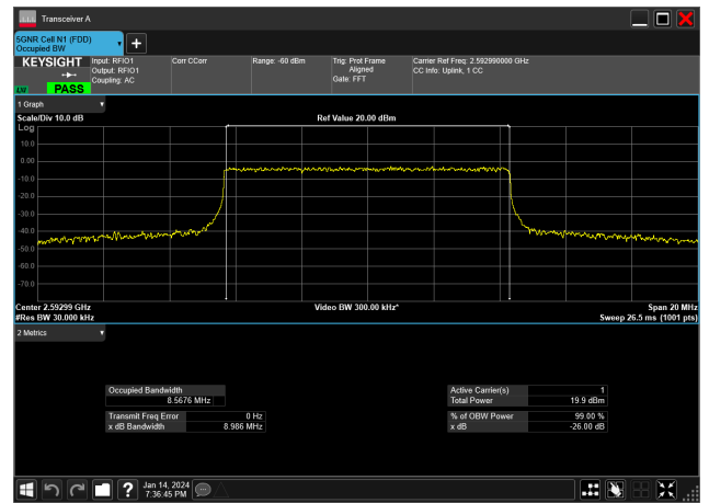
10MHz_30kHz_2592.99MHz_CP-OFDM 16 QAM_RB24@0&8.568 MHz
