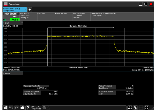
20MHz_30kHz_2506.02MHz_CP-OFDM 256 QAM_RB51@0&amp;18.177 MHz
