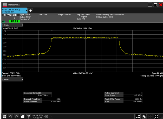
10MHz_30kHz_2592.99MHz_CP-OFDM 256 QAM_RB24@0&8.568 MHz
