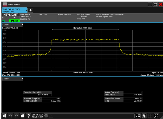
10MHz_30kHz_2685MHz_CP-OFDM 16 QAM_RB24@0&amp;8.570 MHz
