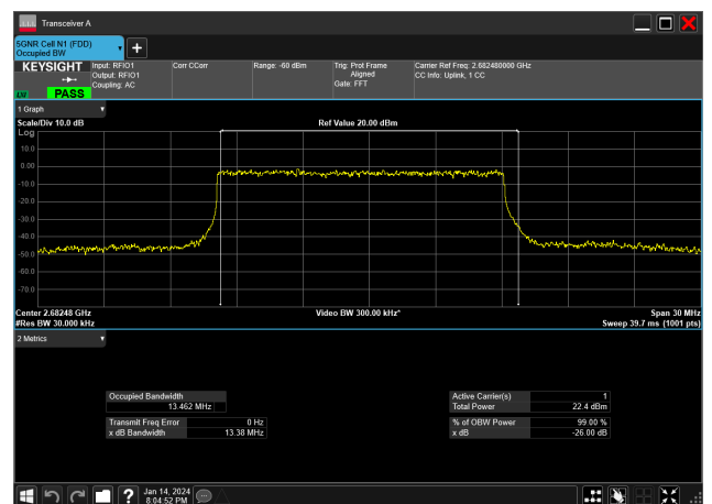
15MHz_30kHz_2682.48MHz_DFT-s-OFDM QPSK_RB36@0&amp;13.462 MHz
