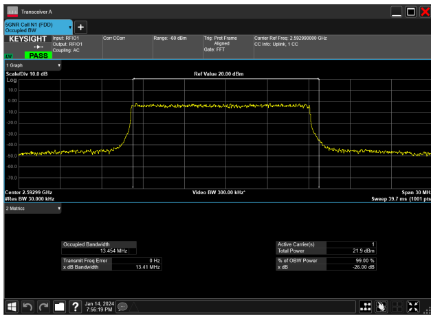
15MHz_30kHz_2592.99MHz_DFT-s-OFDM QPSK_RB36@0&13.454 MHz
