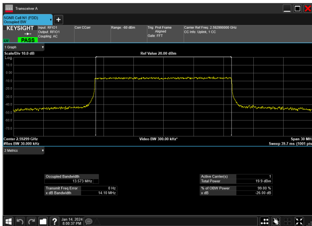
15MHz_30kHz_2592.99MHz_CP-OFDM 16 QAM_RB38@0&amp;13.573 MHz
