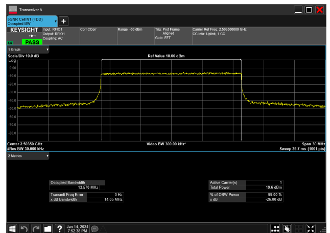
15MHz_30kHz_2503.5MHz_CP-OFDM 16 QAM_RB38@0&amp;13.570 MHz
