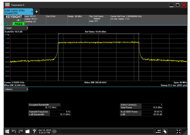
20MHz_30kHz_2592.99MHz_CP-OFDM 16 QAM_RB51@0&18.172 MHz
