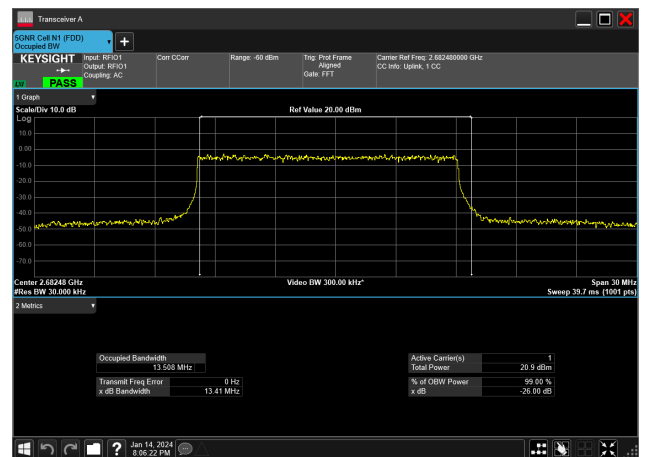
15MHz_30kHz_2682.48MHz_DFT-s-OFDM 64 QAM_RB36@0&amp;13.508 MHz
