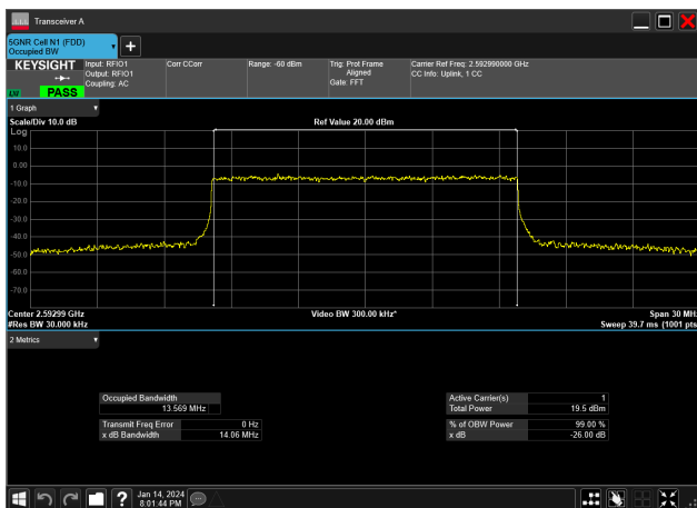
15MHz_30kHz_2592.99MHz_CP-OFDM 64 QAM_RB38@0&amp;13.569 MHz
