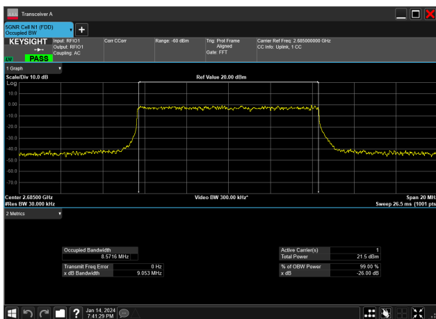
10MHz_30kHz_2685MHz_DFT-s-OFDM 16 QAM_RB24@0&amp;8.572 MHz
