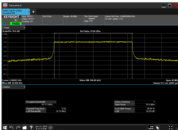
20MHz_30kHz_2506.02MHz_CP-OFDM 64 QAM_RB51@0&amp;18.171 MHz
