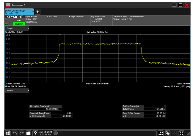
15MHz_30kHz_2592.99MHz_CP-OFDM 256 QAM_RB38@0&amp;13.563 MHz
