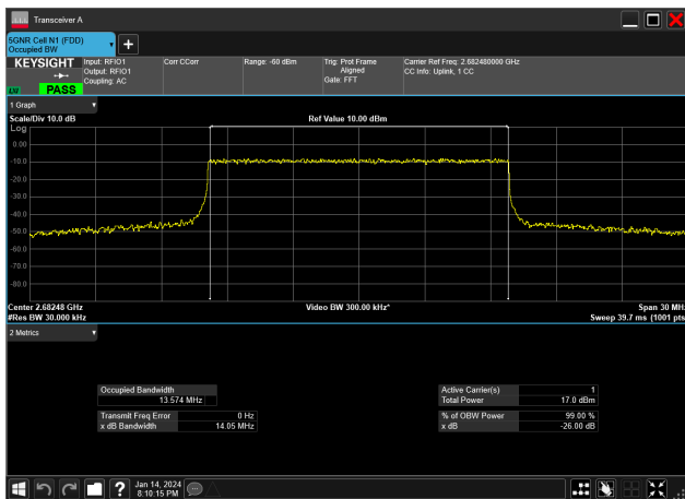
15MHz_30kHz_2682.48MHz_CP-OFDM 256 QAM_RB38@0&13.574 MHz
