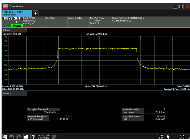
15MHz_30kHz_2592.99MHz_DFT-s-OFDM 16 QAM_RB36@0&amp;13.458 MHz
