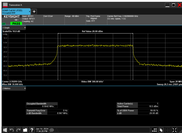
10MHz_30kHz_2592.99MHz_DFT-s-OFDM 256 QAM_RB24@0&amp;8.564 MHz
