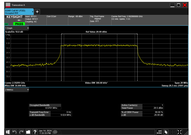
10MHz_30kHz_2592.99MHz_DFT-s-OFDM 64 QAM_RB24@0&amp;8.570 MHz
