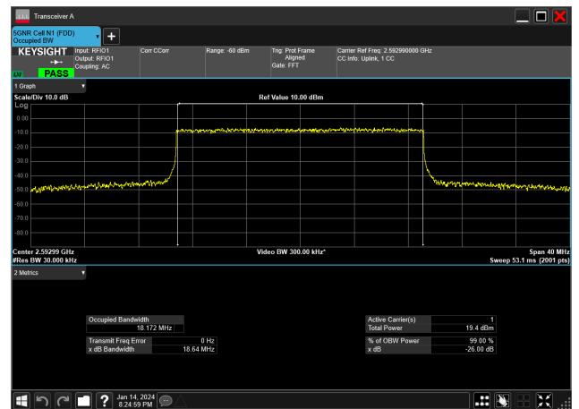
20MHz_30kHz_2592.99MHz_CP-OFDM 64 QAM_RB51@0&18.172 MHz
