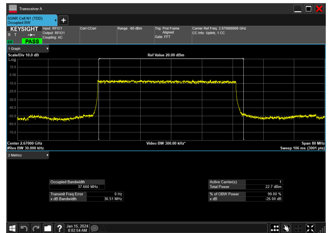
40MHz_30kHz_2670MHz_DFT-s-OFDM PI/2 BPSK_RB100@0&amp;37.660 MHz
