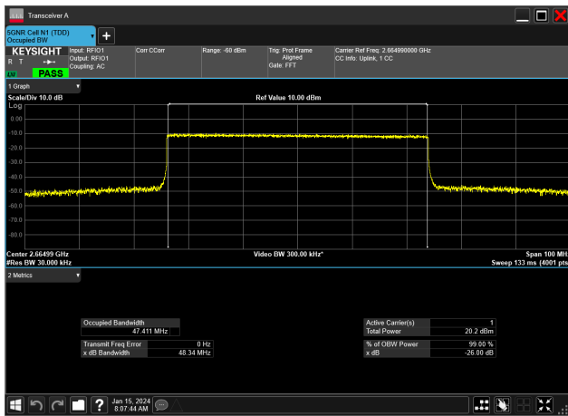
50MHz_30kHz_2664.99MHz_CP-OFDM QPSK_RB133@0&amp;47.411 MHz
