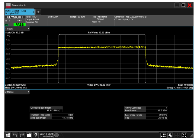
50MHz_30kHz_2592.99MHz_CP-OFDM 256 QAM_RB133@0&amp;47.413 MHz
