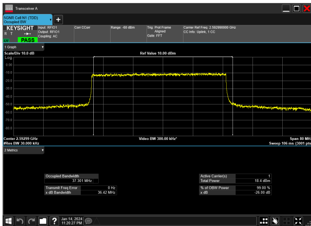
40MHz_30kHz_2592.99MHz_DFT-s-OFDM 256 QAM_RB100@0&amp;37.301 MHz
