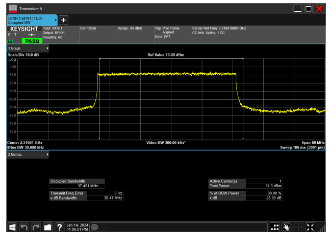
40MHz_30kHz_2516.01MHz_DFT-s-OFDM PI/2 BPSK_RB100@0&37.451 MHz
