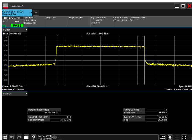
40MHz_30kHz_2670MHz_CP-OFDM 64 QAM_RB106@0&amp;37.778 MHz
