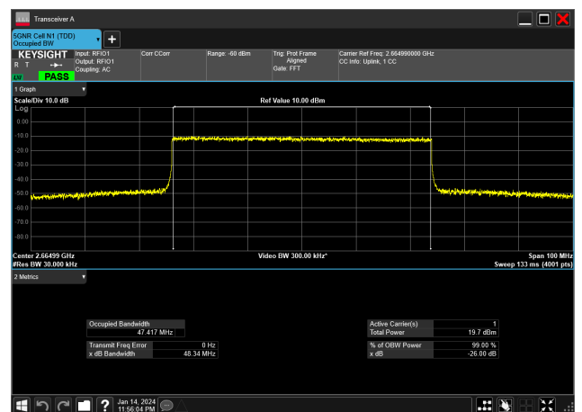
50MHz_30kHz_2664.99MHz_CP-OFDM 64 QAM_RB133@0&47.417 MHz
