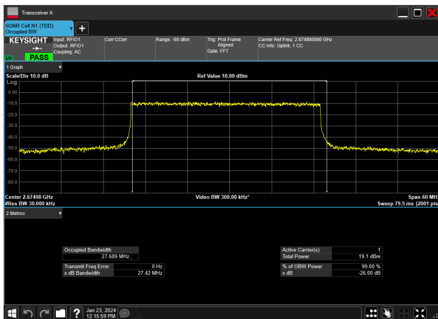
30MHz_30kHz_2674.98MHz_DFT-s-OFDM 256 QAM_RB75@0&amp;27.689 MHz
