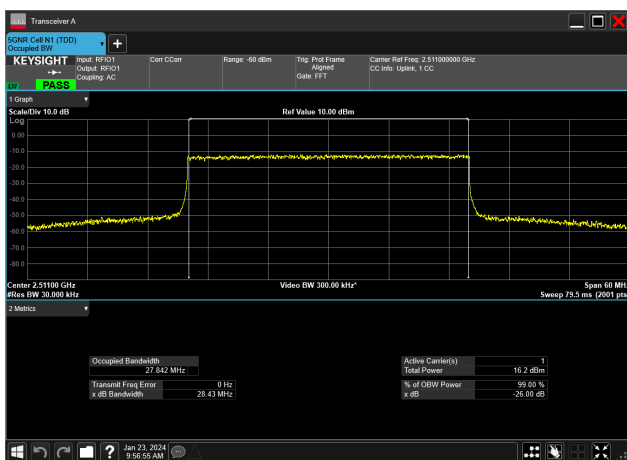
30MHz_30kHz_2511MHz_CP-OFDM 256 QAM_RB78@0&27.842 MHz
