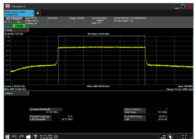
50MHz_30kHz_2521.02MHz_CP-OFDM 64 QAM_RB133@0&amp;47.367 MHz
