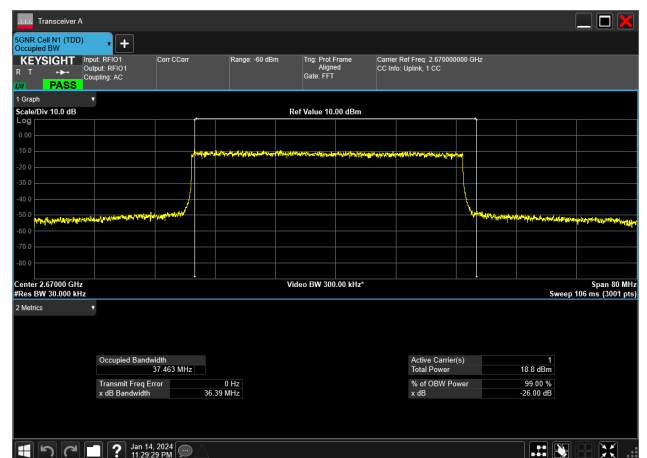
40MHz_30kHz_2670MHz_DFT-s-OFDM 256 QAM_RB100@0&amp;37.463 MHz
