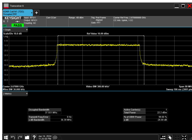
40MHz_30kHz_2670MHz_DFT-s-OFDM QPSK_RB100@0&amp;37.551 MHz
