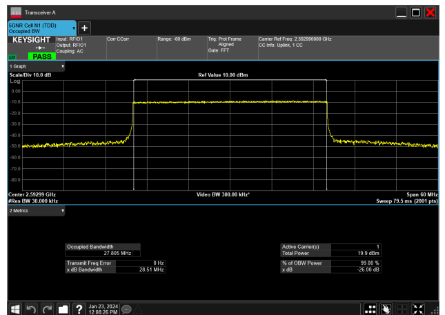
30MHz_30kHz_2592.99MHz_CP-OFDM QPSK_RB78@0&amp;27.805 MHz
