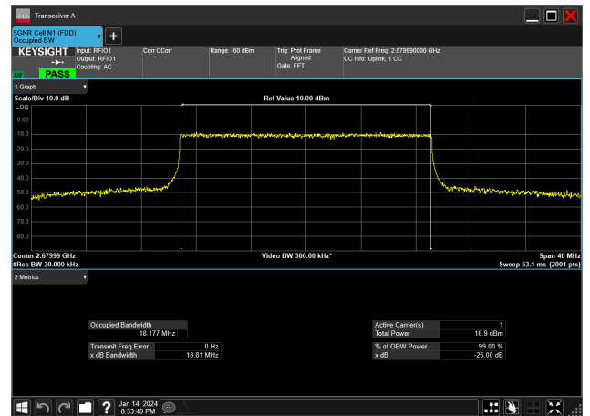
20MHz_30kHz_2679.99MHz_CP-OFDM 256 QAM_RB51@0&amp;18.177 MHz
