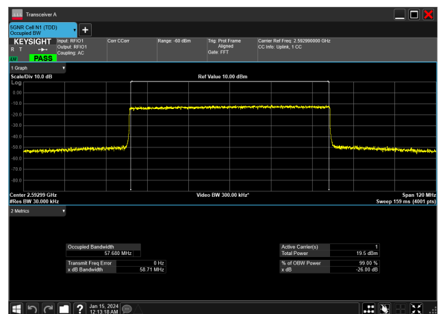
60MHz_30kHz_2592.99MHz_CP-OFDM 64 QAM_RB162@0&amp;57.680 MHz
