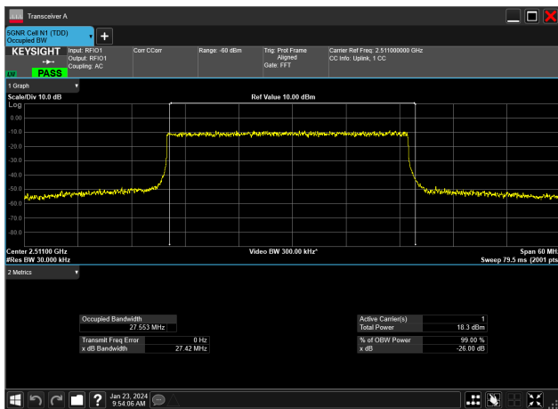
30MHz_30kHz_2511MHz_DFT-s-OFDM 256 QAM_RB75@0&amp;27.553 MHz
