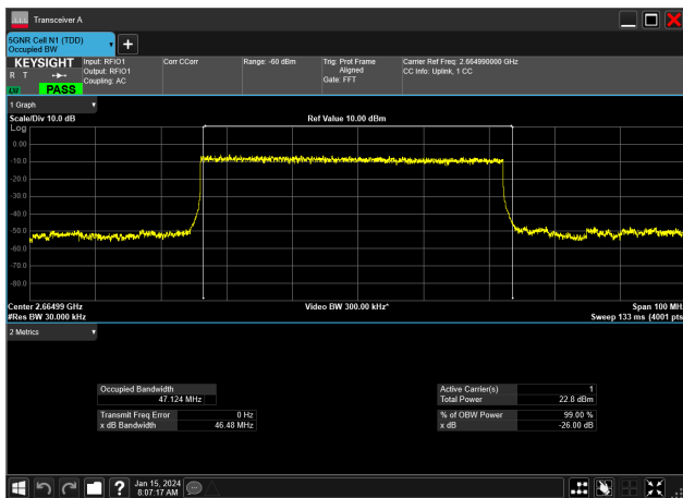
50MHz_30kHz_2664.99MHz_DFT-s-OFDM PI/2 BPSK_RB128@0&amp;47.124 MHz
