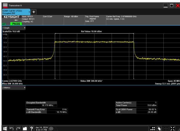
20MHz_30kHz_2679.99MHz_CP-OFDM 64 QAM_RB51@0&amp;18.179 MHz
