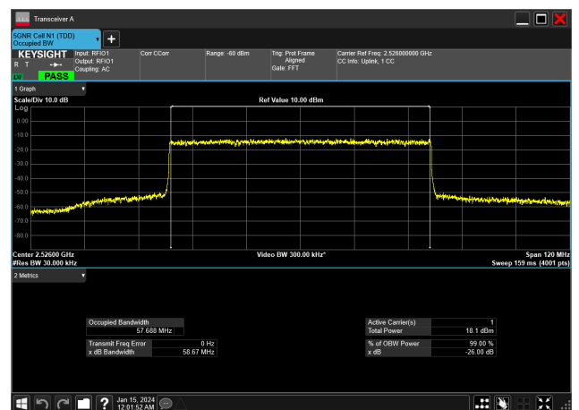
60MHz_30kHz_2526MHz_DFT-s-OFDM 256 QAM_RB162@0&amp;57.688 MHz
