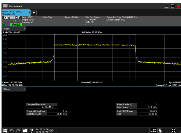
30MHz_30kHz_2674.98MHz_CP-OFDM 256 QAM_RB78@0&27.804 MHz
