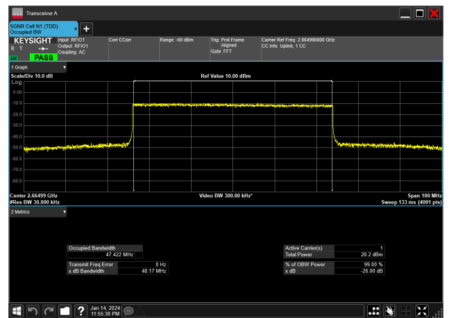
50MHz_30kHz_2664.99MHz_CP-OFDM 16 QAM_RB133@0&47.422 MHz
