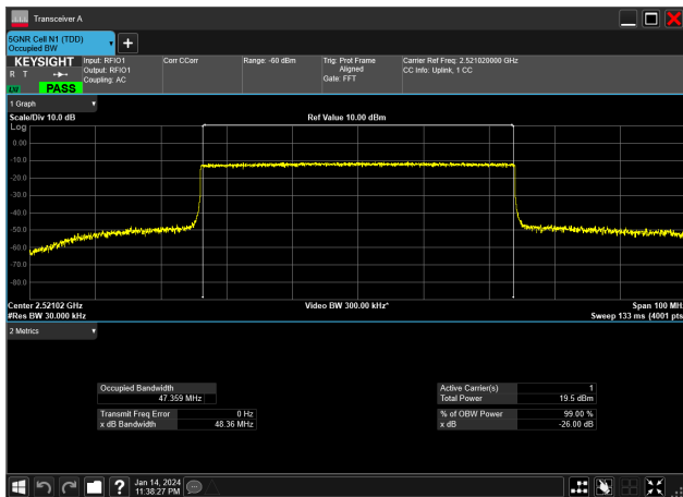
50MHz_30kHz_2521.02MHz_CP-OFDM QPSK_RB133@0&amp;47.359 MHz
