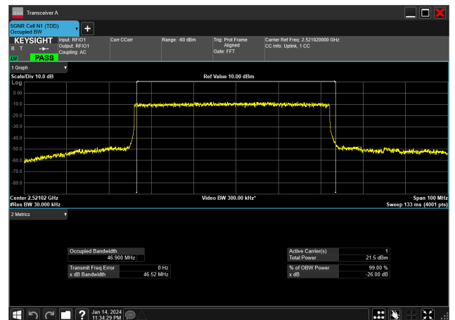
50MHz_30kHz_2521.02MHz_DFT-s-OFDM QPSK_RB128@0&amp;46.900 MHz
