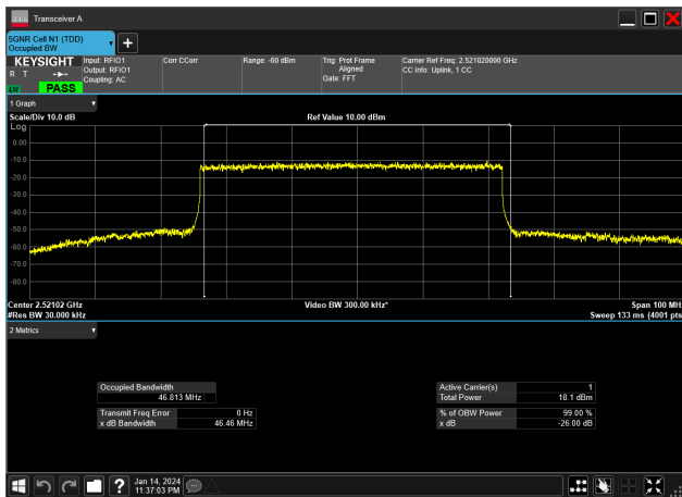
50MHz_30kHz_2521.02MHz_DFT-s-OFDM 256 QAM_RB128@0&amp;46.813 MHz
