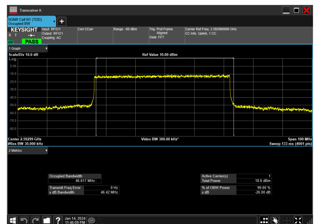
50MHz_30kHz_2592.99MHz_DFT-s-OFDM 256 QAM_RB128@0&amp;46.817 MHz
