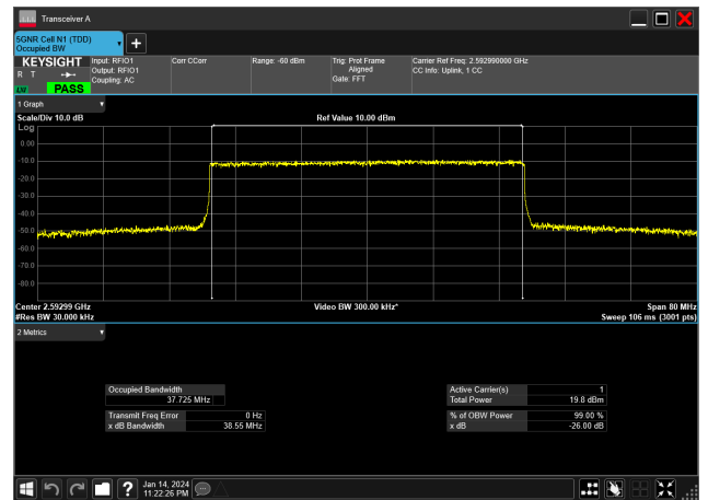
40MHz_30kHz_2592.99MHz_CP-OFDM 16 QAM_RB106@0&37.725 MHz
