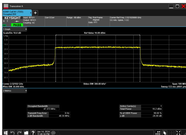
50MHz_30kHz_2521.02MHz_CP-OFDM 256 QAM_RB133@0&amp;47.373 MHz
