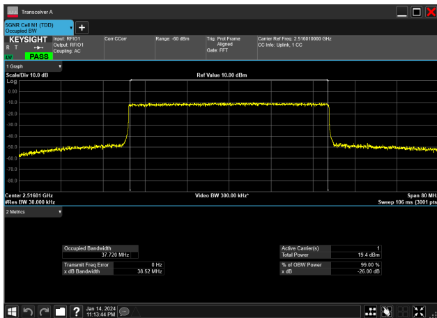
40MHz_30kHz_2516.01MHz_CP-OFDM 16 QAM_RB106@0&amp;37.720 MHz
