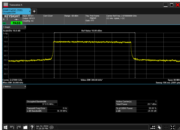
40MHz_30kHz_2670MHz_DFT-s-OFDM 64 QAM_RB100@0&amp;37.515 MHz
