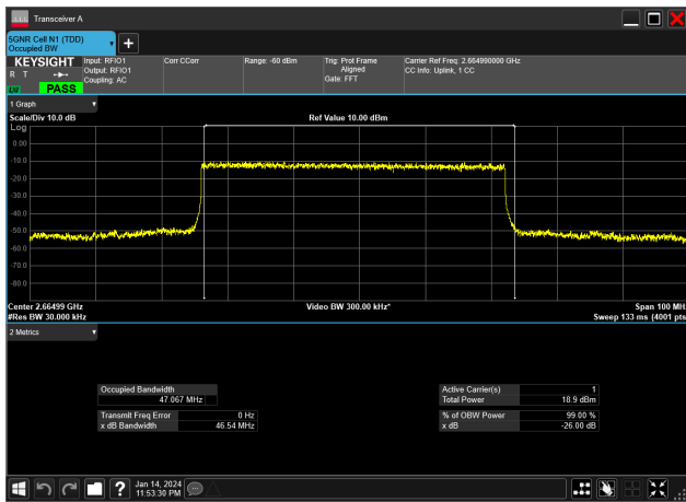
50MHz_30kHz_2664.99MHz_DFT-s-OFDM 256 QAM_RB128@0&amp;47.067 MHz
