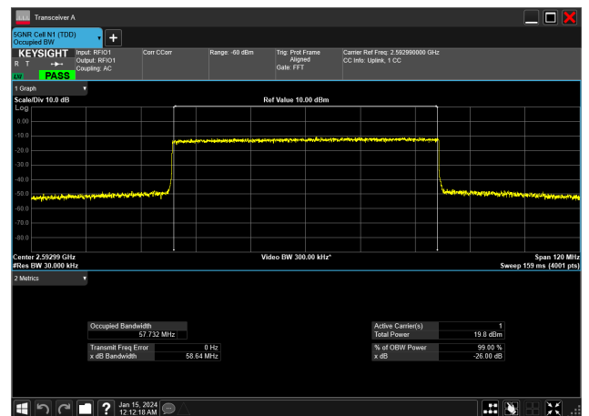
60MHz_30kHz_2592.99MHz_CP-OFDM 16 QAM_RB162@0&amp;57.732 MHz
