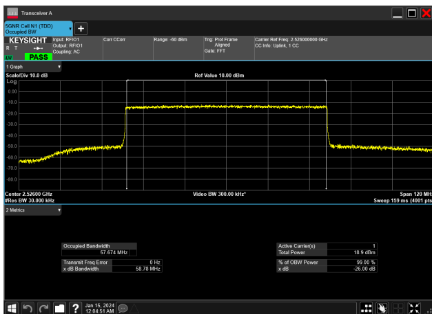
60MHz_30kHz_2526MHz_CP-OFDM 64 QAM_RB162@0&amp;57.674 MHz
