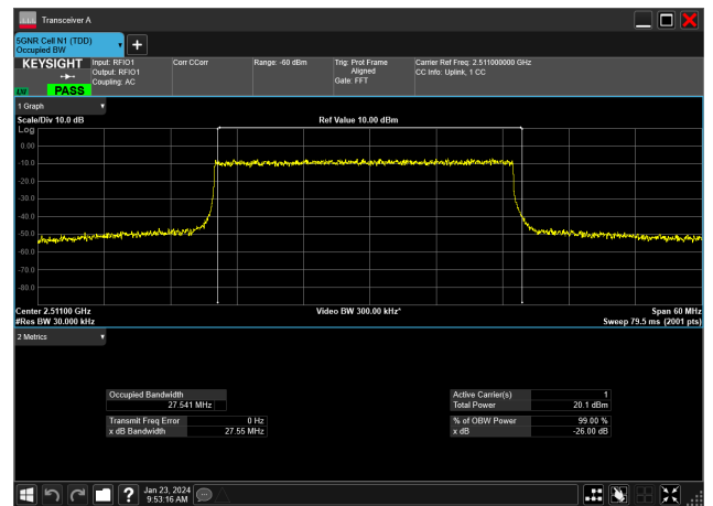
30MHz_30kHz_2511MHz_DFT-s-OFDM 64 QAM_RB75@0&amp;27.541 MHz
