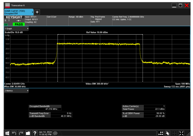
50MHz_30kHz_2664.99MHz_DFT-s-OFDM QPSK_RB128@0&amp;47.216 MHz
