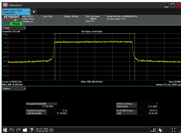
30MHz_30kHz_2592.99MHz_DFT-s-OFDM QPSK_RB75@0&27.499 MHz
