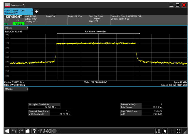
40MHz_30kHz_2592.99MHz_DFT-s-OFDM 64 QAM_RB100@0&amp;37.340 MHz
