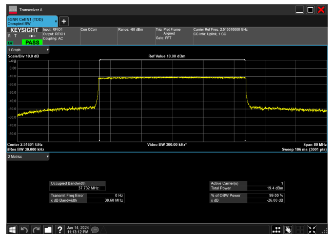
40MHz_30kHz_2516.01MHz_CP-OFDM QPSK_RB106@0&amp;37.732 MHz
