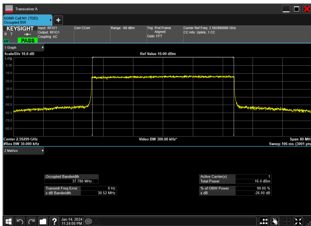
40MHz_30kHz_2592.99MHz_CP-OFDM 256 QAM_RB106@0&37.780 MHz
