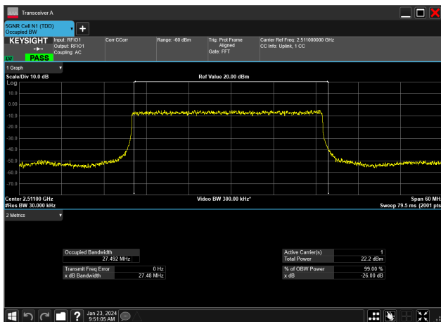
30MHz_30kHz_2511MHz_DFT-s-OFDM PI/2 BPSK_RB75@0&amp;27.492 MHz
