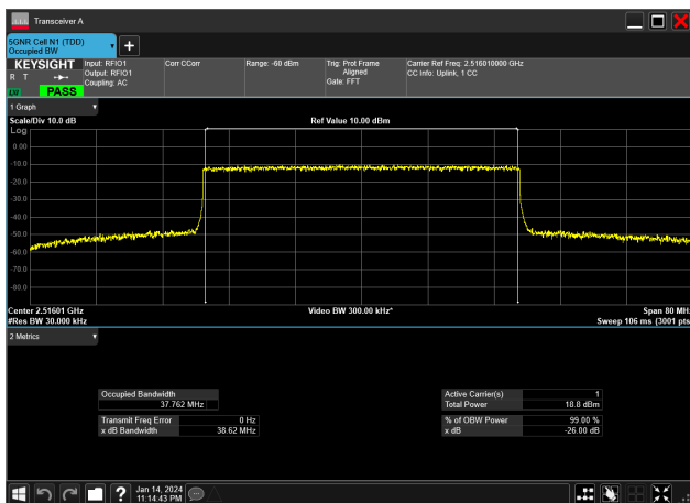
40MHz_30kHz_2516.01MHz_CP-OFDM 64 QAM_RB106@0&amp;37.762 MHz
