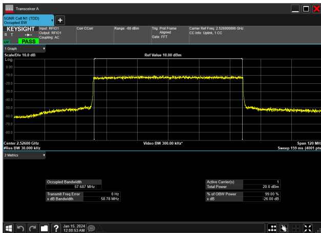
60MHz_30kHz_2526MHz_DFT-s-OFDM 64 QAM_RB162@0&amp;57.687 MHz
