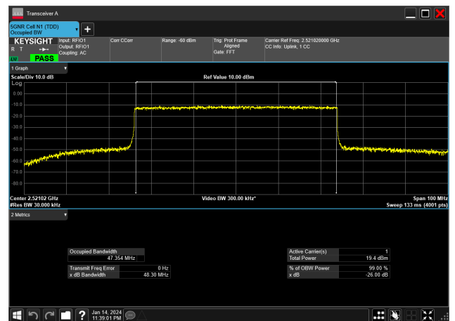
50MHz_30kHz_2521.02MHz_CP-OFDM 16 QAM_RB133@0&amp;47.354 MHz
