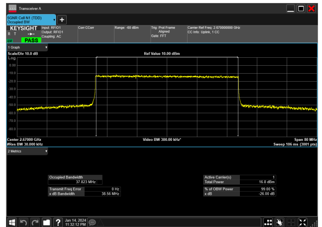
40MHz_30kHz_2670MHz_CP-OFDM 256 QAM_RB106@0&amp;37.823 MHz
