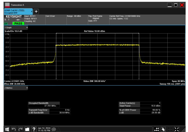
40MHz_30kHz_2516.01MHz_CP-OFDM 256 QAM_RB106@0&amp;37.781 MHz
