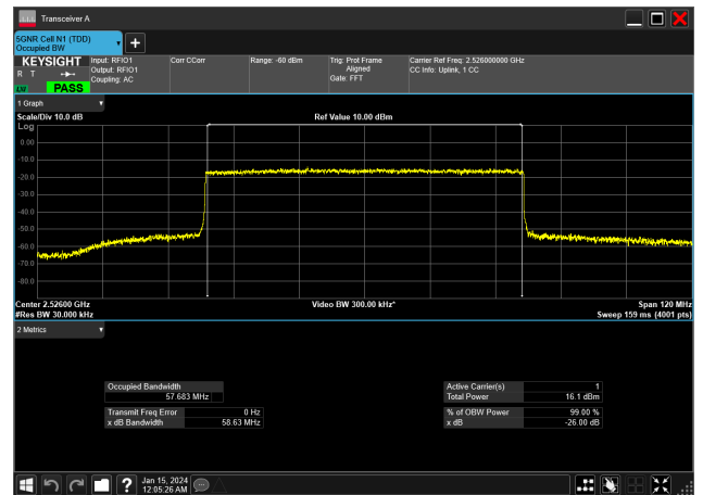
60MHz_30kHz_2526MHz_CP-OFDM 256 QAM_RB162@0&amp;57.683 MHz
