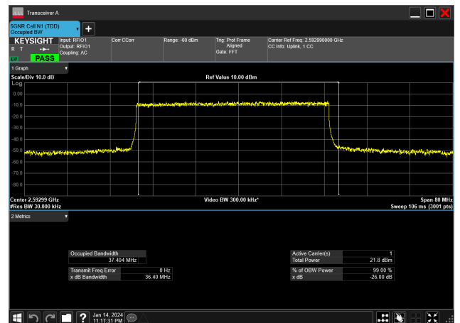
40MHz_30kHz_2592.99MHz_DFT-s-OFDM QPSK_RB100@0&amp;37.404 MHz
