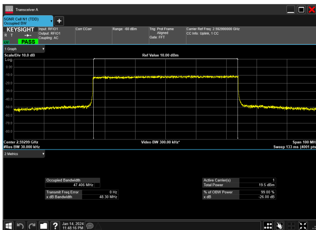
50MHz_30kHz_2592.99MHz_CP-OFDM 64 QAM_RB133@0&amp;47.406 MHz
