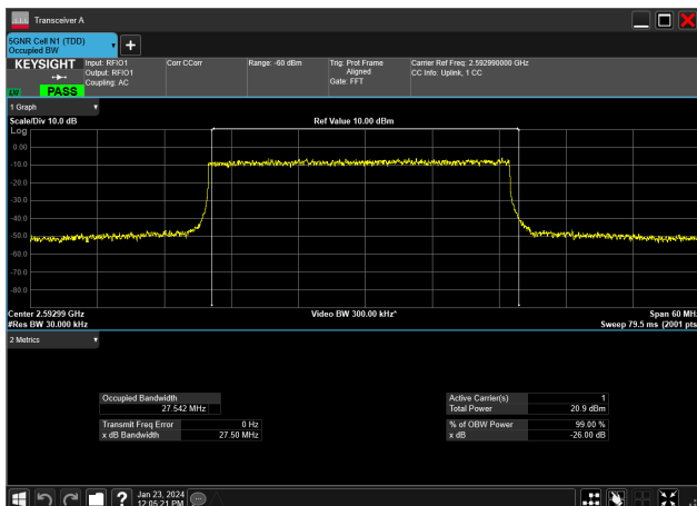
30MHz_30kHz_2592.99MHz_DFT-s-OFDM 16 QAM_RB75@0&amp;27.542 MHz
