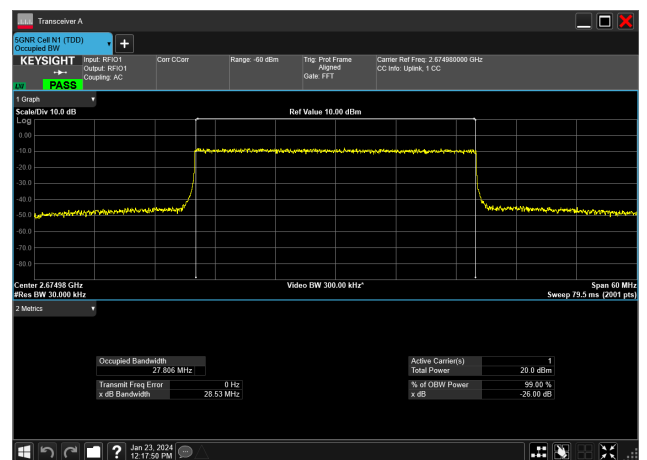
30MHz_30kHz_2674.98MHz_CP-OFDM 64 QAM_RB78@0&27.806 MHz
