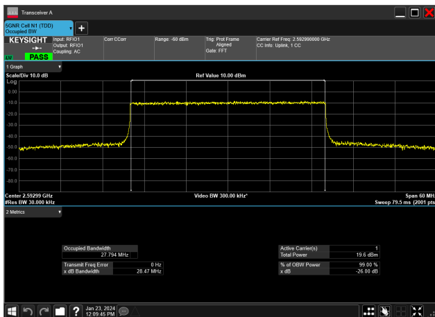
30MHz_30kHz_2592.99MHz_CP-OFDM 64 QAM_RB78@0&amp;27.794 MHz
