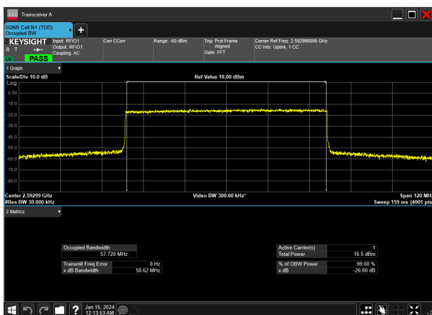
60MHz_30kHz_2592.99MHz_CP-OFDM 256 QAM_RB162@0&amp;57.720 MHz
