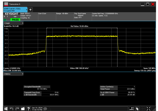
60MHz_30kHz_2526MHz_DFT-s-OFDM PI/2 BPSK_RB162@0&amp;57.725 MHz
