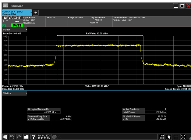
50MHz_30kHz_2592.99MHz_DFT-s-OFDM QPSK_RB128@0&46.971 MHz
