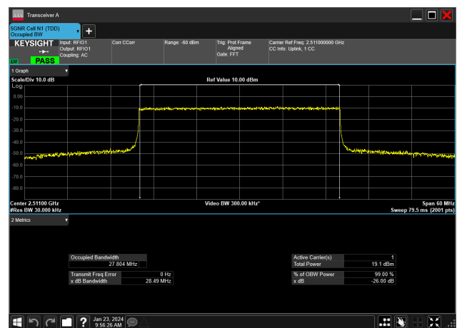
30MHz_30kHz_2511MHz_CP-OFDM 64 QAM_RB78@0&27.804 MHz
