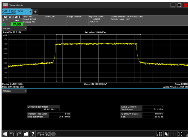
40MHz_30kHz_2516.01MHz_DFT-s-OFDM QPSK_RB100@0&37.443 MHz
