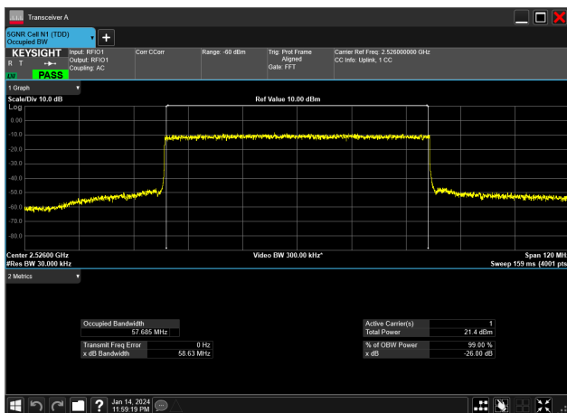
60MHz_30kHz_2526MHz_DFT-s-OFDM QPSK_RB162@0&amp;57.685 MHz
