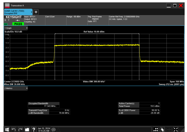
80MHz_30kHz_2536.02MHz_CP-OFDM 16 QAM_RB217@0&77.343 MHz
