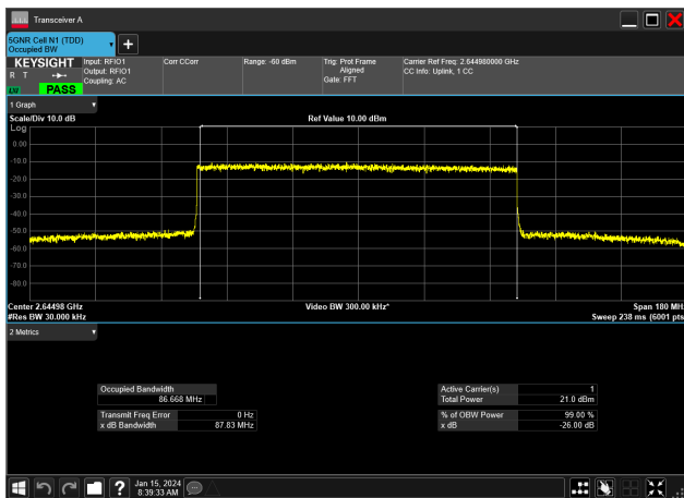
90MHz_30kHz_2644.98MHz_DFT-s-OFDM 16 QAM_RB243@0&amp;86.668 MHz
