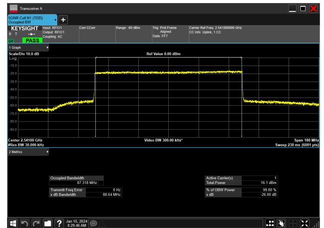
90MHz_30kHz_2541MHz_CP-OFDM 256 QAM_RB245@0&amp;87.318 MHz
