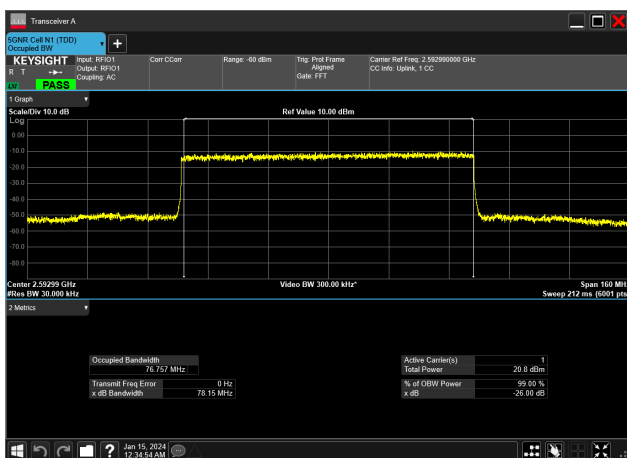
80MHz_30kHz_2592.99MHz_DFT-s-OFDM 16 QAM_RB216@0&amp;76.757 MHz
