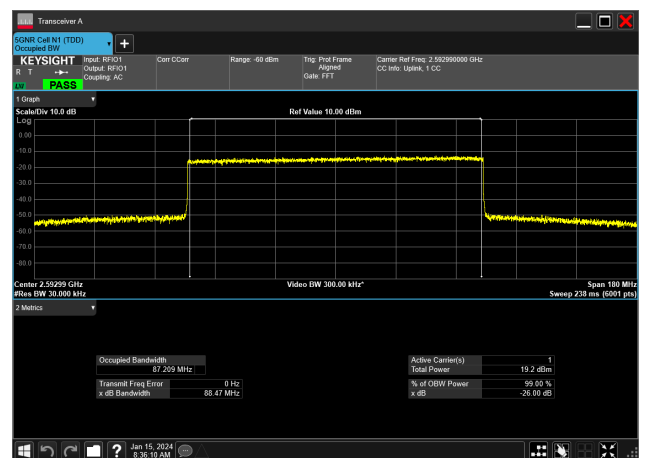
90MHz_30kHz_2592.99MHz_CP-OFDM 64 QAM_RB245@0&amp;87.209 MHz
