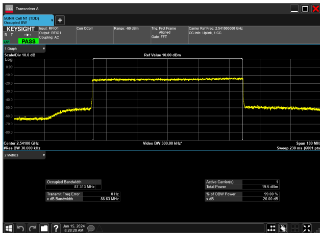
90MHz_30kHz_2541MHz_CP-OFDM 16 QAM_RB245@0&amp;87.313 MHz
