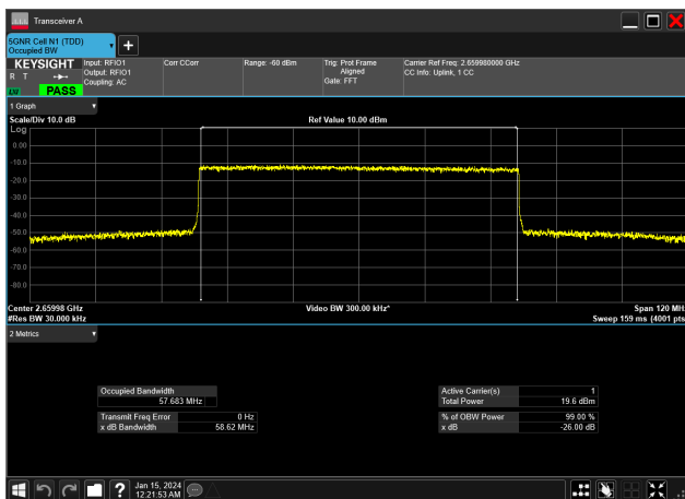
60MHz_30kHz_2659.98MHz_CP-OFDM 64 QAM_RB162@0&amp;57.683 MHz
