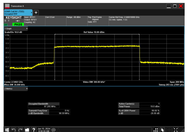
100MHz_30kHz_2546.01MHz_CP-OFDM 64 QAM_RB273@0&97.205 MHz
