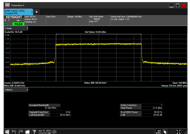
60MHz_30kHz_2592.99MHz_DFT-s-OFDM QPSK_RB162@0&amp;57.684 MHz
