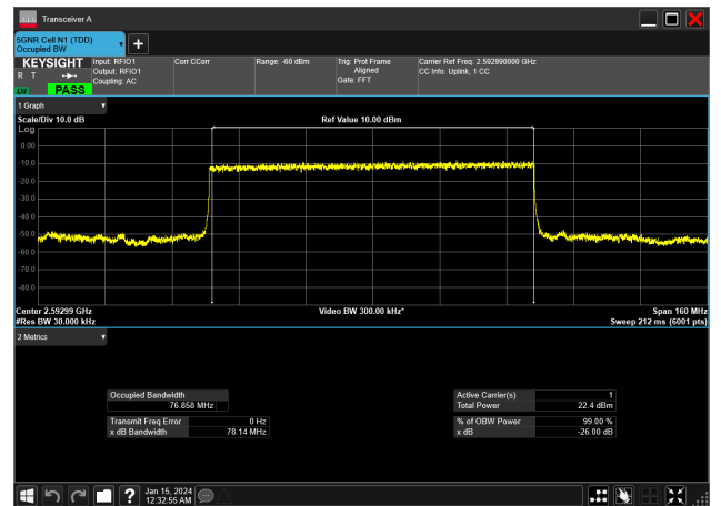
80MHz_30kHz_2592.99MHz_DFT-s-OFDM PI/2 BPSK_RB216@0&76.858 MHz
