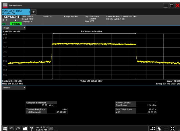
90MHz_30kHz_2644.98MHz_DFT-s-OFDM QPSK_RB243@0&86.591 MHz
