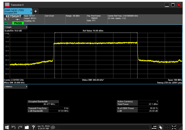
90MHz_30kHz_2541MHz_DFT-s-OFDM PI/2 BPSK_RB243@0&amp;86.477 MHz
