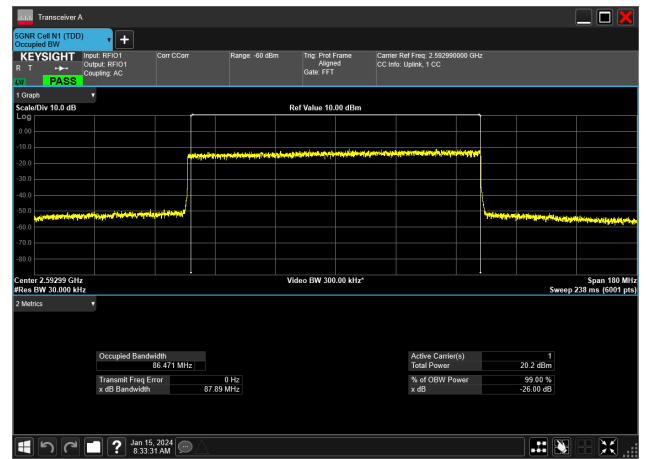
90MHz_30kHz_2592.99MHz_DFT-s-OFDM 64 QAM_RB243@0&86.471 MHz
