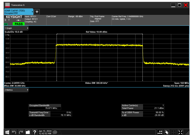
80MHz_30kHz_2649.99MHz_DFT-s-OFDM 16 QAM_RB216@0&amp;76.871 MHz
