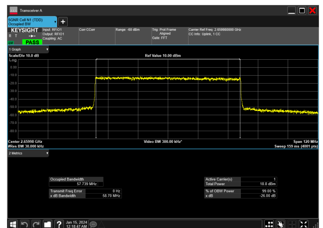
60MHz_30kHz_2659.98MHz_DFT-s-OFDM 256 QAM_RB162@0&amp;57.739 MHz
