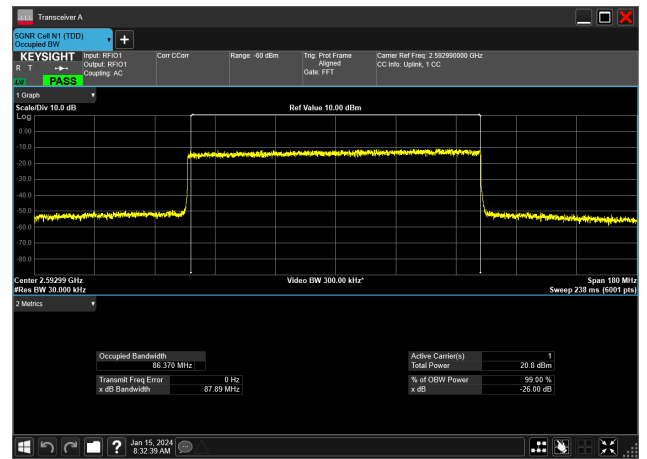
90MHz_30kHz_2592.99MHz_DFT-s-OFDM 16 QAM_RB243@0&86.370 MHz
