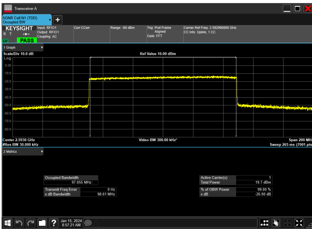
100MHz_30kHz_2592.99MHz_CP-OFDM 16 QAM_RB273@0&97.055 MHz
