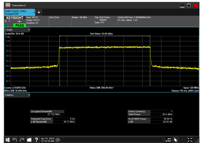
60MHz_30kHz_2592.99MHz_DFT-s-OFDM 64 QAM_RB162@0&amp;57.722 MHz
