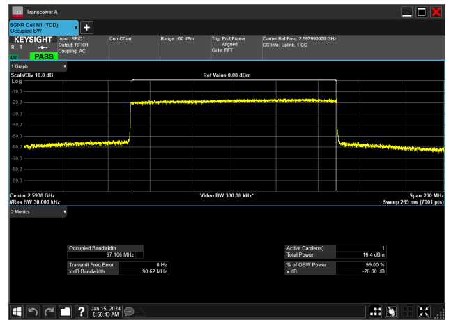
100MHz_30kHz_2592.99MHz_CP-OFDM 256 QAM_RB273@0&97.106 MHz
