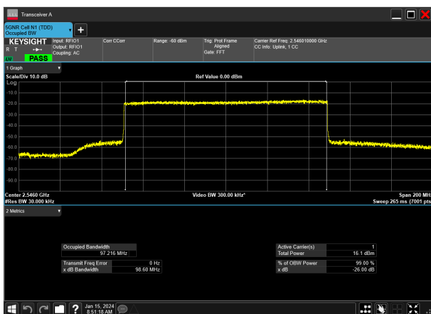
100MHz_30kHz_2546.01MHz_CP-OFDM 256 QAM_RB273@0&97.216 MHz
