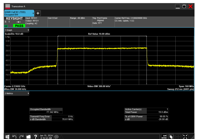
80MHz_30kHz_2536.02MHz_CP-OFDM 64 QAM_RB217@0&77.342 MHz
