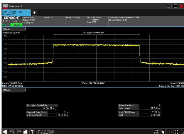
60MHz_30kHz_2659.98MHz_DFT-s-OFDM 16 QAM_RB162@0&amp;57.727 MHz
