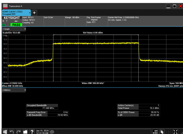
80MHz_30kHz_2536.02MHz_CP-OFDM 256 QAM_RB217@0&77.348 MHz
