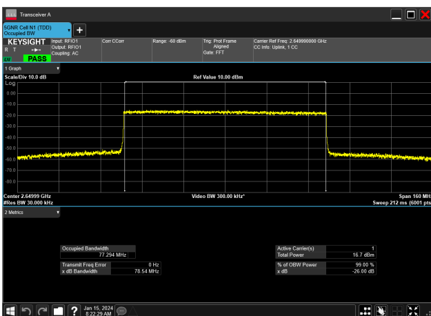
80MHz_30kHz_2649.99MHz_CP-OFDM 256 QAM_RB217@0&77.294 MHz
