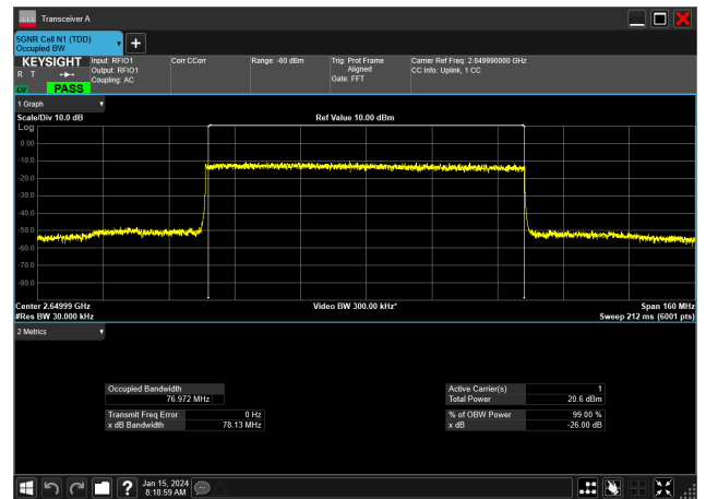
80MHz_30kHz_2649.99MHz_DFT-s-OFDM 64 QAM_RB216@0&amp;76.972 MHz
