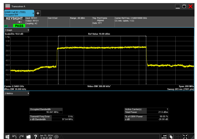
100MHz_30kHz_2546.01MHz_DFT-s-OFDM QPSK_RB270@0&amp;95.841 MHz
