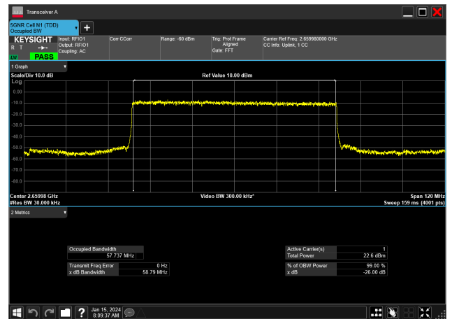
60MHz_30kHz_2659.98MHz_DFT-s-OFDM 16 BPSK_RB162@0&57.737 MHz
