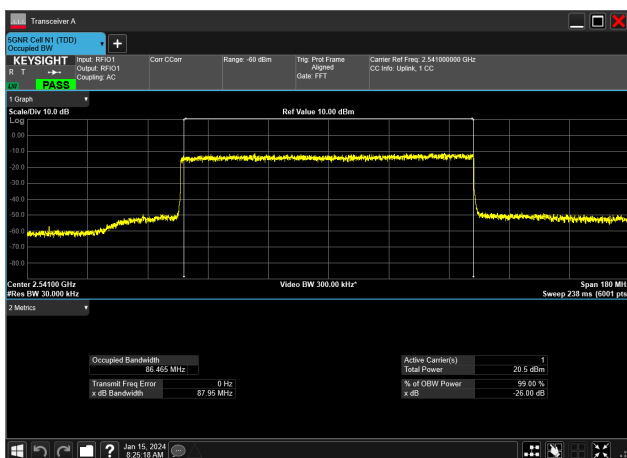
90MHz_30kHz_2541MHz_DFT-s-OFDM 16 QAM_RB243@0&amp;86.465 MHz
