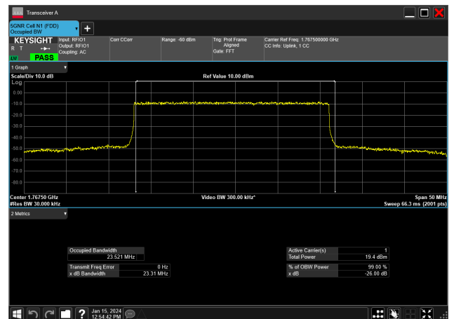
25MHz_15kHz_1767.5MHz_DFT-s-OFDM 256 QAM_RB128@0&amp;23.521 MHz
