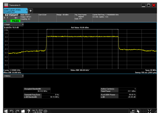
40MHz_15kHz_1745MHz_DFT-s-OFDM QPSK_RB216@0&amp;38.532 MHz
