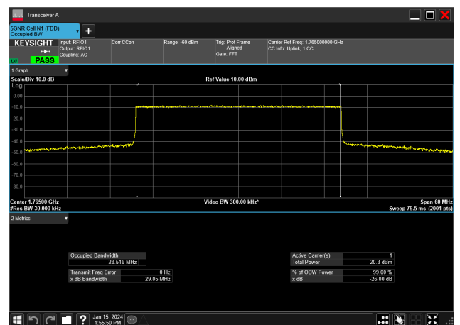
30MHz_15kHz_1765MHz_CP-OFDM 64 QAM_RB160@0&amp;28.516 MHz
