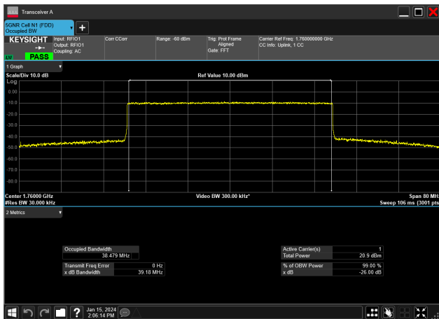
40MHz_15kHz_1760MHz_CP-OFDM 16 QAM_RB216@0&amp;38.479 MHz
