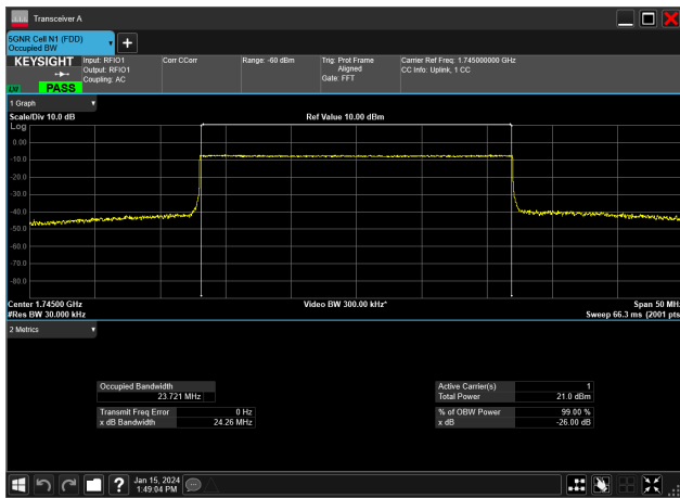
25MHz_15kHz_1745MHz_CP-OFDM QPSK_RB133@0&amp;23.721 MHz
