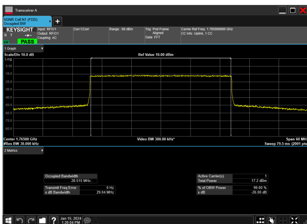
30MHz_15kHz_1765MHz_CP-OFDM 256 QAM_RB160@0&amp;28.515 MHz
