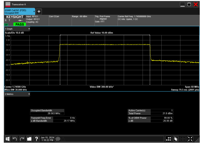
30MHz_15kHz_1745MHz_CP-OFDM QPSK_RB160@0&amp;28.563 MHz
