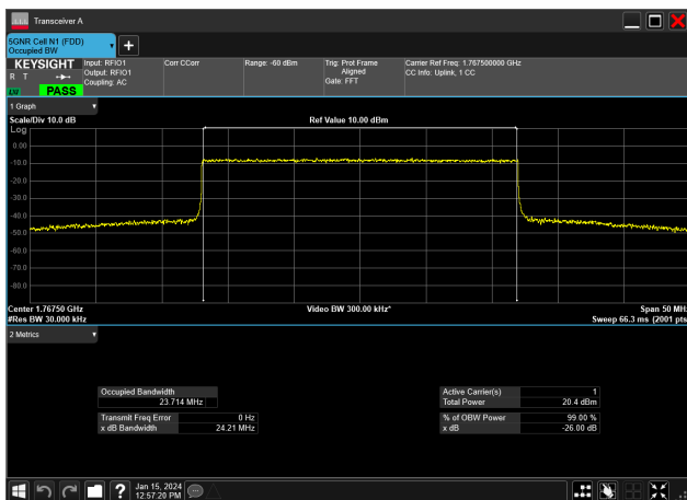
25MHz_15kHz_1767.5MHz_CP-OFDM 64 QAM_RB133@0&amp;23.714 MHz
