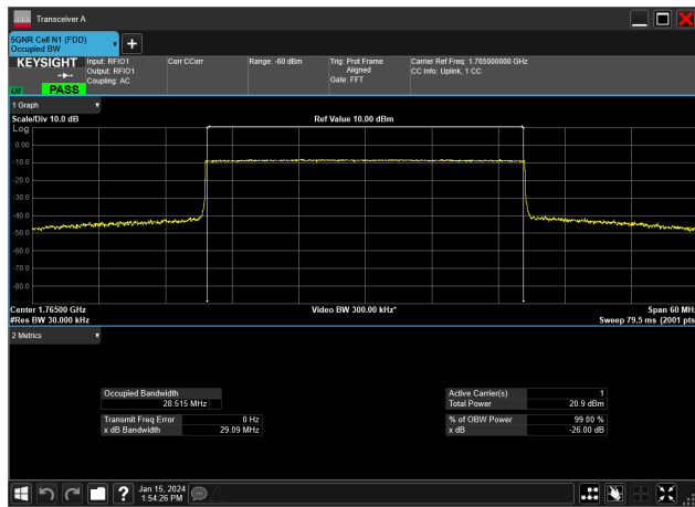
30MHz_15kHz_1765MHz_CP-OFDM QPSK_RB160@0&amp;28.515 MHz
