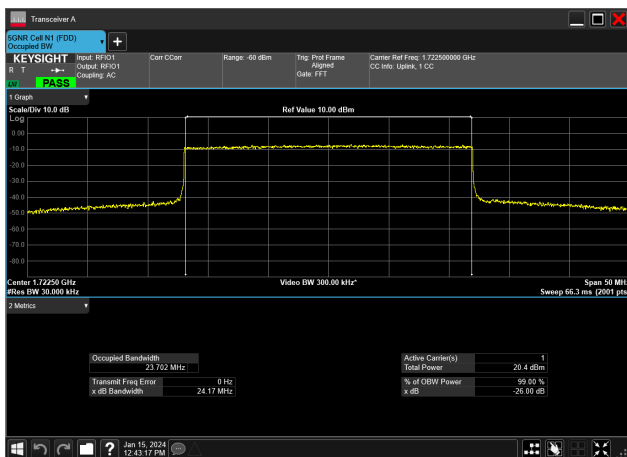
25MHz_15kHz_1722.5MHz_CP-OFDM 64 QAM_RB133@0&amp;23.702 MHz
