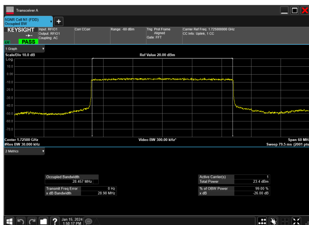
30MHz_15kHz_1725MHz_DFT-s-OFDM PI/2 BPSK_RB160@0&amp;28.457 MHz
