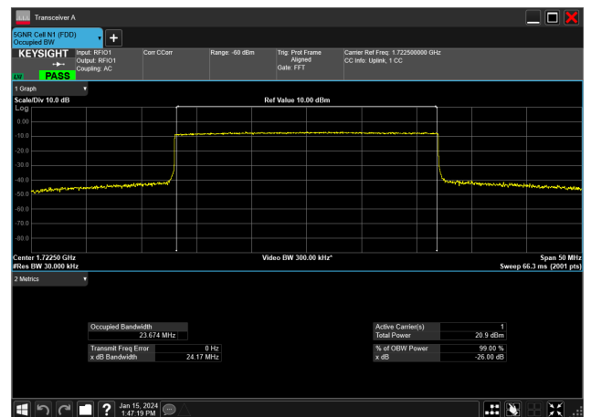
25MHz_15kHz_1722.5MHz_CP-OFDM QPSK_RB133@0&amp;23.674 MHz
