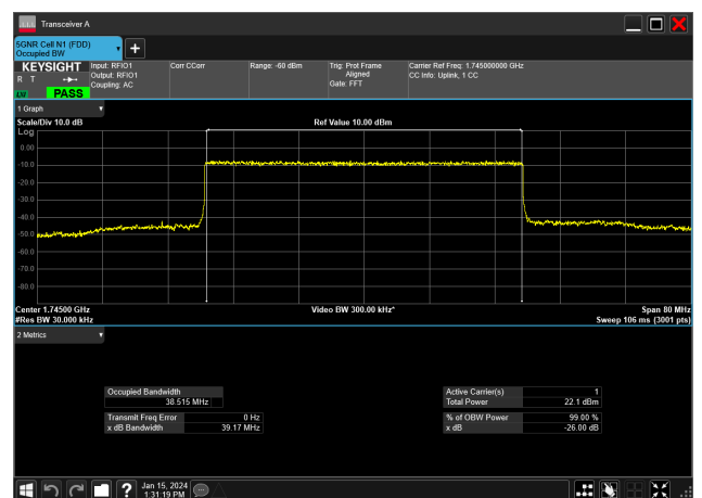
40MHz_15kHz_1745MHz_DFT-s-OFDM 16 QAM_RB216@0&amp;38.515 MHz
