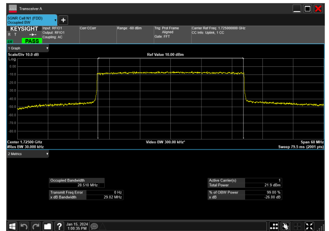
30MHz_15kHz_1725MHz_DFT-s-OFDM 16 QAM_RB160@0&amp;28.510 MHz
