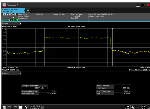
25MHz_15kHz_1745MHz_DFT-s-OFDM PI/2 BPSK_RB128@0&amp;23.561 MHz
