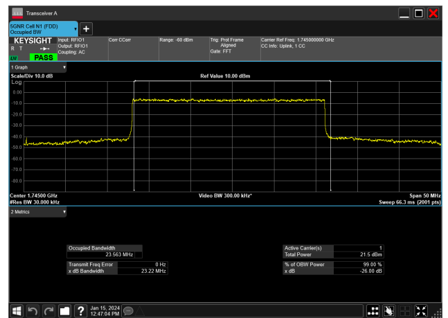
25MHz_15kHz_1745MHz_DFT-s-OFDM 64 QAM_RB128@0&amp;23.563 MHz
