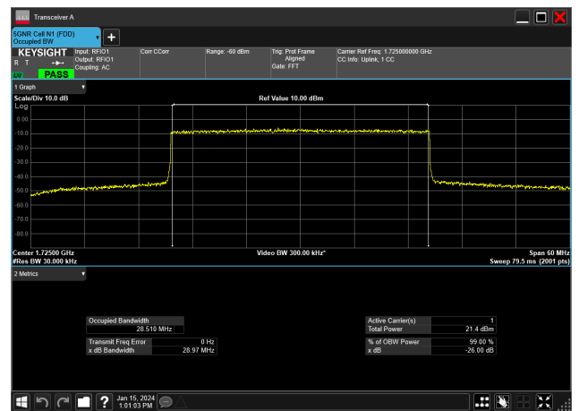
30MHz_15kHz_1725MHz_DFT-s-OFDM 64 QAM_RB160@0&amp;28.510 MHz
