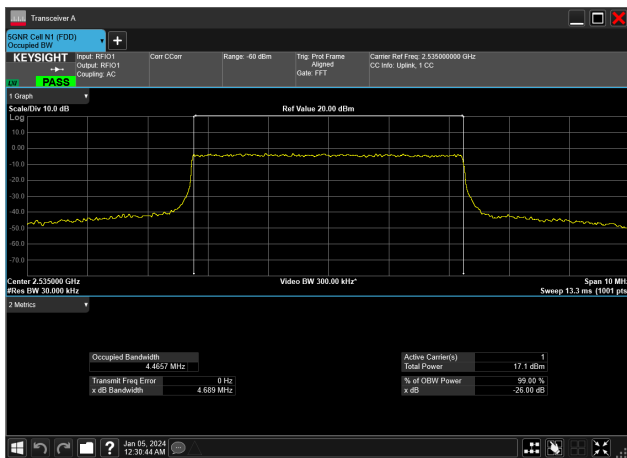
5MHz_15kHz_2535MHz_CP-OFDM 256 QAM_RB25@0&amp;4.466 MHz
