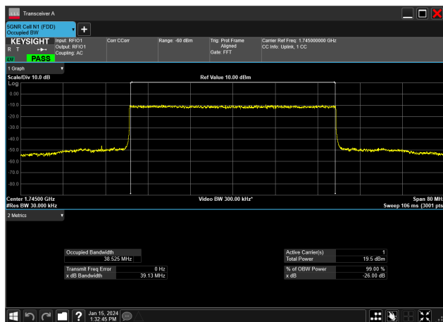
40MHz_15kHz_1745MHz_DFT-s-OFDM 256 QAM_RB216@0&amp;38.525 MHz
