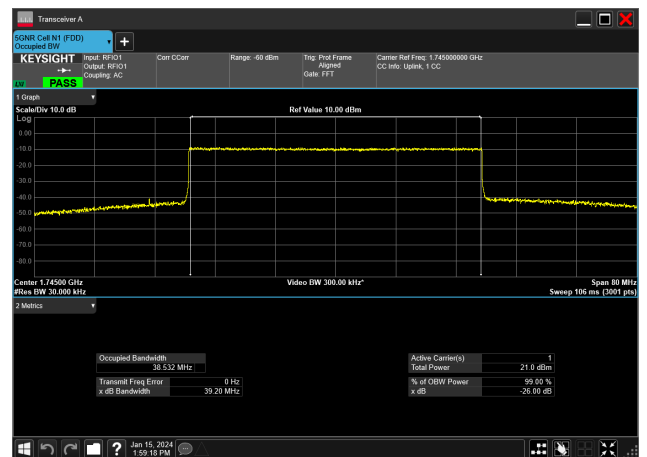
40MHz_15kHz_1745MHz_CP-OFDM 16 QAM_RB216@0&amp;38.532 MHz
