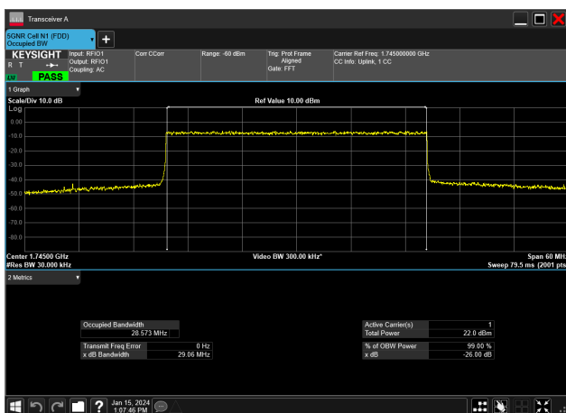
30MHz_15kHz_1745MHz_DFT-s-OFDM 16 QAM_RB160@0&amp;28.573 MHz
