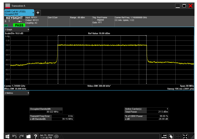
40MHz_15kHz_1745MHz_DFT-s-OFDM 64 QAM_RB216@0&amp;38.522 MHz
