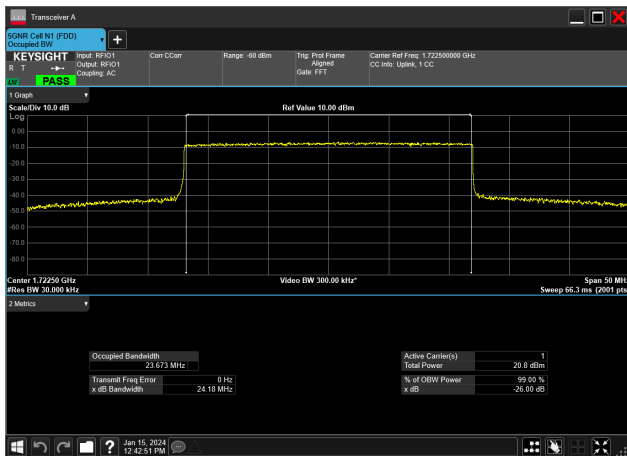
25MHz_15kHz_1722.5MHz_CP-OFDM 16 QAM_RB133@0&amp;23.673 MHz
