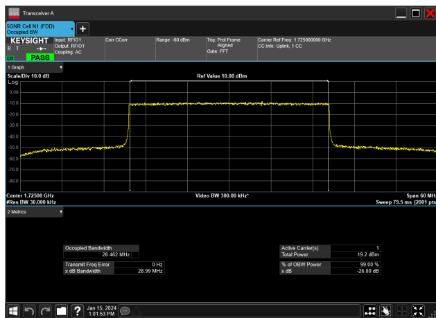
30MHz_15kHz_1725MHz_DFT-s-OFDM 256 QAM_RB160@0&amp;28.462 MHz
