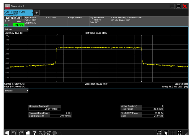
30MHz_15kHz_1765MHz_DFT-s-OFDM QPSK_RB160@0&amp;28.507 MHz
