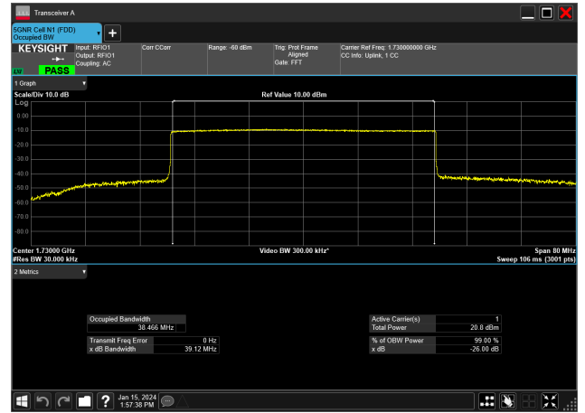
40MHz_15kHz_1730MHz_CP-OFDM QPSK_RB216@0&amp;38.466 MHz
