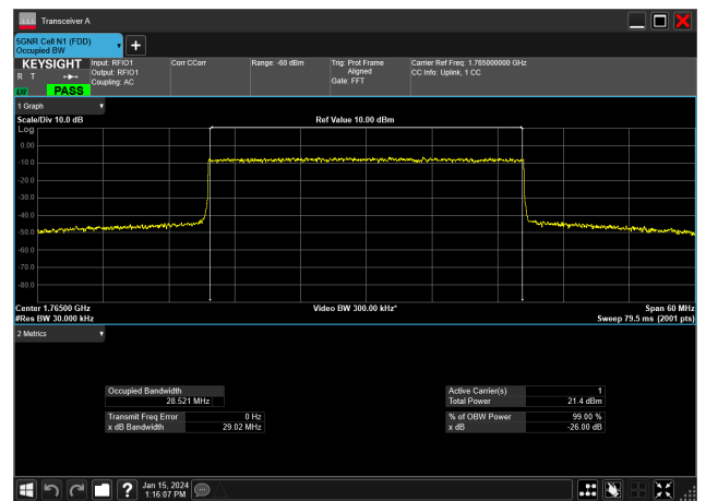
30MHz_15kHz_1765MHz_DFT-s-OFDM 64 QAM_RB160@0&amp;28.521 MHz
