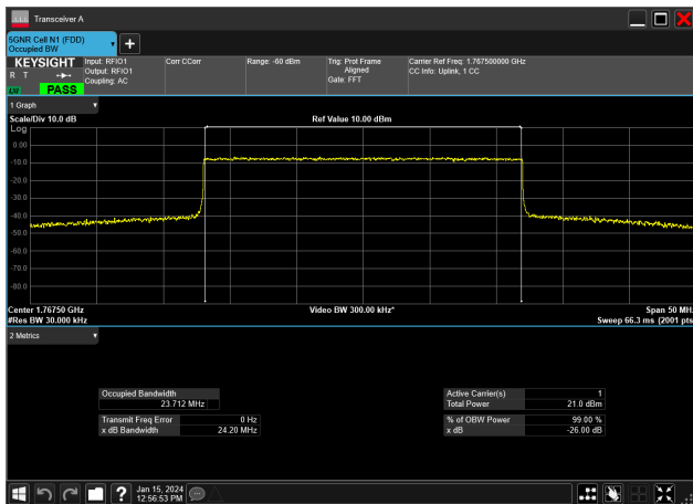
25MHz_15kHz_1767.5MHz_CP-OFDM 16 QAM_RB133@0&amp;23.712 MHz
