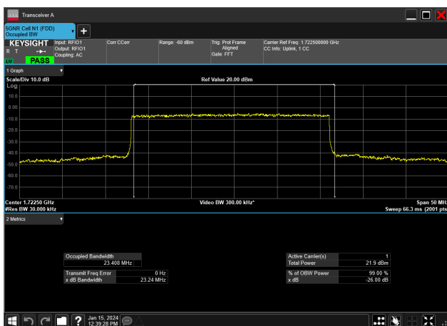
25MHz_15kHz_1722.5MHz_DFT-s-OFDM 16 QAM_RB128@0&amp;23.408 MHz
