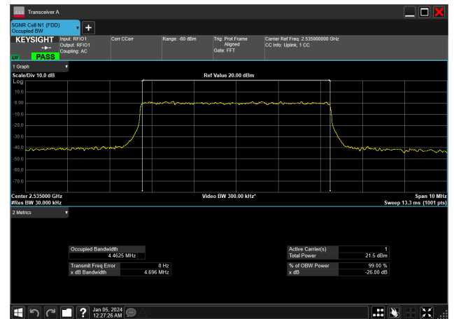
5MHz_15kHz_2535MHz_DFT-s-OFDM 16 QAM_RB25@0&amp;4.463 MHz
