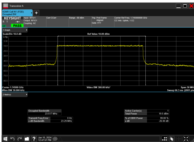
25MHz_15kHz_1745MHz_DFT-s-OFDM 256 QAM_RB128@0&amp;23.517 MHz
