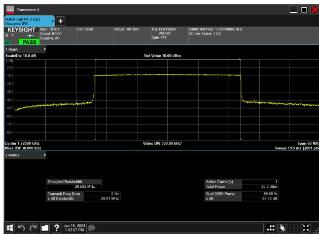
30MHz_15kHz_1725MHz_CP-OFDM QPSK_RB160@0&amp;28.502 MHz
