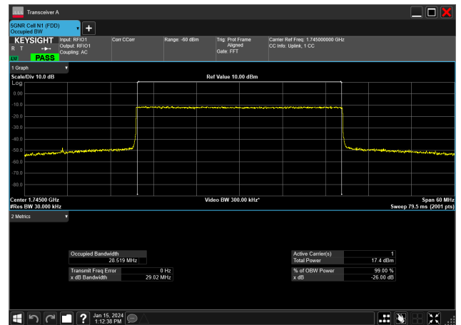
30MHz_15kHz_1745MHz_CP-OFDM 256 QAM_RB160@0&amp;28.519 MHz
