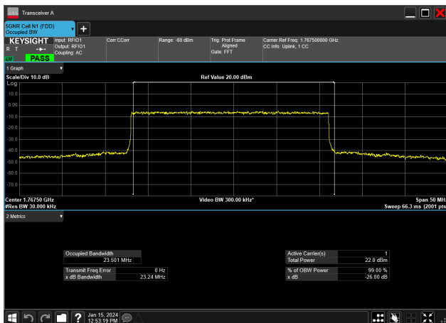
25MHz_15kHz_1767.5MHz_DFT-s-OFDM 16 QAM_RB128@0&amp;23.501 MHz
