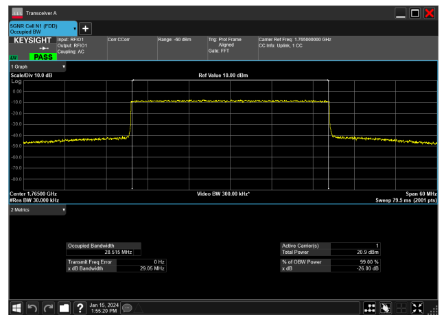
30MHz_15kHz_1765MHz_CP-OFDM 16 QAM_RB160@0&amp;28.515 MHz
