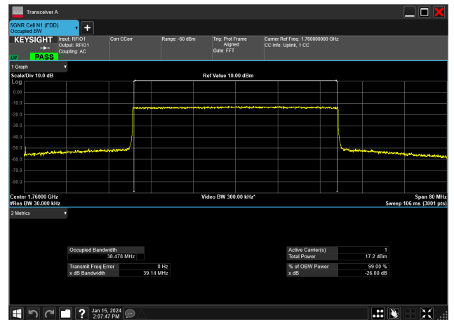
40MHz_15kHz_1760MHz_CP-OFDM 256 QAM_RB216@0&amp;38.478 MHz
