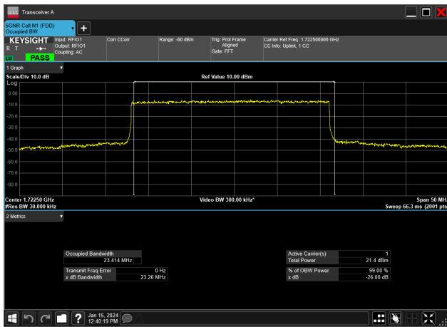
25MHz_15kHz_1722.5MHz_DFT-s-OFDM 64 QAM_RB128@0&23.414 MHz
