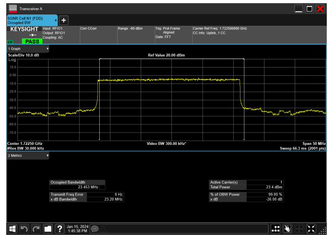
25MHz_15kHz_1722.5MHz_DFT-s-OFDM PI/2 BPSK_RB128@0&23.453 MHz
