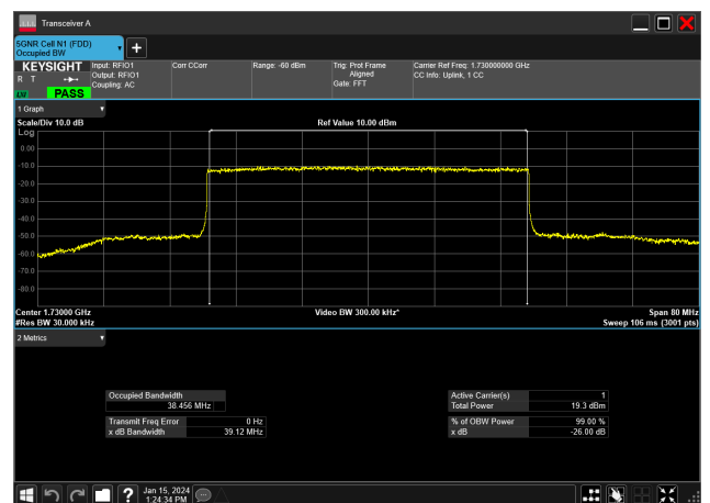
40MHz_15kHz_1730MHz_DFT-s-OFDM 256 QAM_RB216@0&amp;38.456 MHz
