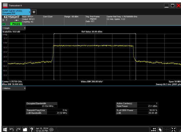
25MHz_15kHz_1767.5MHz_DFT-s-OFDM QPSK_RB128@0&23.554 MHz
