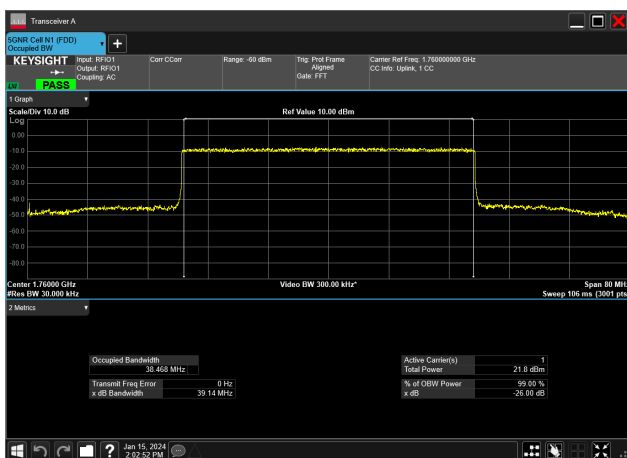
40MHz_15kHz_1760MHz_DFT-s-OFDM 16 QAM_RB216@0&amp;38.468 MHz
