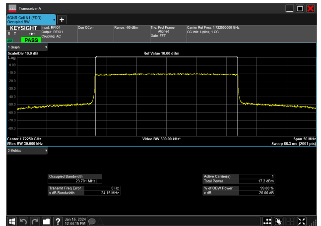
25MHz_15kHz_1722.5MHz_CP-OFDM 256 QAM_RB133@0&amp;23.701 MHz
