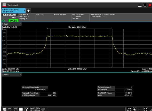
5MHz_15kHz_2535MHz_DFT-s-OFDM PI/2 BPSK_RB25@0&amp;4.464 MHz
