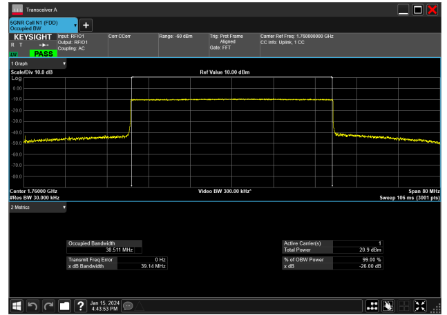
40MHz_15kHz_1760MHz_CP-OFDM QPSK_RB216@0&amp;38.511 MHz
