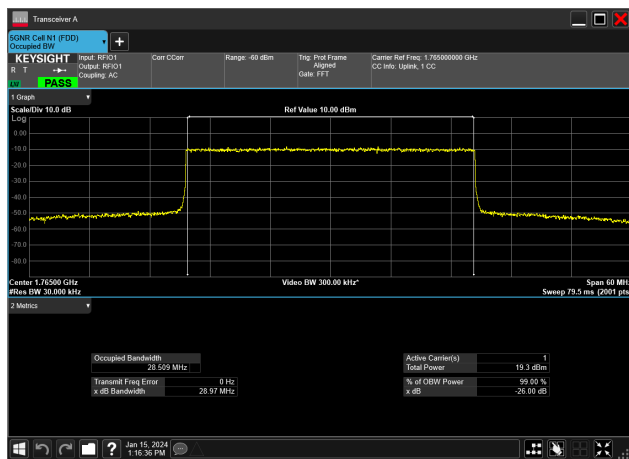
30MHz_15kHz_1765MHz_DFT-s-OFDM 256 QAM_RB160@0&amp;28.509 MHz
