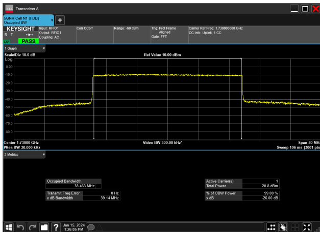
40MHz_15kHz_1730MHz_CP-OFDM 16 QAM_RB216@0&amp;38.463 MHz
