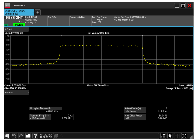
5MHz_15kHz_2535MHz_CP-OFDM 64 QAM_RB25@0&amp;4.464 MHz
