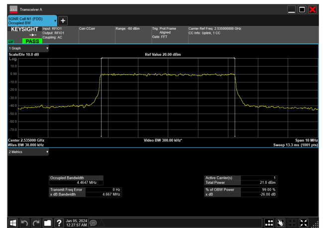
5MHz_15kHz_2535MHz_DFT-s-OFDM 64 QAM_RB25@0&amp;4.465 MHz
