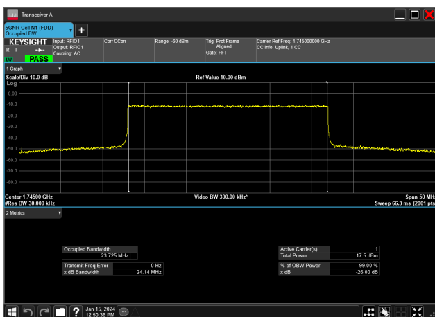
25MHz_15kHz_1745MHz_CP-OFDM 256 QAM_RB133@0&23.725 MHz
