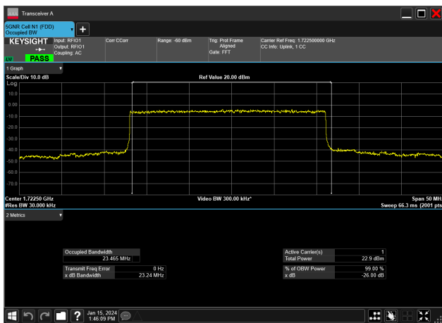
25MHz_15kHz_1722.5MHz_DFT-s-OFDM QPSK_RB128@0&23.465 MHz
