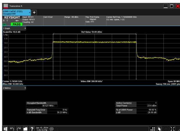
40MHz_15kHz_1745MHz_DFT-s-OFDM PI/2 BPSK_RB216@0&amp;38.521 MHz
