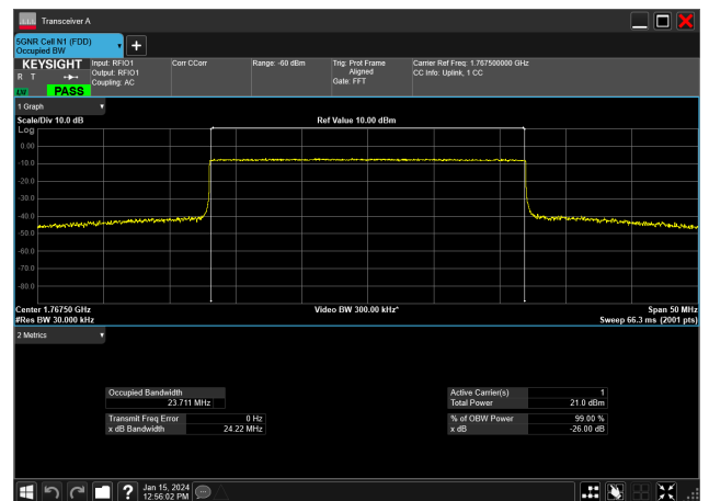
25MHz_15kHz_1767.5MHz_CP-OFDM QPSK_RB133@0&amp;23.711 MHz
