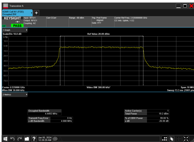
5MHz_15kHz_2535MHz_DFT-s-OFDM 256 QAM_RB25@0&amp;4.449 MHz
