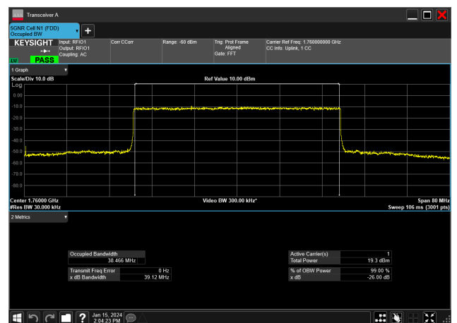
40MHz_15kHz_1760MHz_DFT-s-OFDM 256 QAM_RB216@0&amp;38.466 MHz
