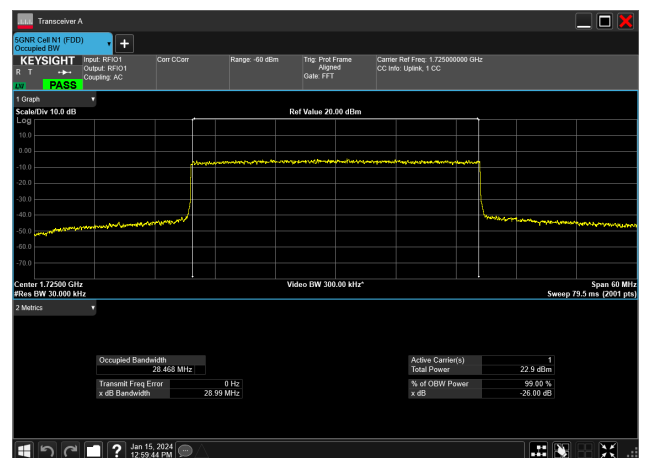
30MHz_15kHz_1725MHz_DFT-s-OFDM QPSK_RB160@0&amp;28.468 MHz
