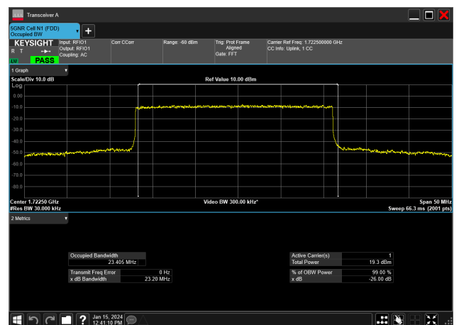
25MHz_15kHz_1722.5MHz_DFT-s-OFDM 256 QAM_RB128@0&amp;23.405 MHz
