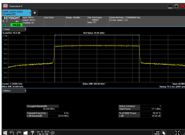
30MHz_15kHz_1725MHz_CP-OFDM 256 QAM_RB160@0&28.500 MHz
