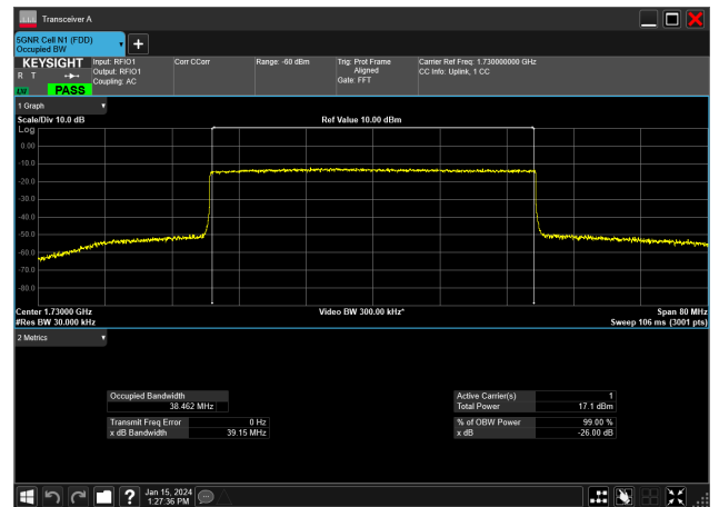
40MHz_15kHz_1730MHz_CP-OFDM 256 QAM_RB216@0&amp;38.462 MHz
