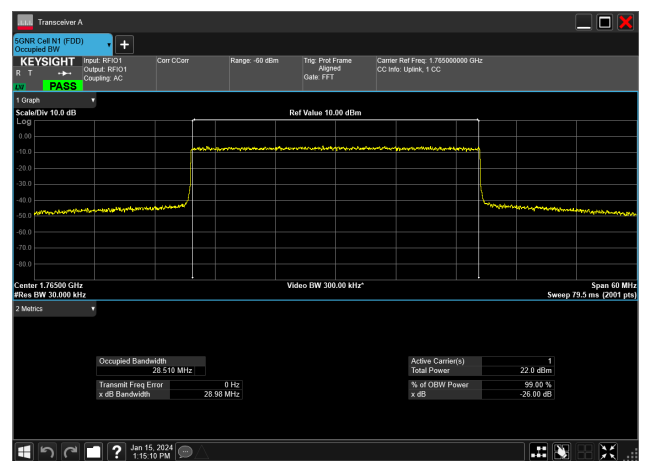
30MHz_15kHz_1765MHz_DFT-s-OFDM 16 QAM_RB160@0&amp;28.510 MHz
