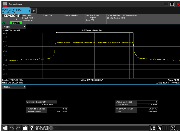
5MHz_15kHz_2502.5MHz_CP-OFDM 16 QAM_RB25@0&amp;4.461 MHz
