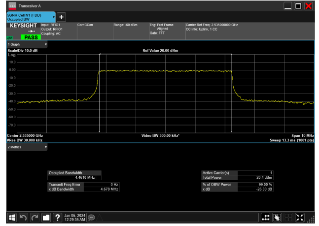
5MHz_15kHz_2535MHz_CP-OFDM 16 QAM_RB25@0&amp;4.461 MHz
