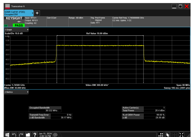
40MHz_15kHz_1745MHz_CP-OFDM 64 QAM_RB216@0&amp;38.532 MHz
