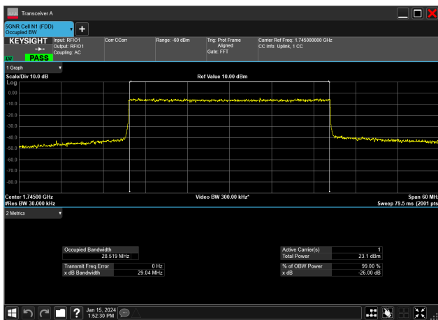
30MHz_15kHz_1745MHz_DFT-s-OFDM QPSK_RB160@0&amp;28.519 MHz
