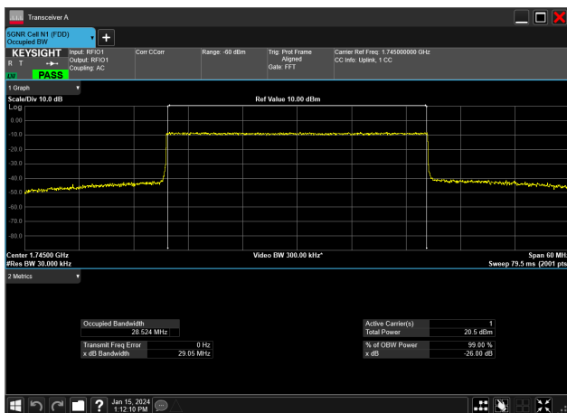
30MHz_15kHz_1745MHz_CP-OFDM 64 QAM_RB160@0&amp;28.524 MHz
