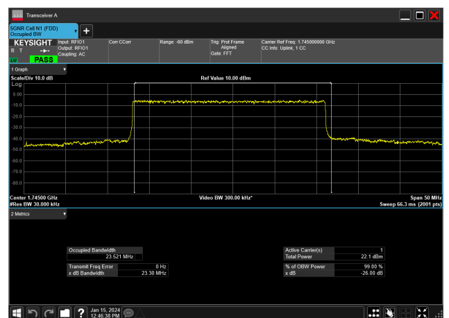
25MHz_15kHz_1745MHz_DFT-s-OFDM 16 QAM_RB128@0&amp;23.521 MHz
