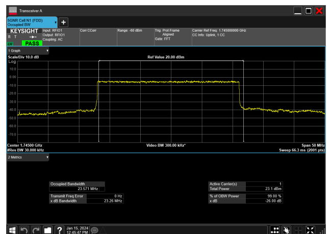
25MHz_15kHz_1745MHz_DFT-s-OFDM QPSK_RB128@0&amp;23.571 MHz
