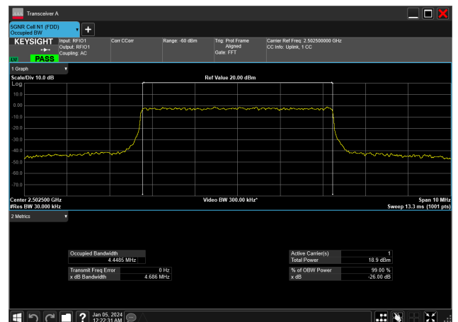
5MHz_15kHz_2502.5MHz_DFT-s-OFDM 256 QAM_RB25@0&amp;4.448 MHz
