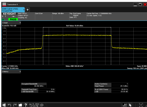
40MHz_15kHz_1730MHz_CP-OFDM 64 QAM_RB216@0&amp;38.456 MHz
