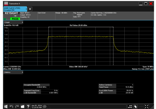
5MHz_15kHz_2502.5MHz_CP-OFDM 256 QAM_RB25@0&amp;4.464 MHz
