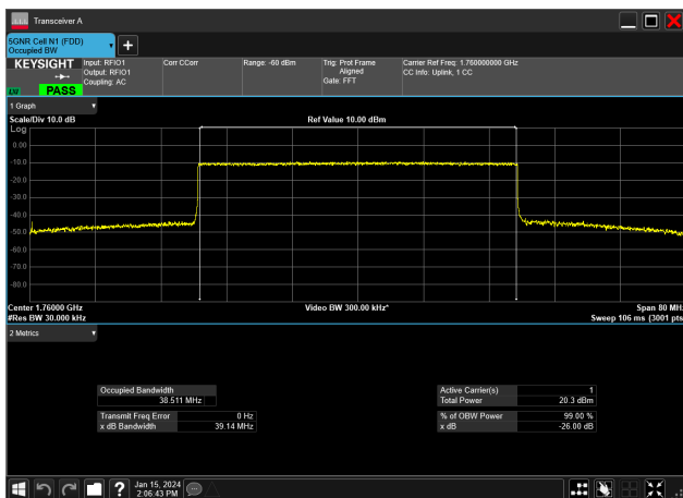
40MHz_15kHz_1760MHz_CP-OFDM 64 QAM_RB216@0&amp;38.511 MHz
