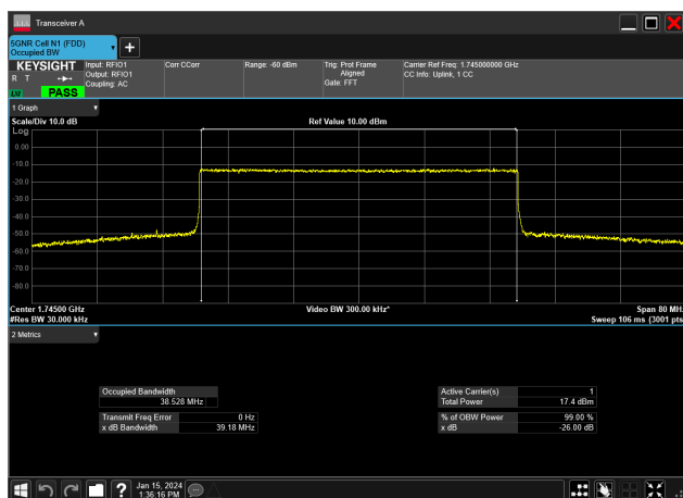
40MHz_15kHz_1745MHz_CP-OFDM 256 QAM_RB216@0&amp;38.528 MHz
