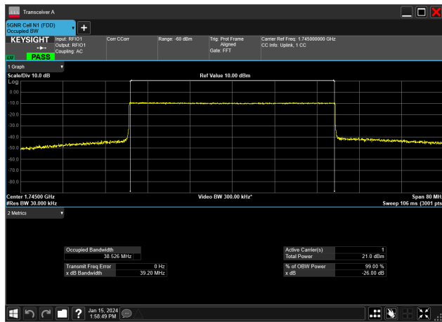
40MHz_15kHz_1745MHz_CP-OFDM QPSK_RB216@0&amp;38.526 MHz
