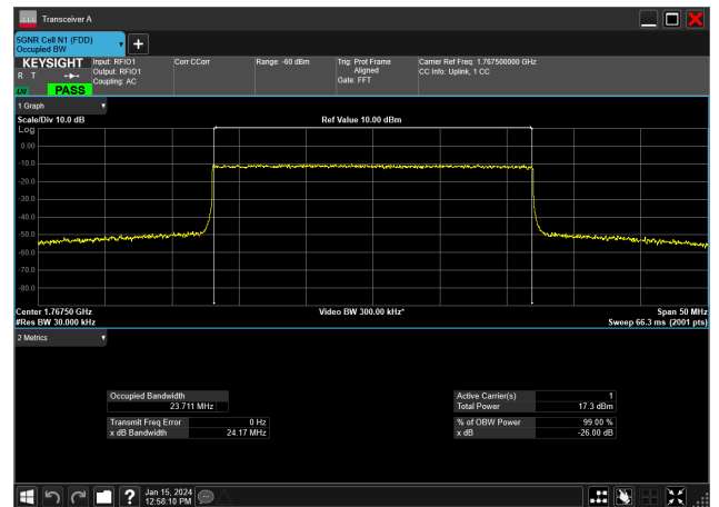
25MHz_15kHz_1767.5MHz_CP-OFDM 256 QAM_RB133@0&amp;23.711 MHz
