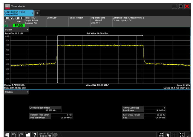
30MHz_15kHz_1745MHz_DFT-s-OFDM 256 QAM_RB160@0&amp;28.525 MHz
